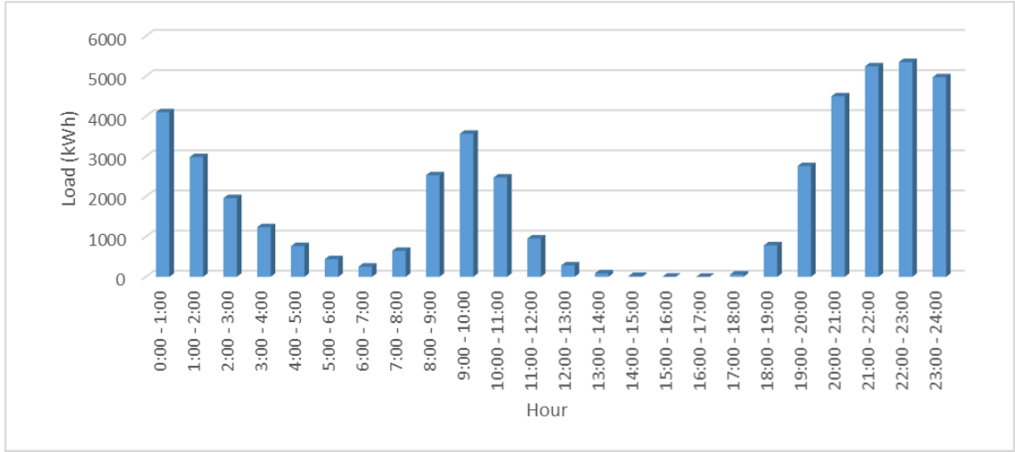
Figure 3.10 Hourly EV Power Demand in kWh with 40% Workplace Charging Availability
