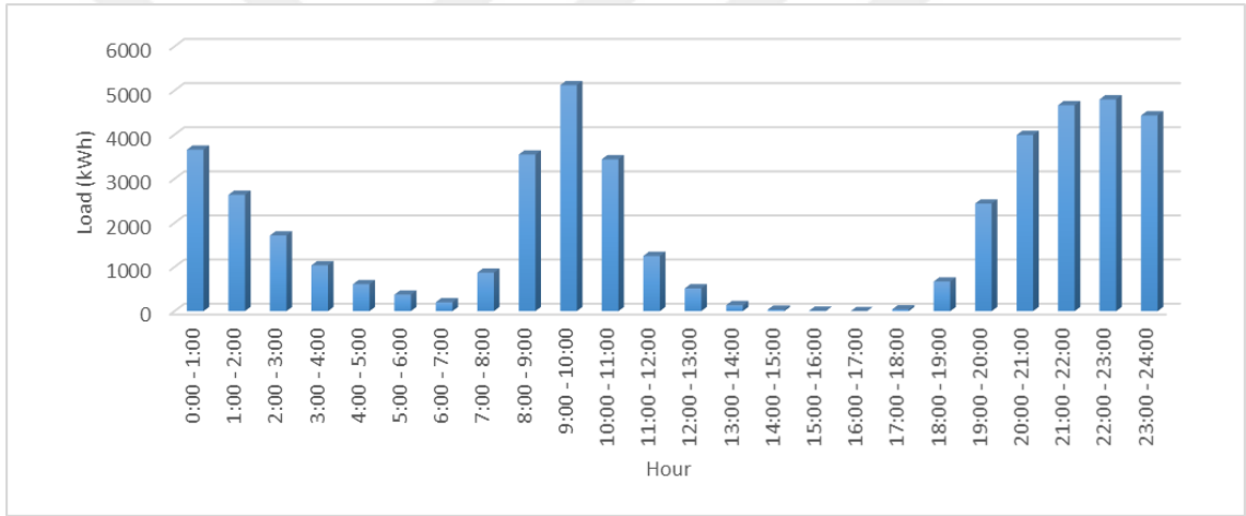
Figure 3.11 Hourly EV Power Demand in kWh with 60% Workplace Charging Availability
