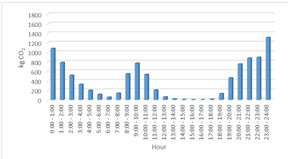
Figure 5.4 Emissions Profile for Winter 2019
