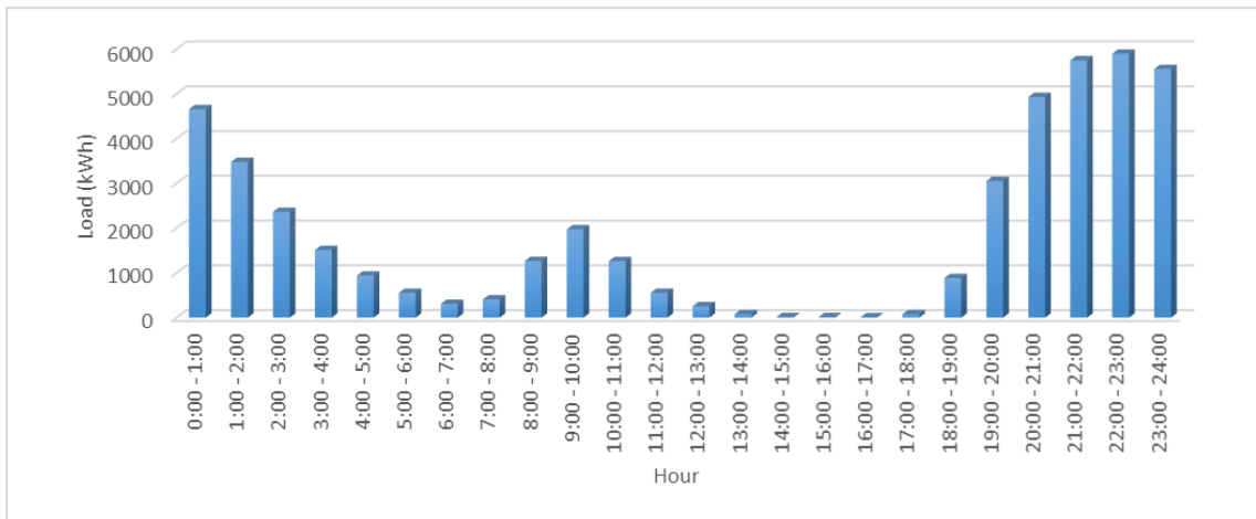
Figure 3.9 Hourly EV Power Demand in kWh with 20% Workplace Charging Availability
