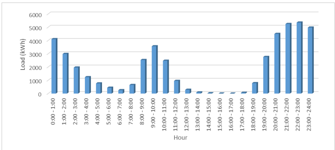
Figure 3.8 Hourly EV Power Demand in kWh
