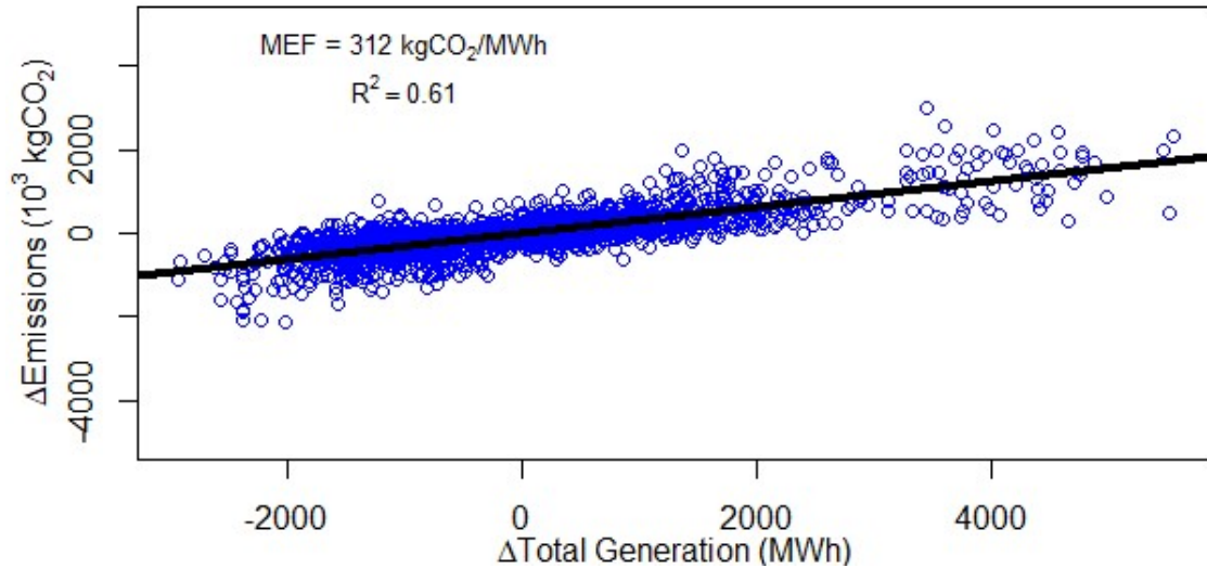
Figure 4.3 MEF for the Spring Season of 2019
