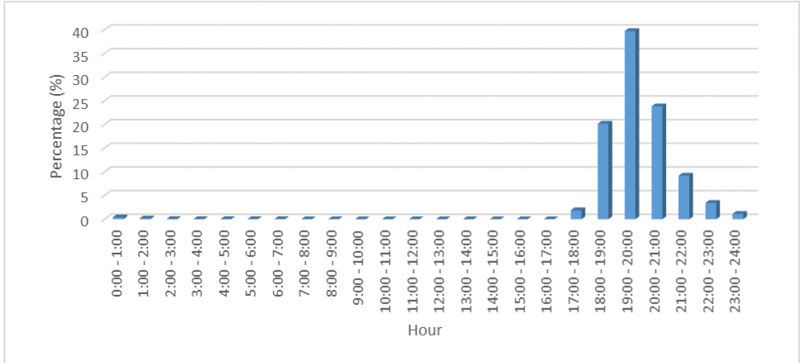
Figure 3.7 Home Charging Plug-in Time Distribution
