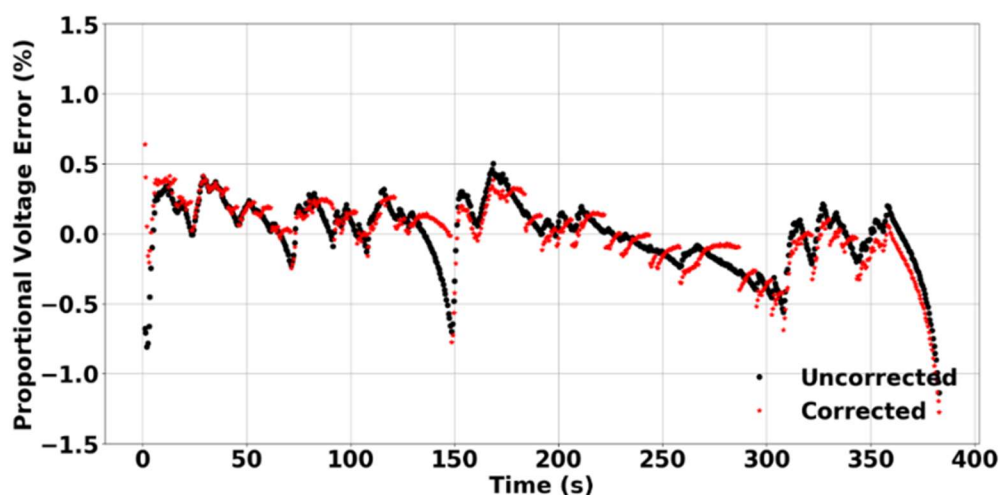
Figure 72. Calculated and measured voltage responses (Up) and percent proportional voltage error for the calculated voltage response (Bottom) after applying recovery correction for HighwayFET.
