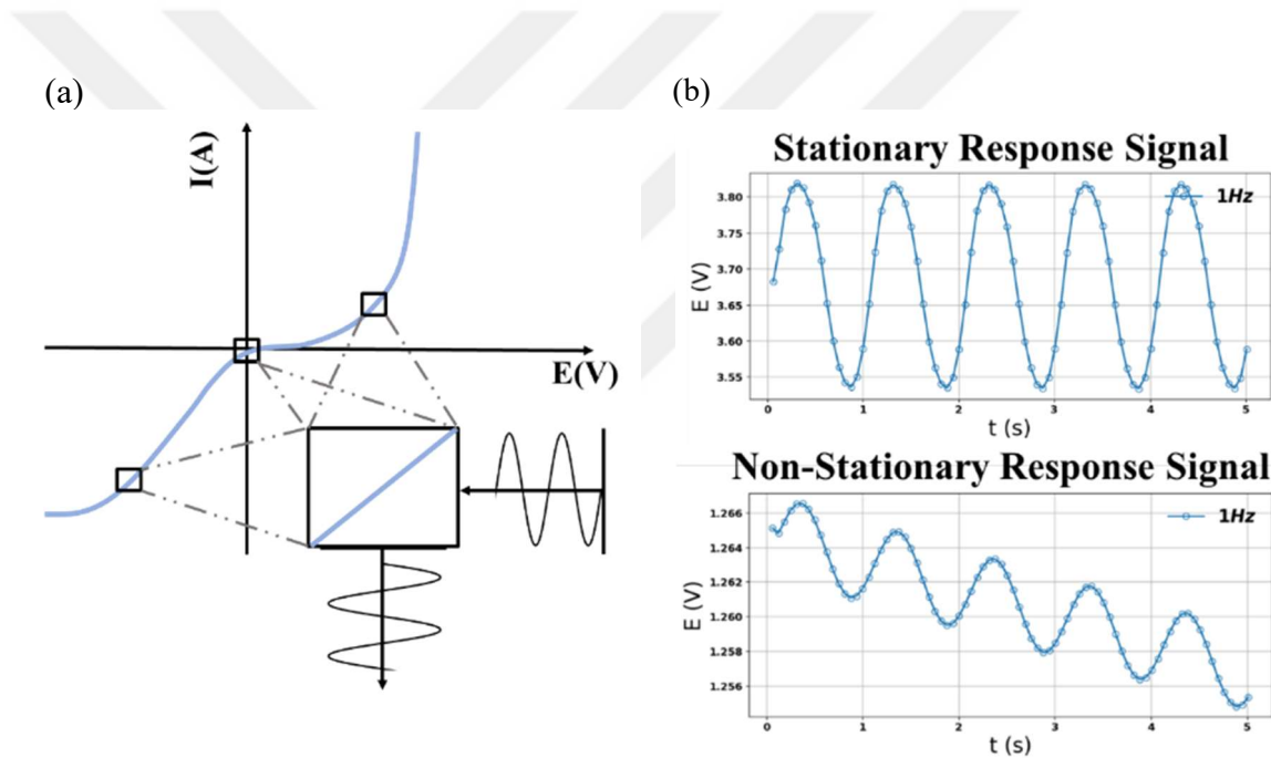
Figure 9. (a) Achieving linearity in EIS measurements by reducing the amplitude of the excitation signal, (b) Stationary vs. Nonstationary response signal in EIS measurements
