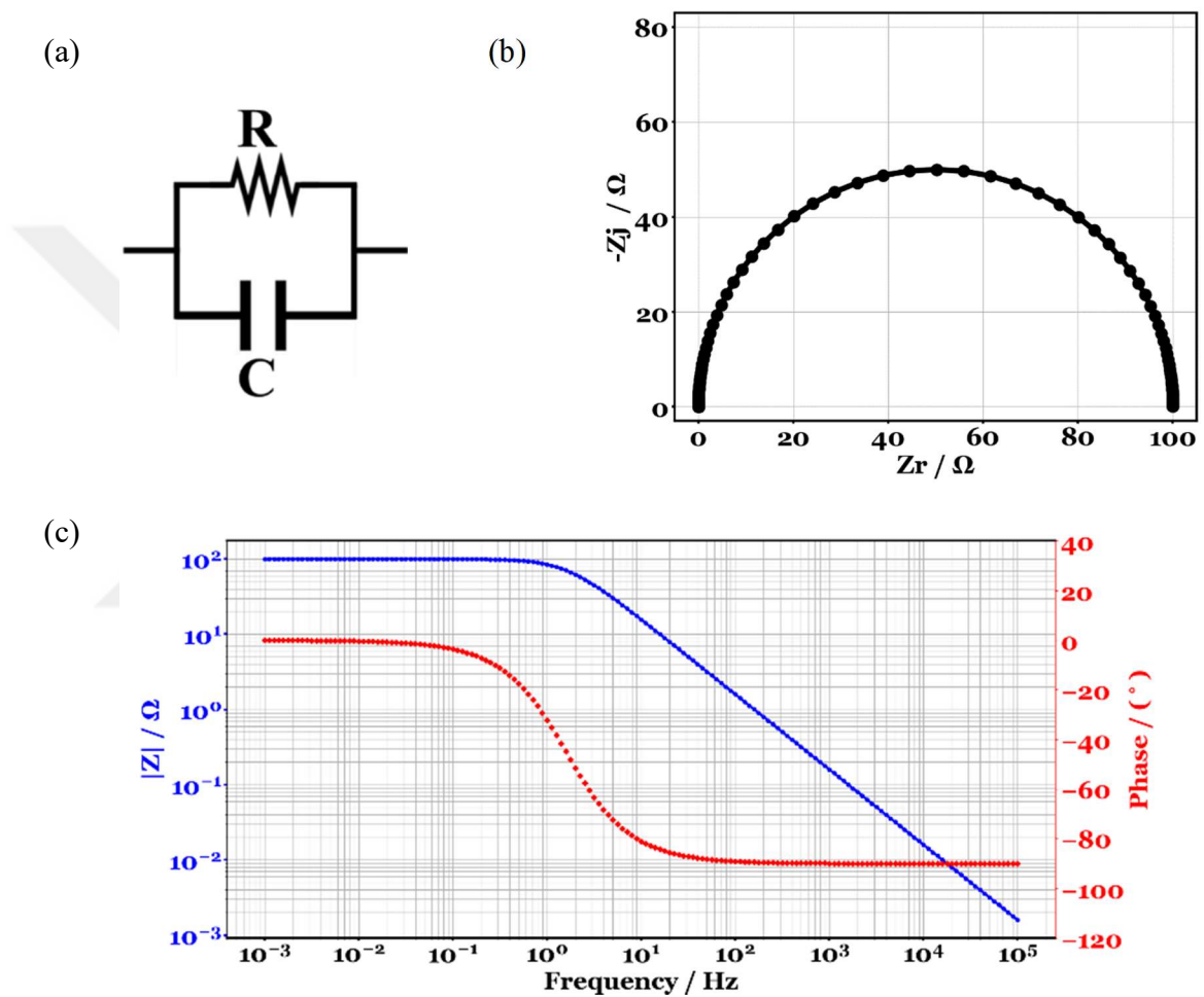
Figure 14. (a) Equivalent circuit symbol for a resistor connected in parallel to a capacitor, impedance response of RC in (b) Nyquist plot, (c) Bode plot showing the modulus impedance and the phase angle
