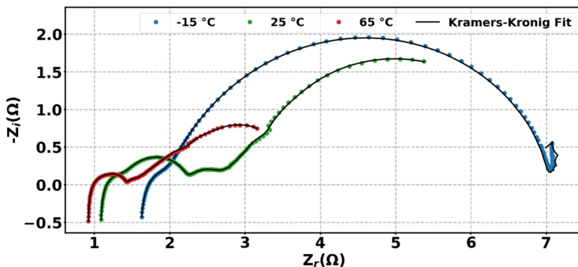
Figure 37. Temperature-dependent EIS of Li/SOCl 2 at 90% SoC with -10mA DC-offset and 2mA AC excitation at 65, 25 and -15 °C
