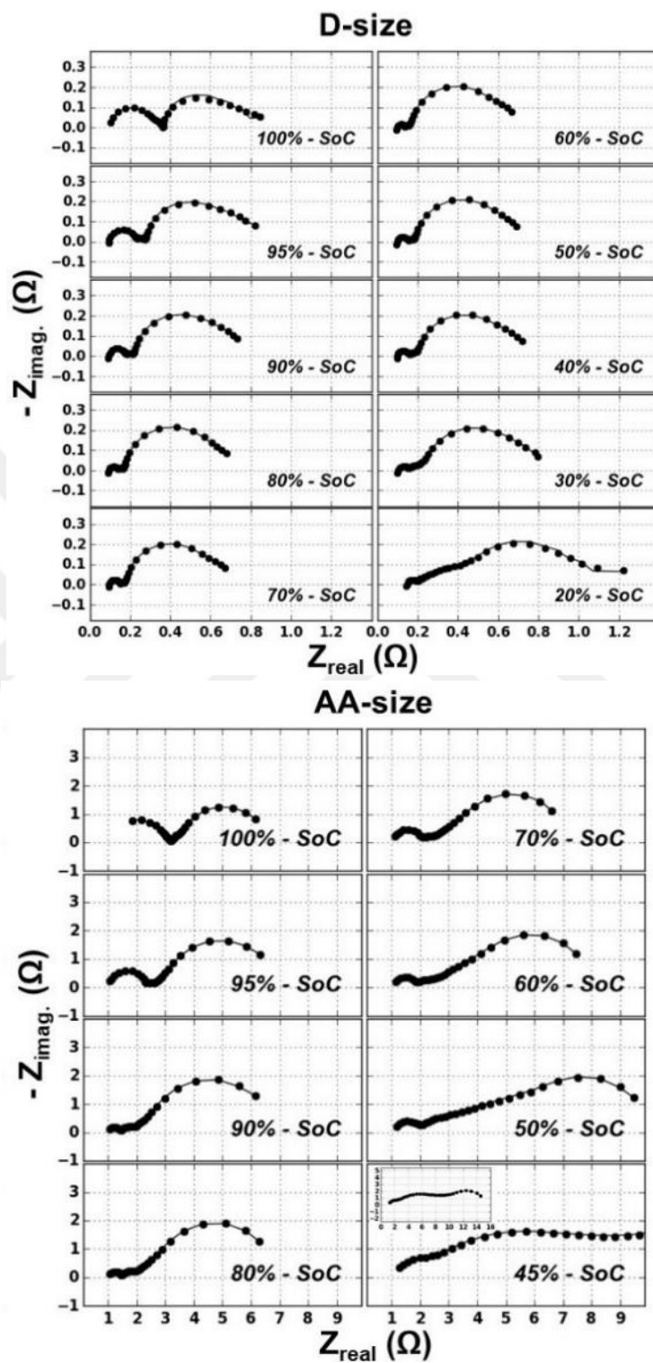
Figure 31. Nyquist diagrams for Li\SOCl 2 at different SoCs with Kramers-Kronig compatibility for D-size cell and AA-size cell
