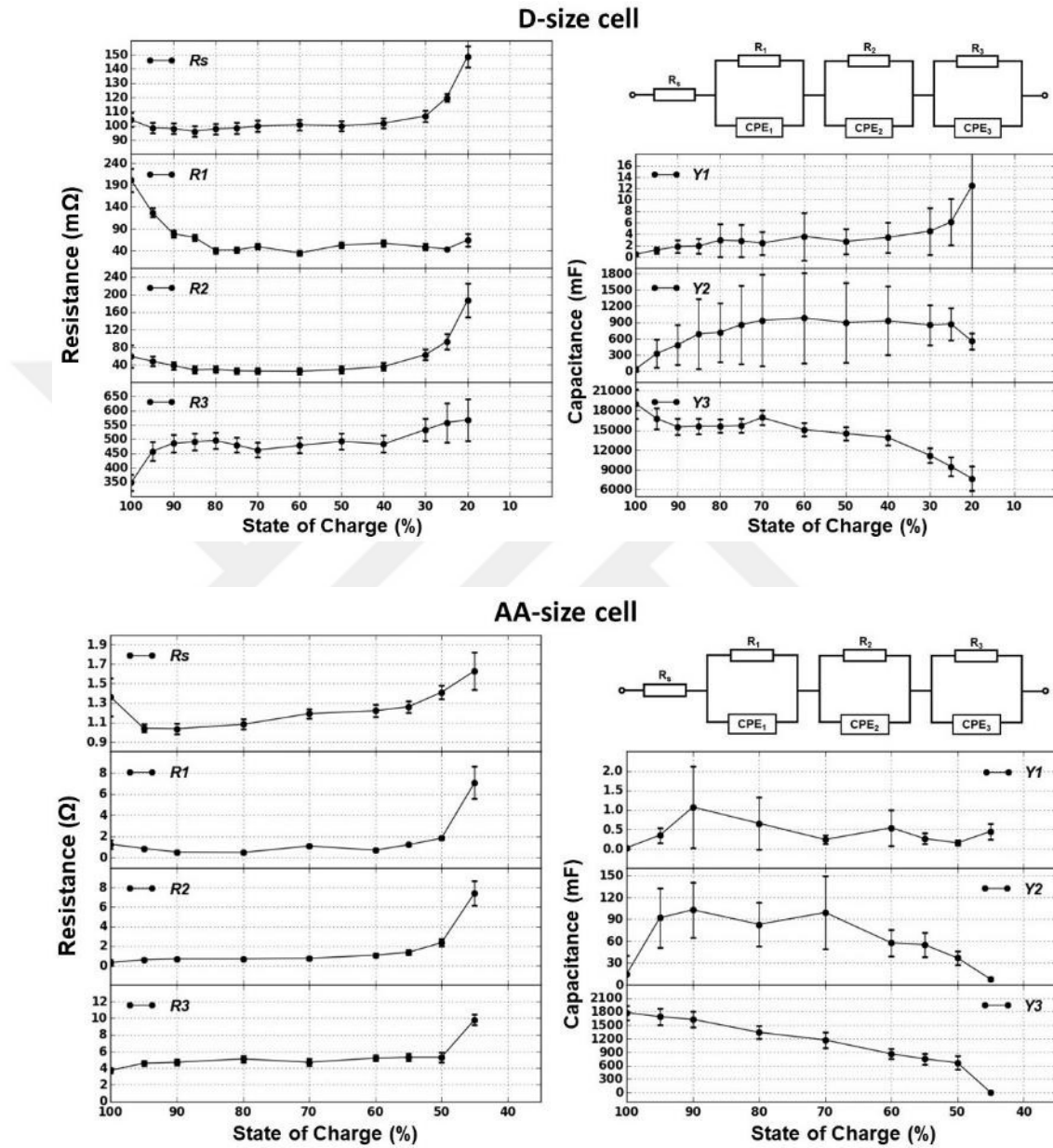
Figure 32. Equivalent circuit model and its components ( R_s , R_1 , Y_1 , R_2 , Y_2 , R_3 , Y_3 ) vs. SoC for D-size and AA-size cell
