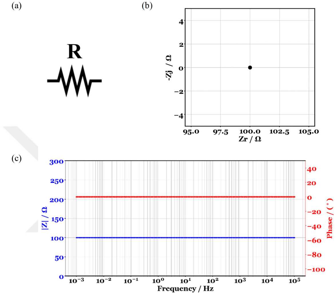
Figure 11. (a) Equivalent circuit symbol for a resistor, impedance response of R in (b) Nyquist plot, (c) Bode plot showing the modulus impedance and the phase angle
