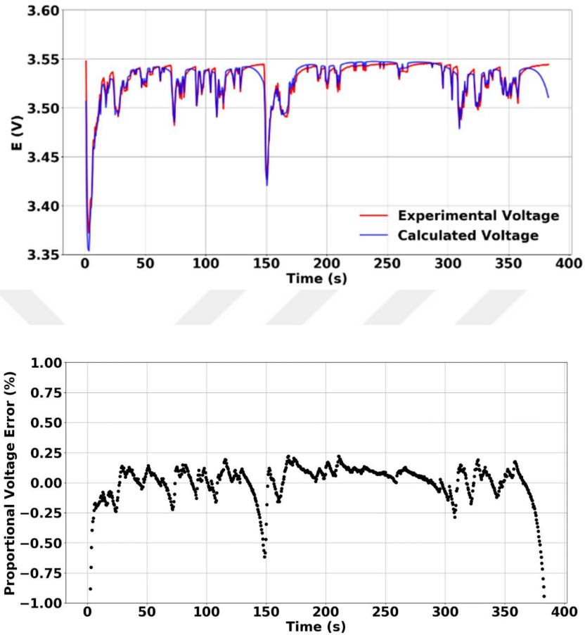
Figure 67. Calculated and measured voltage responses (Up) and percent proportional voltage error for the calculated voltage response (Bottom) of the \text{Li}\backslash\text{SOCl}_2 cell plus -50mA DC-offset for HighwayFET.
