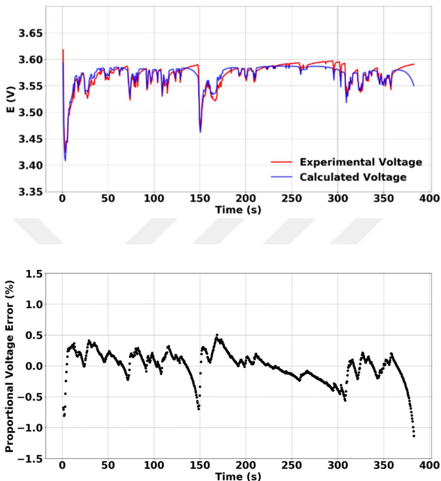
Figure 69. Calculated and measured voltage responses (Up) and percent proportional voltage error for the calculated voltage response (Bottom) of the \text{Li}\backslash\text{SOCl}_2 cell for HighwayFET.
