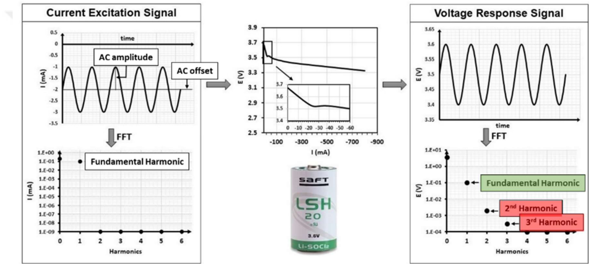
Figure 53. Galvanostatic-EIS while discharge method and harmonic analysis. Time and frequency domain of the current excitation signal (left) and voltage response signal (right).
