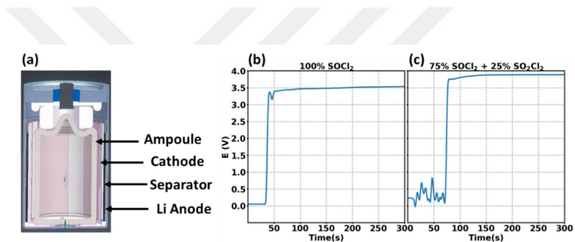
Figure 33. (a) Cross sectional view of PILTEK 10-10-01 model battery, representing ampoule, Lithium anode layer, separator and other supporting structures. Potential vs. time plots for the reserve battery during activation for (b) 100% SOCl 2 electrolyte cell and (c) 75% SOCl 2 plus 25% SO 2 Cl 2 mixture electrolyte cell.
