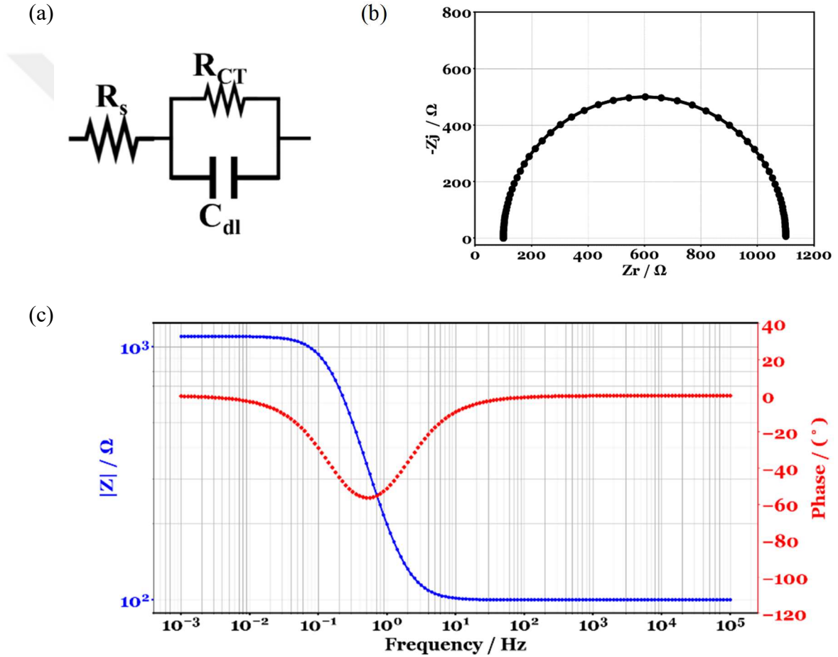
Figure 15. (a) Equivalent circuit symbol for a Randle's equivalent circuit, impedance response of R_s - R_{CT} \parallel C_{DL} in (b) Nyquist plot, (c) Bode plot showing the modulus impedance and the phase angle
