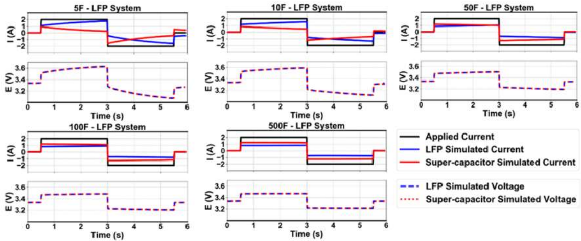
Figure 86. Simulated current distribution and the voltage response of LFP and simulated supercapacitor (5F, 10F, 50F, 100F and 500F) hybrid system under a square wave profile of 2A followed by -2A current pulses
