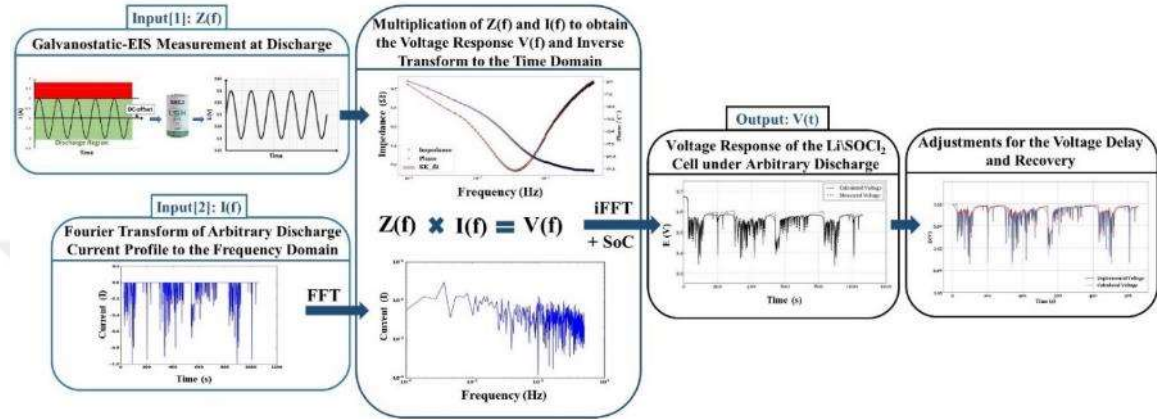
Figure 64. EIS-based modeling methodology for predicting the voltage response of Li/SOCl 2 cell at arbitrary discharge. Input(1) is the EIS measurement of the cell, Input(2) is the arbitrary discharge profile. The Output is the time domain voltage response for the applied profile.
