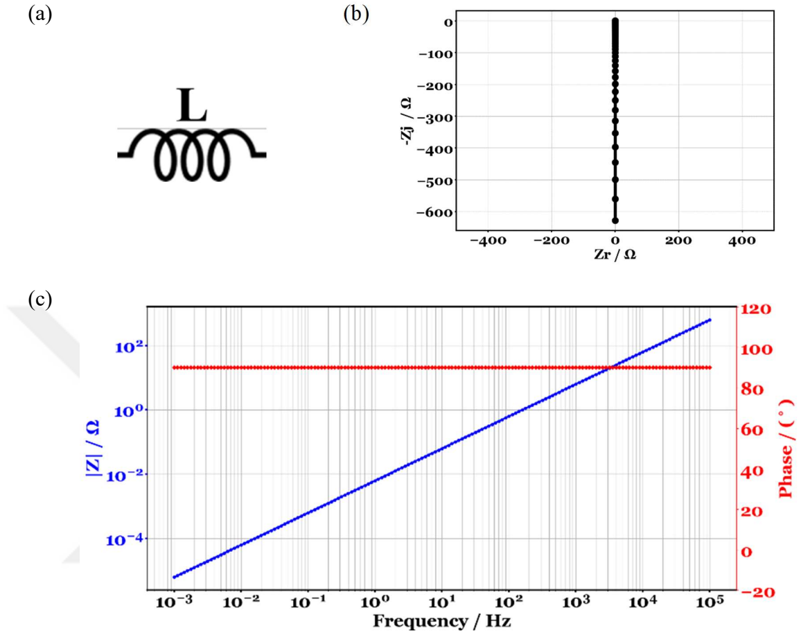
Figure 17. (a) Equivalent circuit symbol for an inductor, impedance response of L in (b) Nyquist plot, (c) Bode plot showing the modulus impedance and the phase angle
