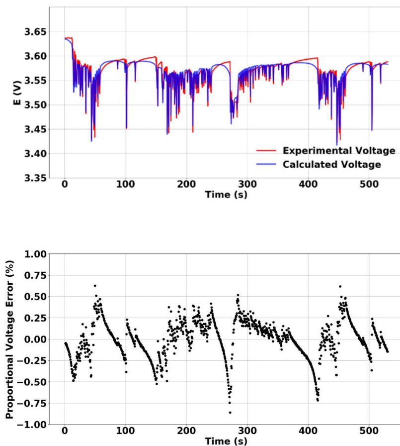
Figure 68. Calculated and measured voltage responses (Up) and percent proportional voltage error for the calculated voltage response (Bottom) of the \text{Li}\backslash\text{SOCl}_2 cell for HDUDDS.
