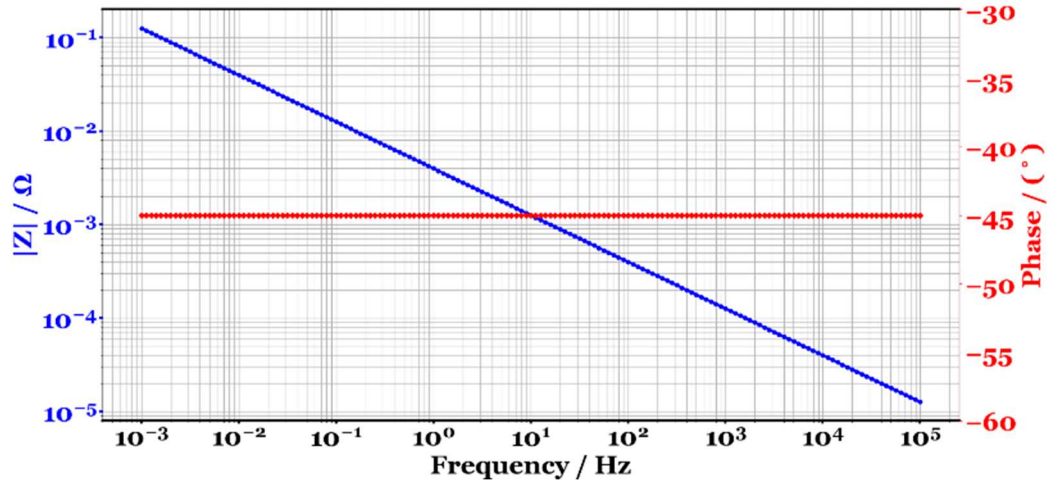
Figure 16. (a) Equivalent circuit symbol for a Warburg element, impedance response of W in (b) Nyquist plot, (c) Bode plot showing the modulus impedance and the phase angle
