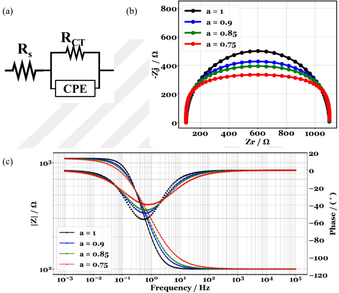
Figure 18. (a) Equivalent circuit for a Constant Phase Element, impedance response of CPE in (b) Nyquist plot, (c) Bode plot showing the modulus impedance and the phase angle with four different \alpha values (1, 0.9, 0.85, 0.75)
