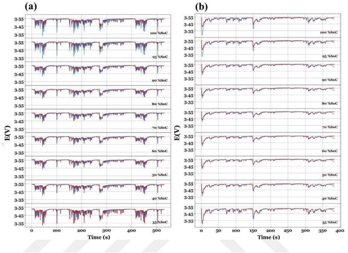
Figure 74. Calculated and experimentally measured voltage responses at different SOC for (a) HDUDDS and (b) HighwayFET
