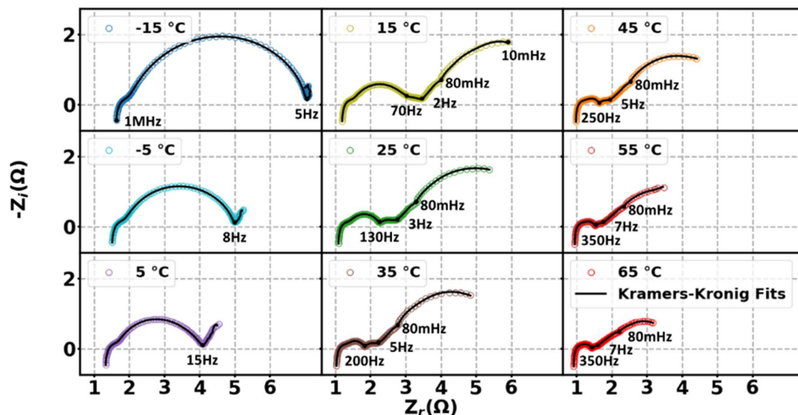
Figure 40. Nyquist plots of the Temperature-dependent EIS for \text{Li}\backslash\text{SOCl}_2 at 90% State-of-Charge
