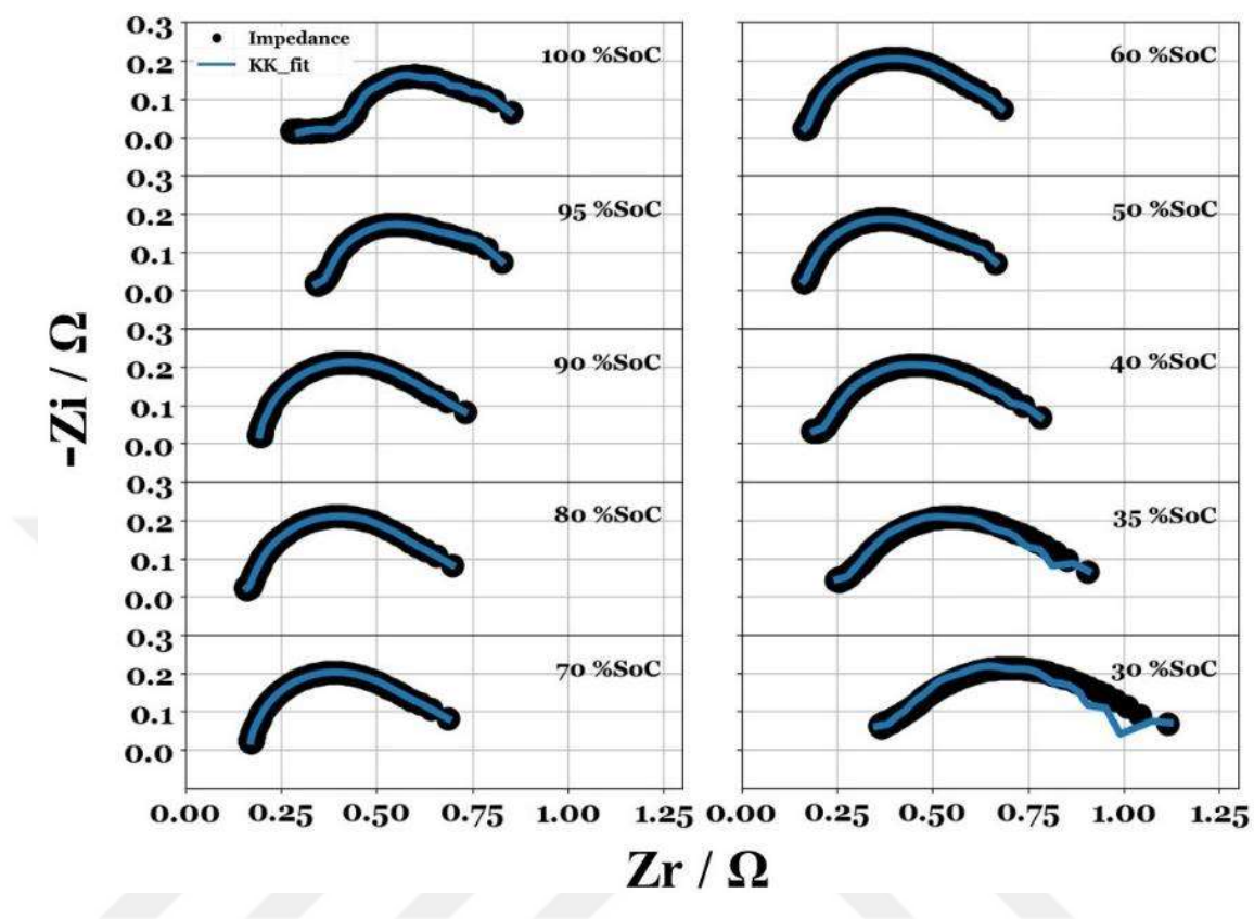
Figure 73. Nyquist plots for the EIS of \text{Li}\backslash\text{SOC}\backslash\text{l}_2 battery from 100% to 30% states of charge
