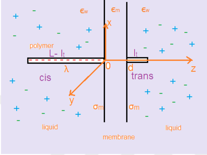
Figure 5.2: Schematic depiction of a polymer with length L translocating through a membrane of thickness d from the CIS to the TRANS side.
