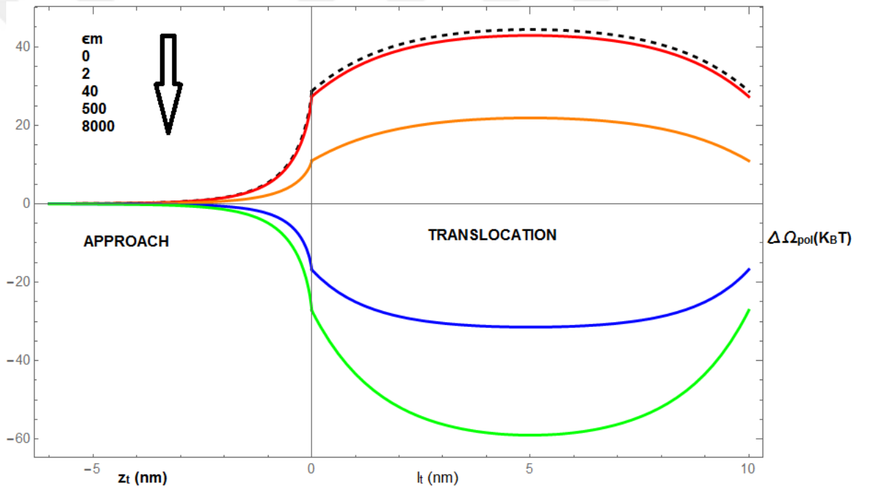
Figure 5.3: Polymer grand potential in the approach and translocation phases through a neutral membrane ( \sigma_m = 0 ) for different \epsilon_m 's. The polymer length is L = 10 nm, the membrane thickness is d = 2 nm, and the solution concentration is n_b = 0.01 M. The black dashed curve corresponds to the limit \epsilon_m = 0 .
