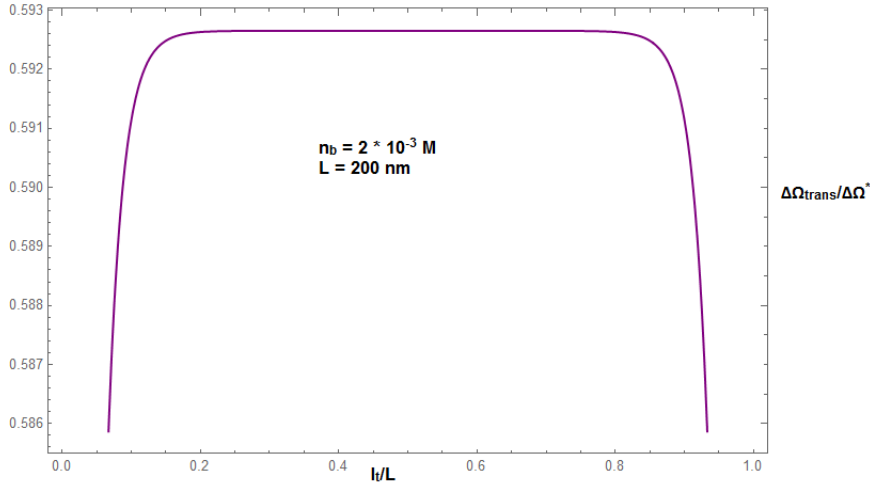
Figure 5.7: Polymer translocation energy rescaled by the characteristic energy \Delta\Omega^* = k_B T l_B \lambda^2 / \kappa versus the translocated length rescaled by the polymer length l_t/L . For very long polymers (e.g L = 200 nm), the potential curve becomes steep on the sides and the potential has a stable maximum for most of the range 0 < l_t < L , instead of a metastable point, making the potential curve look like a potential step rather than a convex curve.
