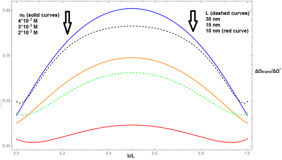
Figure 5.6: Polymer translocation energy rescaled by the characteristic energy \Delta\Omega^* = k_B T l_B \lambda^2 / \kappa versus the translocated length rescaled by the polymer length l_t/L . The solution concentration is n_b = 2 \times 10^{-3} M (red curve), n_b = 3 \times 10^{-3} M (orange curve), and n_b = 4 \times 10^{-3} M (blue curve). The polymer length is L = 10 nm (red curve), L = 15 nm (green curve), and L = 30 nm (black curve).
