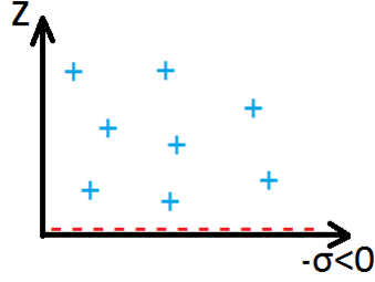
Figure 3.1: Schematic depiction of the counter-ion-only liquid in contact with a negatively charged membrane surface.
