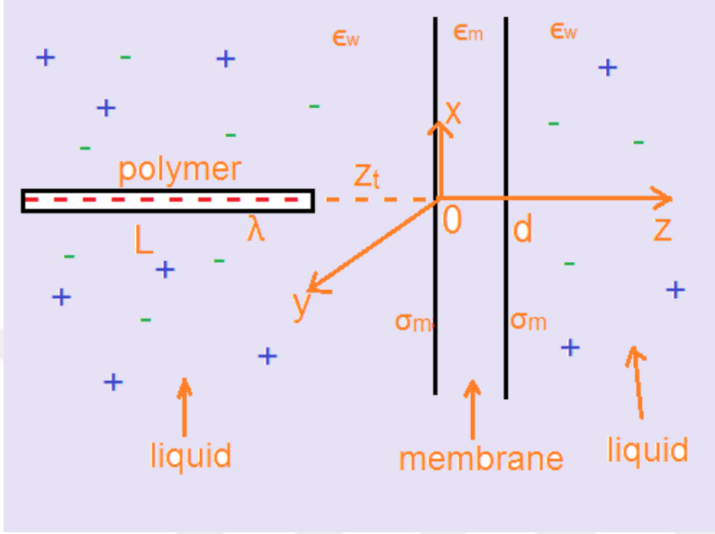
Figure 5.1: Schematic representation of a polymer with length L approaching a membrane of thickness d from the CIS side at a distance z_t ( L \gg d ).
