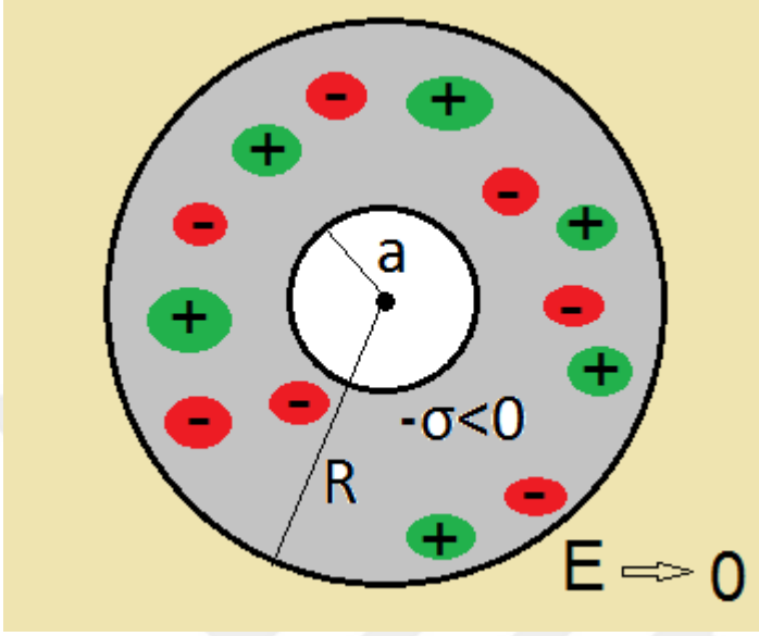
Figure 3.2: Accumulation of charges around a rod-like object of radius a and surface charge density -\sigma < 0 confined to a pore of radius R .
