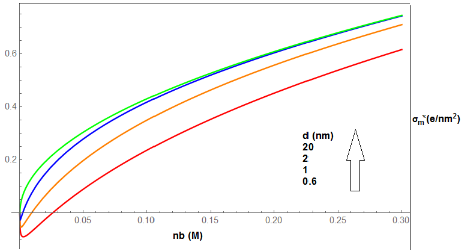
Figure 5.9: The critical membrane surface charge density versus the solution concentration for different membrane thickness values.
