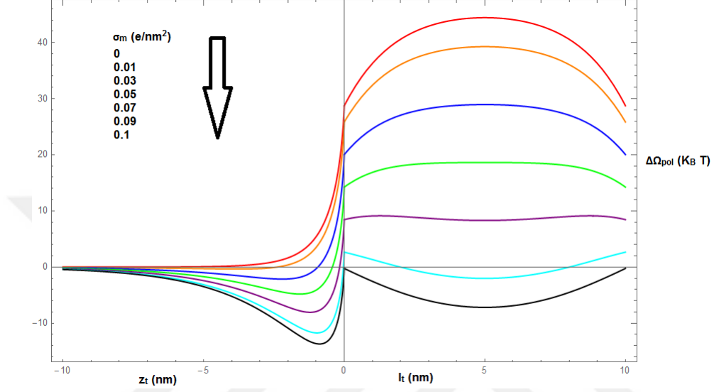
Figure 5.8: Polymer grand potential in the approach and translocation phases for different membrane surface charge densities. The membrane permittivity \epsilon_m is set to zero, and the salt concentration is n_b = 0.01 M.
