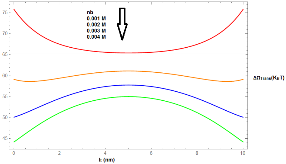
Figure 5.5: Polymer translocation energy for salt concentrations n_b = 0.001, 0.002, 0.003, 0.004 M. The figure shows how the translocation energy profile turns from concave to convex at the characteristic concentration n_b \simeq 0.002 M.
