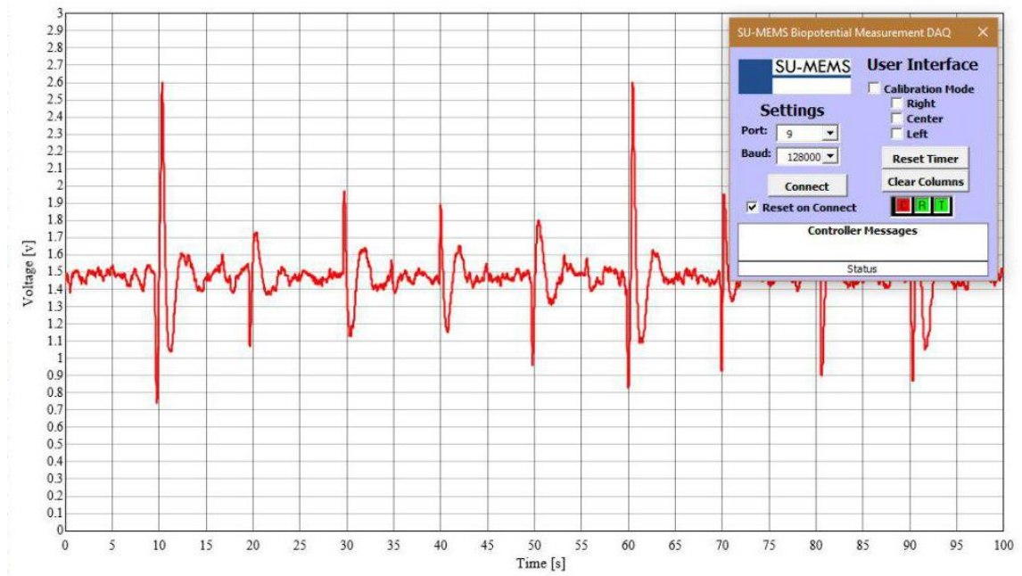
Figure 3.7. EOG signal after smoothing in the \mu CU which is displayed in real-time through the preliminary Microsoft Excel-based GUI.
