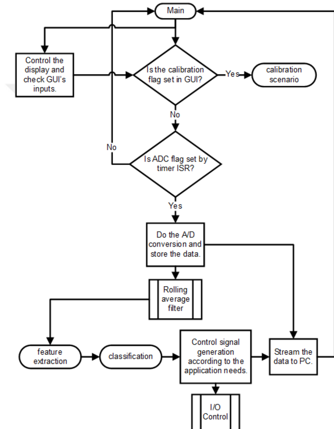
Figure 4.1. Summarized flowchart of the developed algorithm for automatic detection of blink along with four different saccadic EMs in single-channel forehead EOG.
