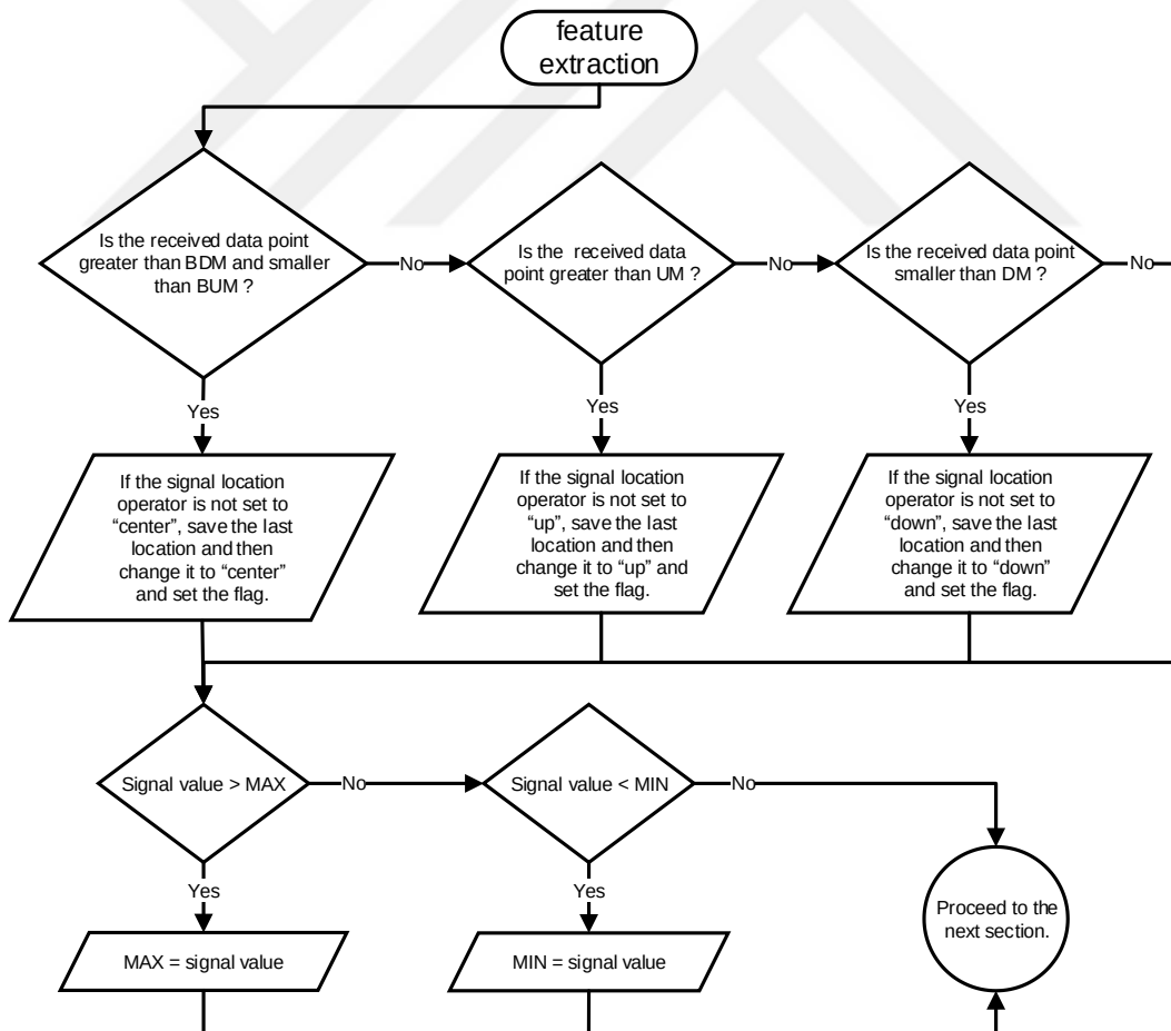
Figure S2. The detailed feature extraction section of the flowchart for the proposed automatic EM detection algorithm.
