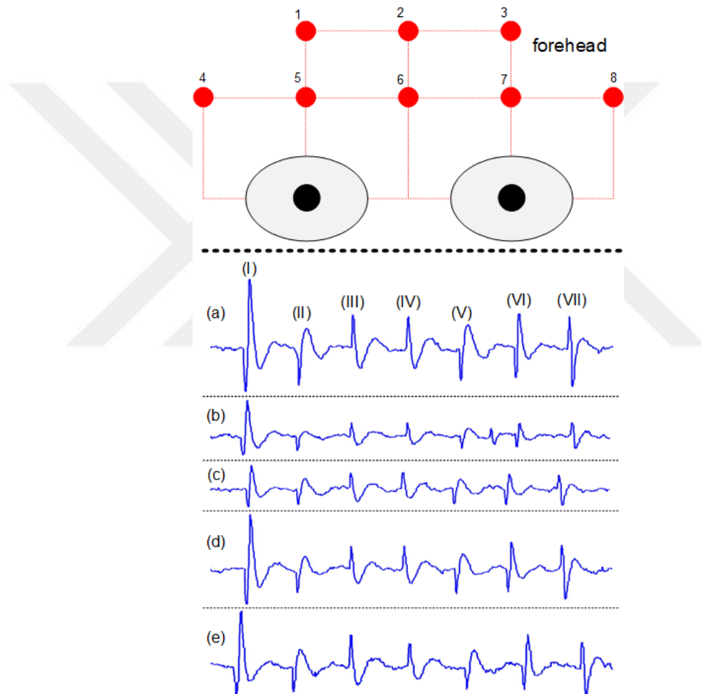
Figure 3.5. Systematic analysis of electrode positioning in forehead EOG. The fabricated electrodes were cut into \sim 3 \times 3 cm dimension to test different placement configurations. Waveforms show the induced electrooculograms from (a) locations 4, 6, 8; (b) locations 5, 6, 7; (c) locations 1, 2, 3; (d) locations 5, 6, 8; (e) locations 4, 6, 7; where the first, second, and third digit corresponds to the location of the left, reference, and the right lead, respectively. The performed EMs were: (I) voluntary blink, (II) slow left, (III) slow right, (IV) swift left, and (V) swift right.
