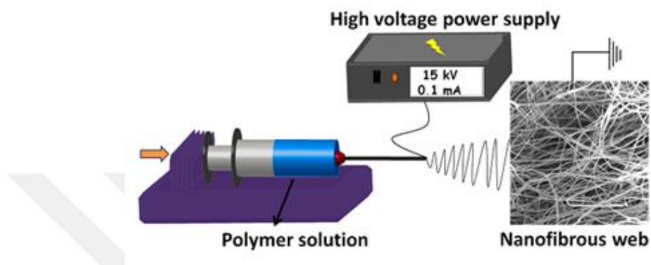
Figure 2: Schematic representation of the electrospinning set-up.
