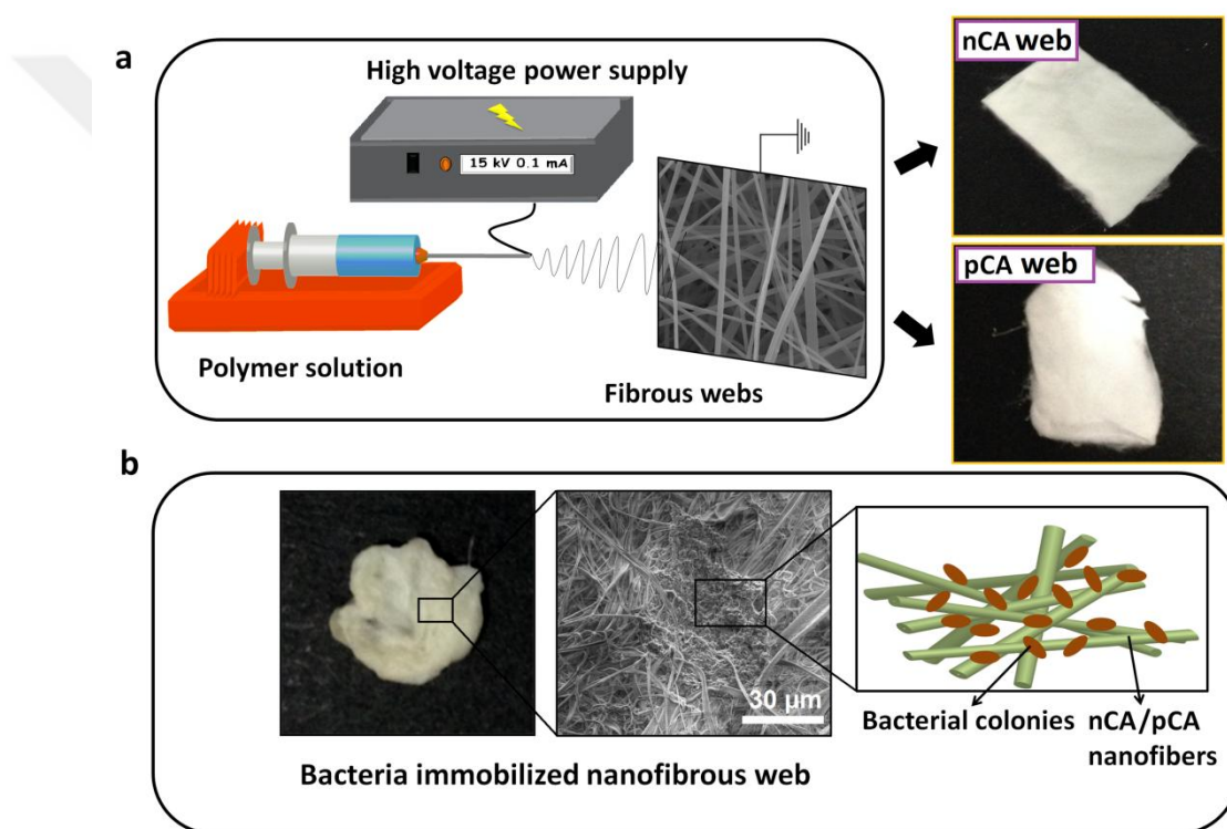
Figure 19: (a) Schematic representation of electrospinning process for nCA and pCA webs, and photographs of nCA and pCA webs, (b) representative images for bacteria immobilized webs including a SEM micrograph and schematic representation of bacterial cells on fibrous surfaces. (Copyright © 2013, Reproduced from Ref. [19] with permission from the Royal Society of Chemistry)
