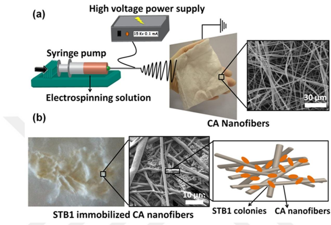
Figure 4: (a) Schematic representation of electrospinning process for CA nanofibers and photograph of CA nanofibrous web (b) photograph of STB1 immobilized CA nanofibrous web and schematic representation of bacterial cells on nanofiber surfaces. (Copyright © 2013, Reproduced from Ref. [18] with permission from the Royal Society of Chemistry)
