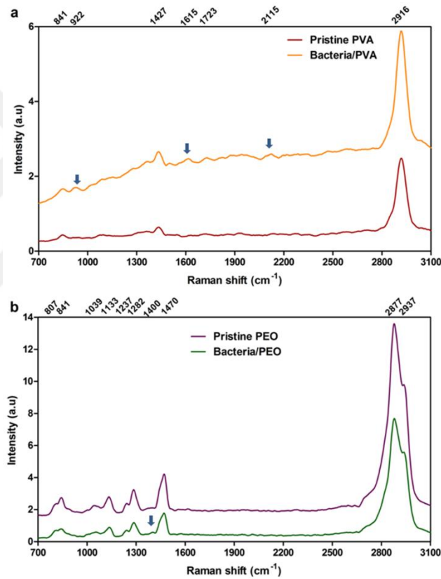
Figure 43: Raman spectra of (a) pristine PVA and bacteria/PVA and (b) pristine PEO and bacteria/PEO webs.
