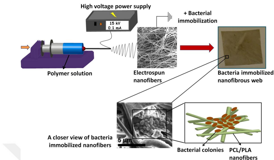
Figure 35: Schematic representation of the electrospinning process and representative images for bacterial immobilization including a photograph of bacteria immobilized electrospun nanofibrous web, a SEM micrograph of bacteria immobilized nanofibers and a schematic representation of the immobilized cells on electrospun nanofibers.
