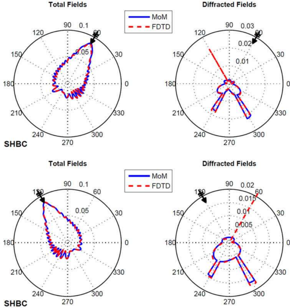
Figure 4.5 Total (Left) and diffracted (right) fields around the SHBC strip: (Top), \phi_0 = 60^\circ , (Bottom), \phi_0 = 120^\circ , ( f = 30\text{MHz} , L = \lambda , \rho_0 = 8\lambda , \rho = 7\lambda Solid: MoM, Dashed: FDTD).
