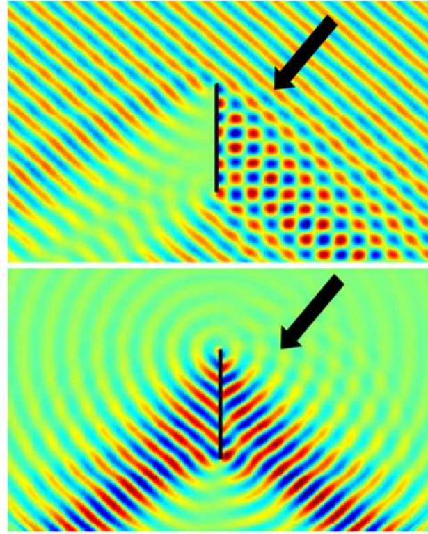
Figure 4.3 FDTD-generated (Top) total and (Bottom) scattered fields around the SHBC strip.
