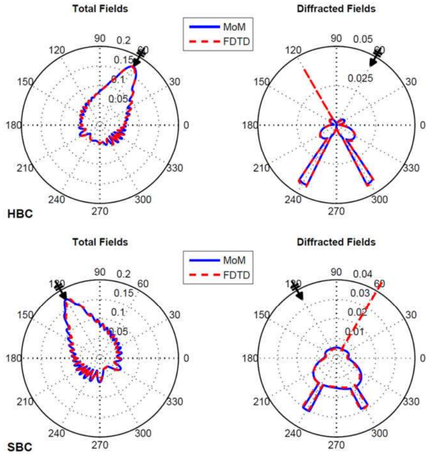
Figure 4.4 Total (Left) and diffracted (right) fields around the strip: (Top) HBC, \varphi_0 = 60^\circ , (Bottom) SBC, \varphi = 120^\circ ( f = 30\text{MHz} , L = \lambda , \rho_0 = 8\lambda , \rho = 7\lambda Solid: MoM, Dashed: FDTD).
