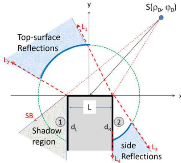
Figure 3.3 Double tip structure (Structure-1)
