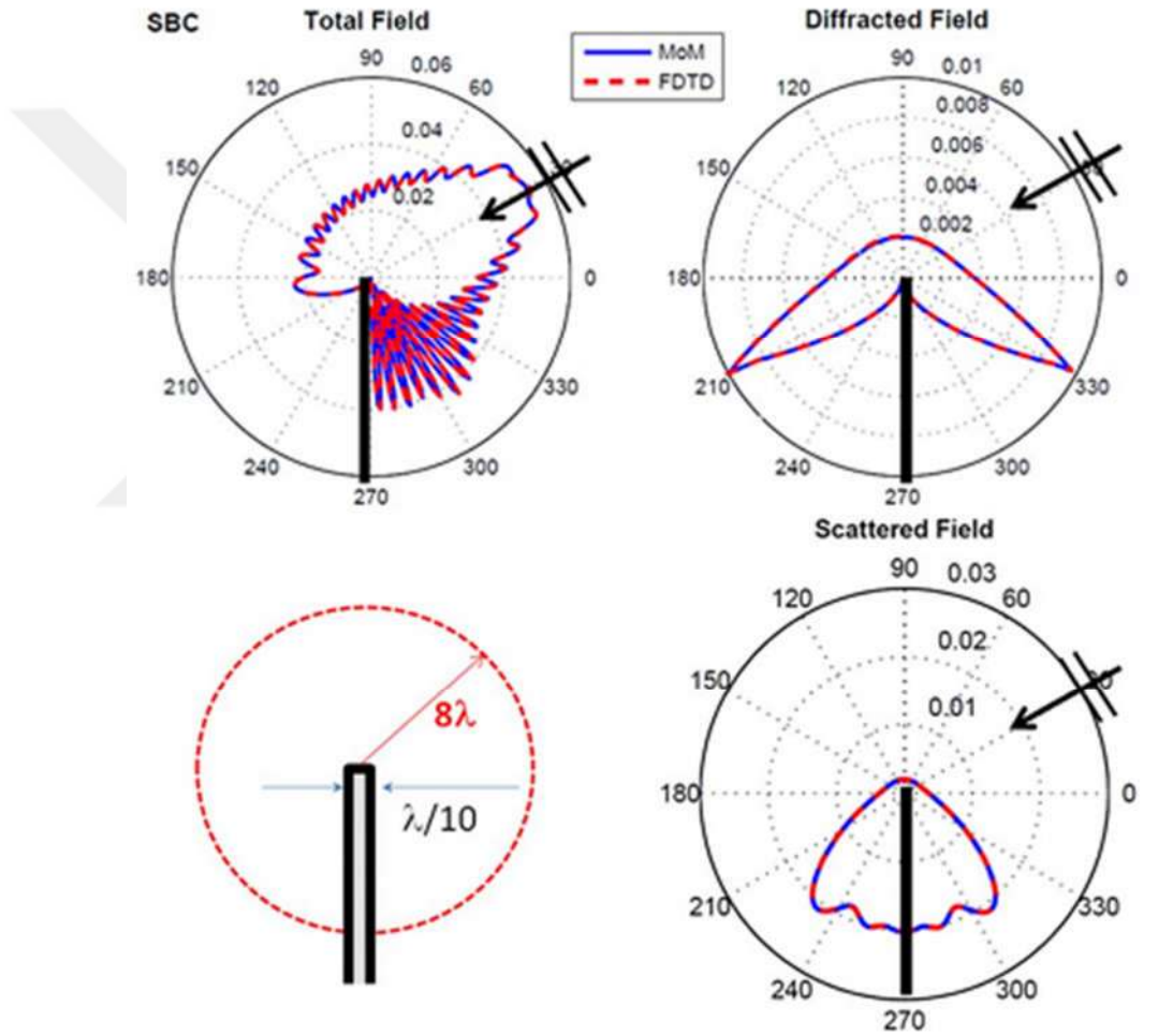
Figure 3.6 Total, diffracted, and scattered fields around Structure-1; L = \lambda/10 , \rho_0 = 10\lambda , \phi_0 = 30^\circ ,
