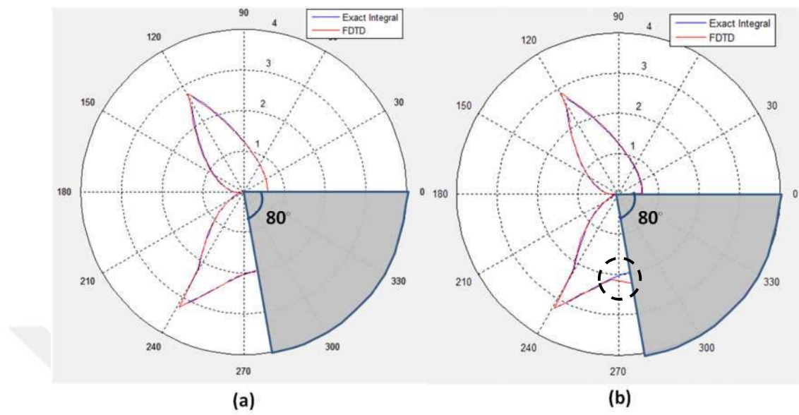
Figure 2.21 Comparison of Dey-Mitra (a) and staircase (b) modeling in wedge diffraction problem
