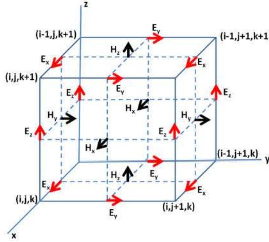
Figure 2.12 Yee Cell
