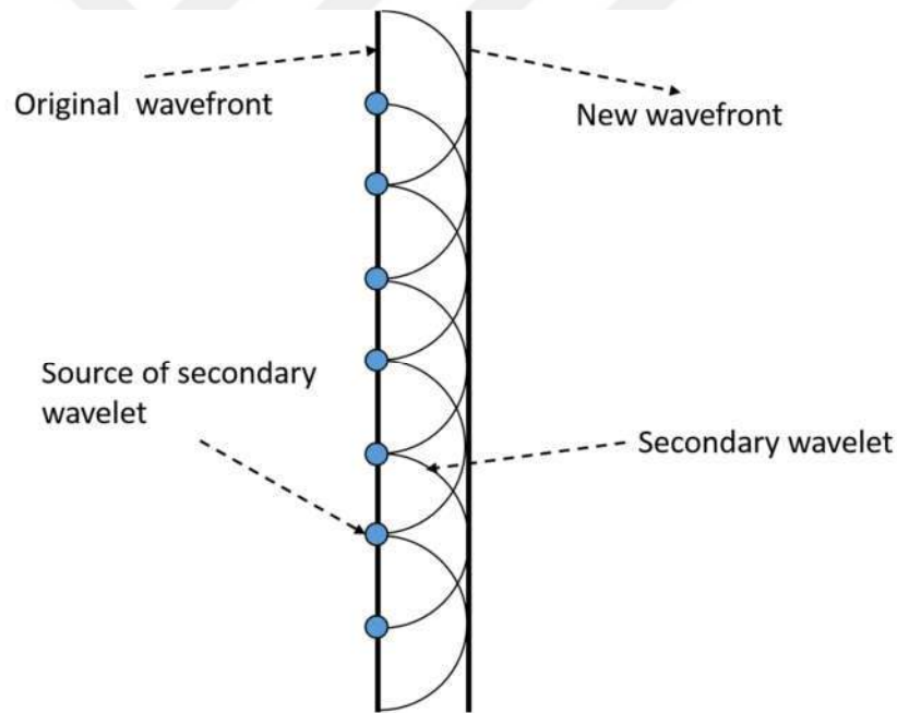
Figure 3.1 Huygen's Principle
