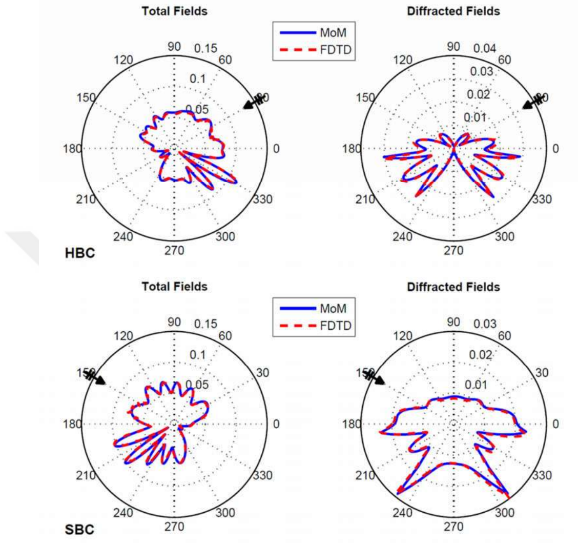
Figure 4.6 Total (Left) and diffracted (right) fields around the strip: (Top) HBC, \varphi_0 = 30^\circ , (Bottom) SBC, \varphi_0 = 150^\circ , ( f = 30\text{MHz} , L = 2\lambda , \rho_0 = 10\lambda , \rho = 3\lambda Solid: MoM, Dashed: FDTD).
