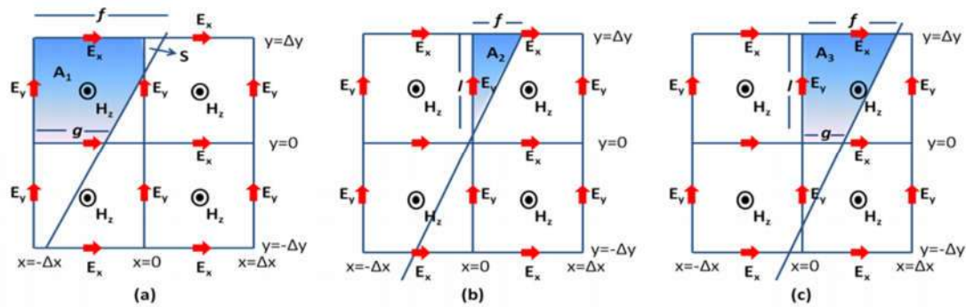
Figure 2.20 Three different scenarios for conformal modeling [37]
