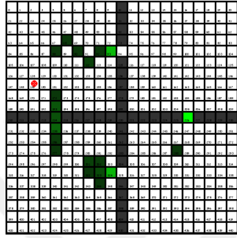
(c) SDD result on STEPPOSITIVE
