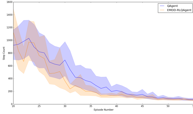
Figure 5.7: The total number of steps that the agents have taken to reach the goal state per episode is shown. The average step value is obtained from 40 experiments. The shaded areas represent the 95% bootstrap confidence interval.
