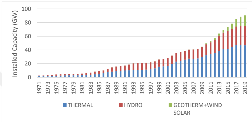
Figure 4-1. Change in Turkey's Installed Capacity from 1971 (Source: TEİAŞ)
