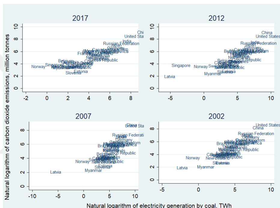
Figure 5-1. Scatterplot of \ln\text{CO}_2 and Natural Logarithm of Electricity Generation by Coal
