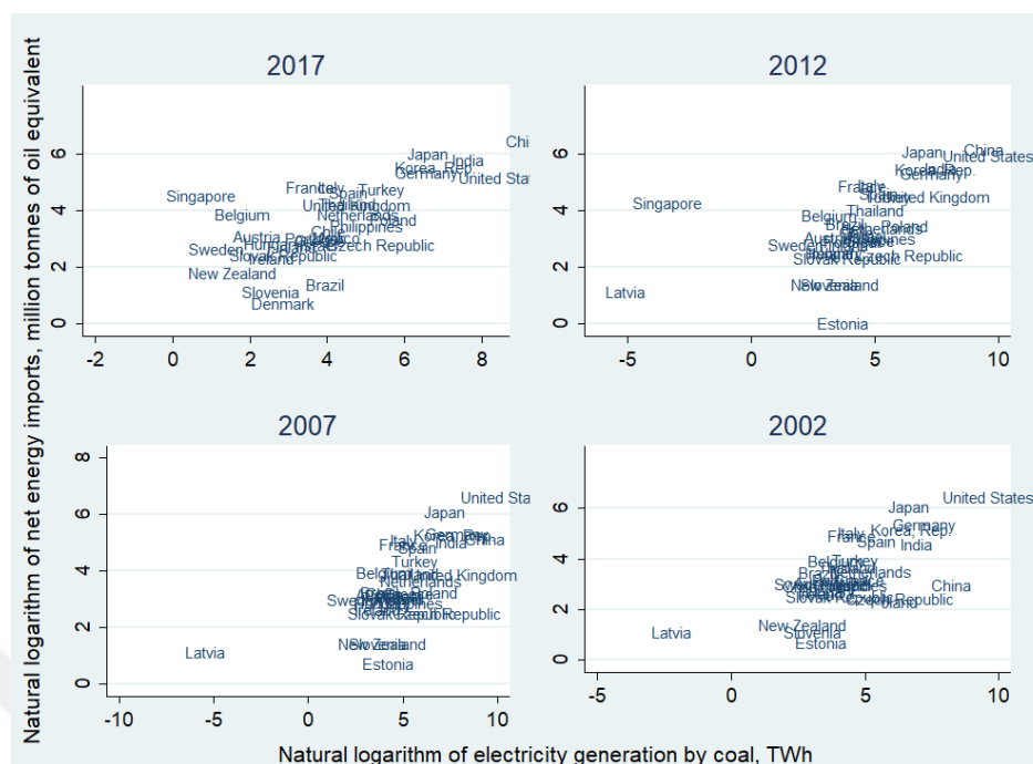
Figure 5-4. Scatterplot of lnEI and Natural Logarithm of Electricity Generation by Coal
