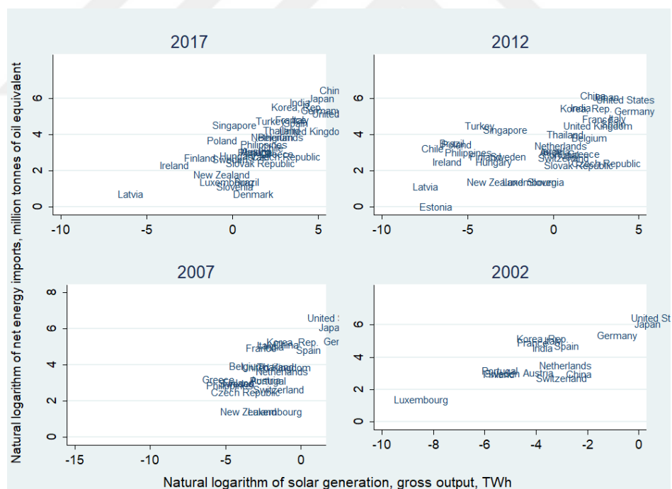
Figure 5-5. Scatterplot of lnEI and Natural Logarithm of Solar Electricity Generation
