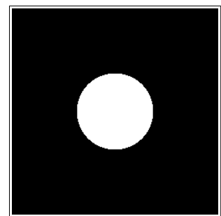
Binary ( T = 160 )
