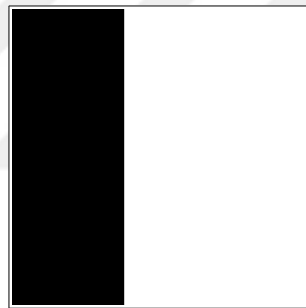
Binary ( T = 96 )
