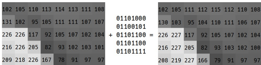
Figure 2.24 LSB Steganography
