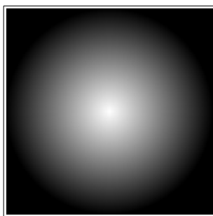
Grayscale
