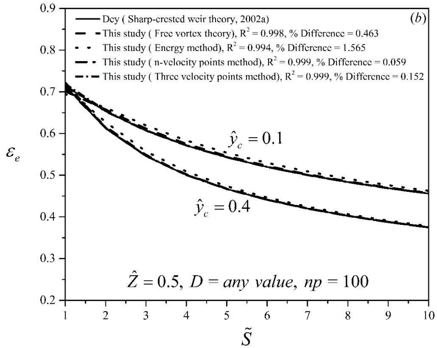
Figure 5.22: Comparison between \varepsilon_e versus \tilde{S} values based on the proposed four methods and (a) Dey (2002) by the Boussinesq approach; (b) Dey (2002) by the sharp-crested weir approach of the circular channel cross-section for \hat{Z} = 0.5 , D = \text{any value} , and 0.1 \leq \hat{y}_c \leq 0.4
