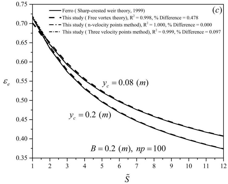
Figure 5.1: Comparison between the variation of \varepsilon_e on \tilde{S} for 0.08 \text{ (m)} \leq y_c \leq 0.2 \text{ (m)} and B = 0.2 \text{ (m)} of the two suggested theoretical approaches and the theoretical solution of the free vortex theory with the study of (a) Anderson (1967); (b) Murty Bhallamudi (1994); and (c) Ferro (1999) in rectangular channel cross-sections
