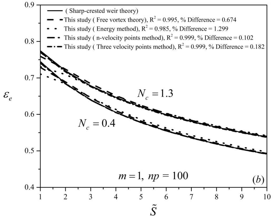
Figure 5.12: Comparison between the \varepsilon_e values obtained based on four theoretical methods and the \varepsilon_e values of the (a) Boussinesq approach by Murty Bhallamudi (1994); and (b) sharp-crested weir theory for the trapezoidal channel cross-sections at supercritical regimes
