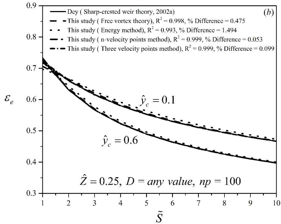
Figure 5.21: Comparison between \varepsilon_e versus \tilde{S} values based on the proposed four methods and (a) Dey (2002) by the Boussinesq approach; (b) Dey (2002) by the sharp-crested weir approach of the circular channel cross-section for \hat{Z} = 0.25 , D = \text{any value} , and 0.1 \leq \hat{y}_c \leq 0.6
