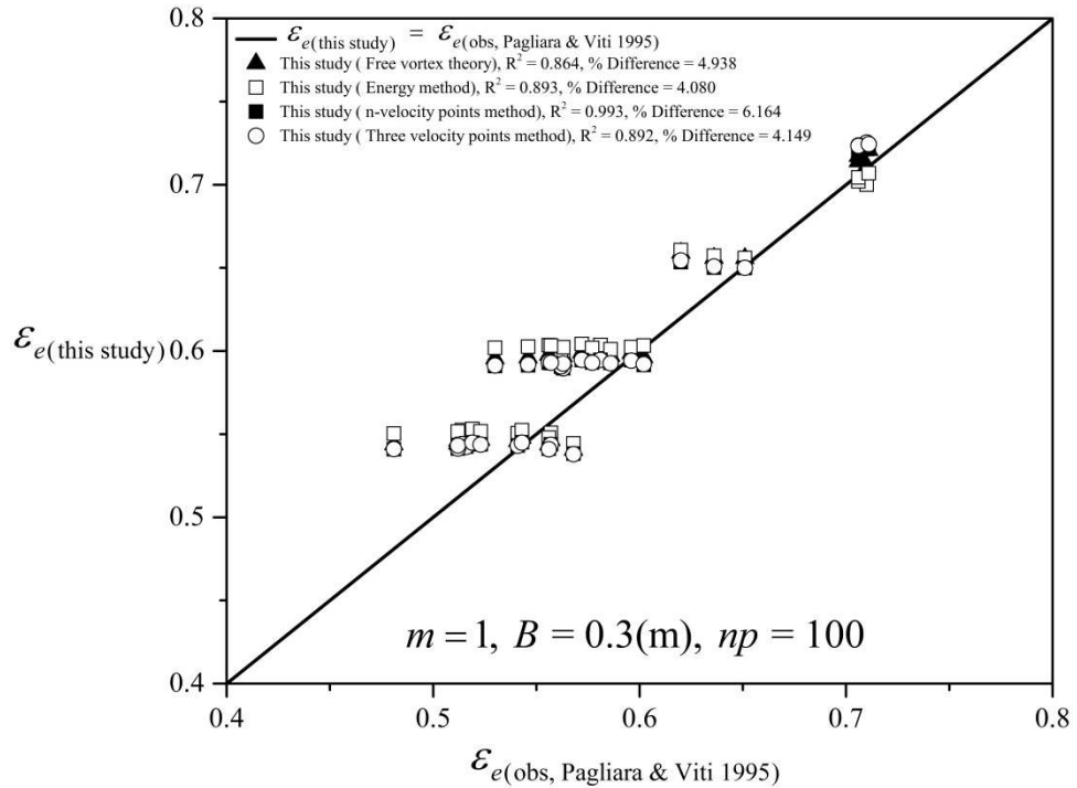
Figure 5.13: Comparison between \varepsilon_e values based on four suggested methods and \varepsilon_e values based on the experimental data sets of Pagliara and Viti (1995) in trapezoidal channel cross-sections at super critical flow regimes
