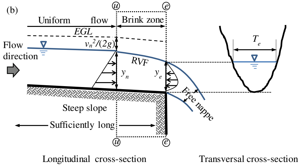
Figure 1.1: (a) Sketch of a free over-fall along the longitudinally mild slope; (b) the longitudinally steep slope, for general channel cross-section with the proposed pressure distribution over the control volume between the upstream section ( u-u ) and the end section ( e-e ) with the transversal cross-section
