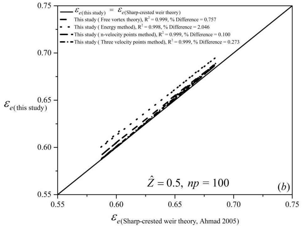
Figure 5.24: \mathcal{E}_e values based on the suggested methods of this study versus (a) \mathcal{E}_e values based on the theoretical study of Dey (2003) using Boussinesq approach; and (b) \mathcal{E}_e values based on the theoretical study of Ahmed (2005) using sharp-crested weir theory in circular channel with \hat{Z} = 0.5
