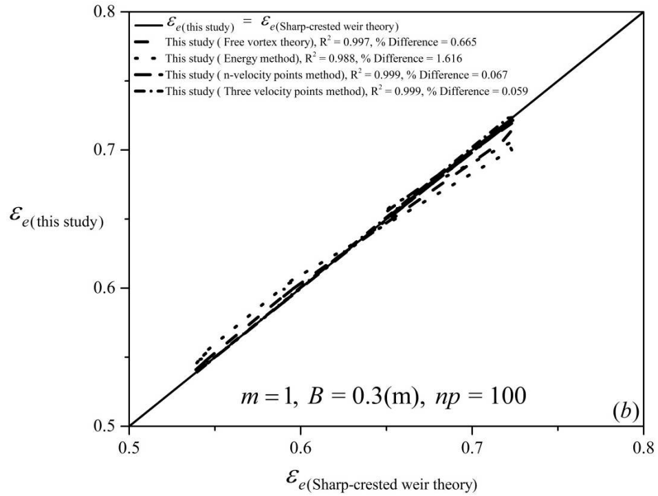
Figure 5.14: Comparison between \mathcal{E}_e values based on four suggested methods and \mathcal{E}_e values obtained based on the theoretical study (a) of Murty Bhallamudi (1994); and (b) the sharp-crested weir theory in trapezoidal channel cross-sections in super critical regimes
