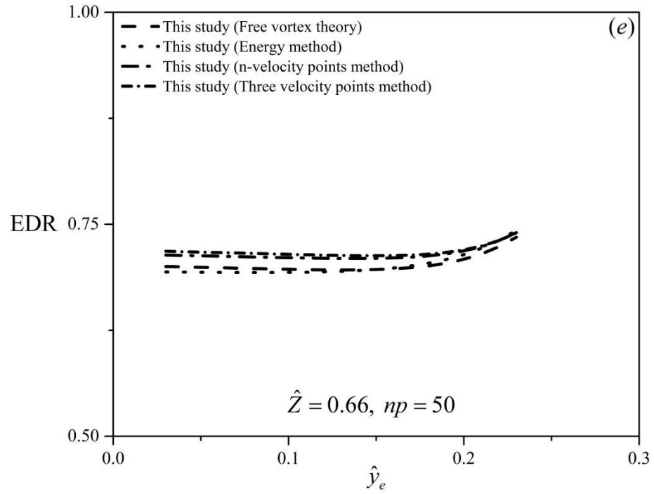
Figure 5.18: EDR values based on the proposed methods of circular channel cross-section with flat-base for (a) \hat{Z} = 0 ; (b) \hat{Z} = 0.25 ; (c) \hat{Z} = 0.33 ; (d) \hat{Z} = 0.5 ; and (e) \hat{Z} = 0.66 at sub-critical flow regimes
