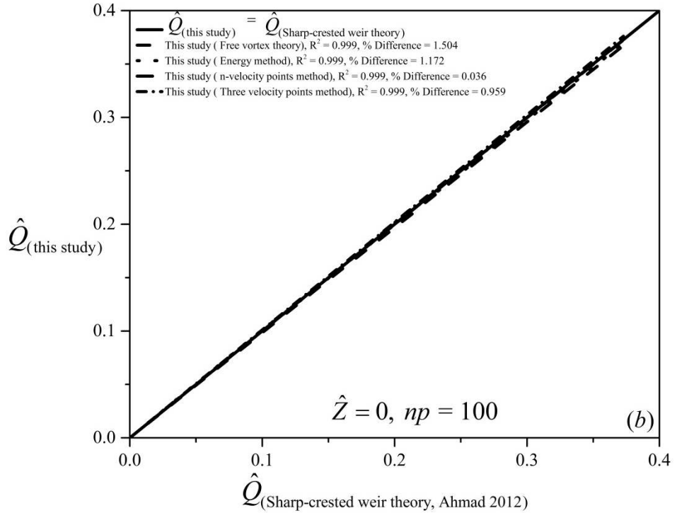
Figure 5.25: Comparison between the computed non-dimensional discharges ( \hat{Q} ) of the suggested methods of this study with (a) the theoretical \hat{Q} results of Dey (1998); and (b) the theoretical \hat{Q} results of Ahmad (2012) for the circular channel cross-section at super critical flow regime with \hat{Z} = 0
