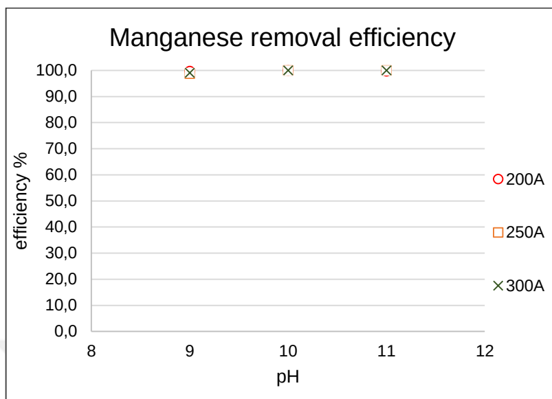
Figure 4.41. Manganese removal efficiency with iron electrodes, pH balanced at E&E output
