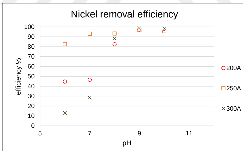
Figure 4.35. Nickel removal efficiency with aluminum electrodes, double reaction time and pH balanced at E&E output
