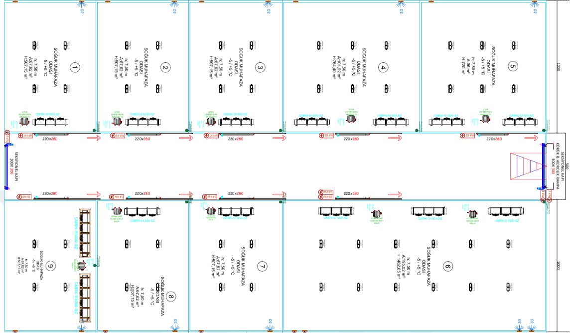
Figure 4.5. Pilot Facility Plan
