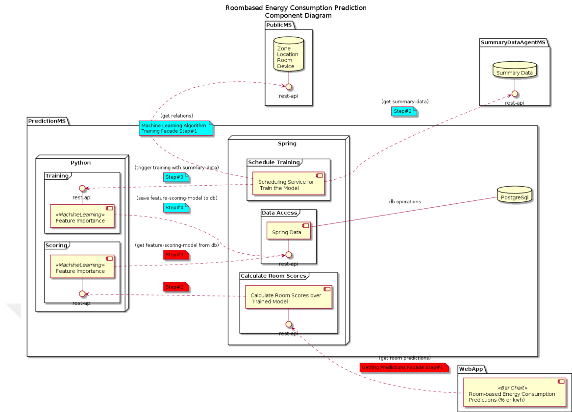
Figure 3.4. Component Diagram of Room-based Consumption Prediction
