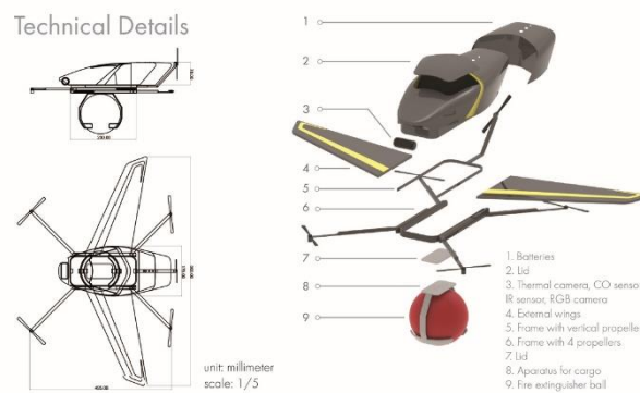
Figure 4.54. Technical representation example, section drawing and exploded render (Student 6)
