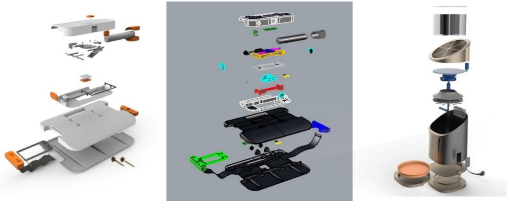
Figure 4.58. Inner parts representation examples. Left: Inner part representation with 3D-model and render (Student 1) and Right: Inner part representation with render (Student 2)
