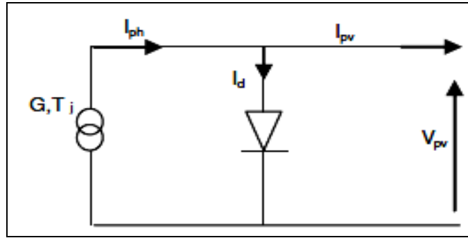
Figure 2.1 Simplified equivalent circuit of solar cell (Rekioua & Matagne, 2012)
