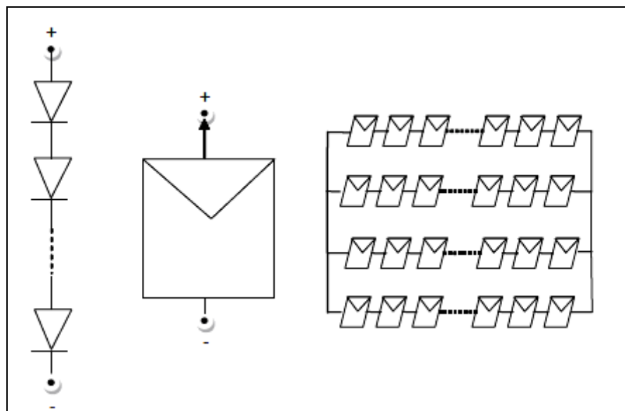
Figure 2.3 Cells, photovoltaic module and panel (respectively)
