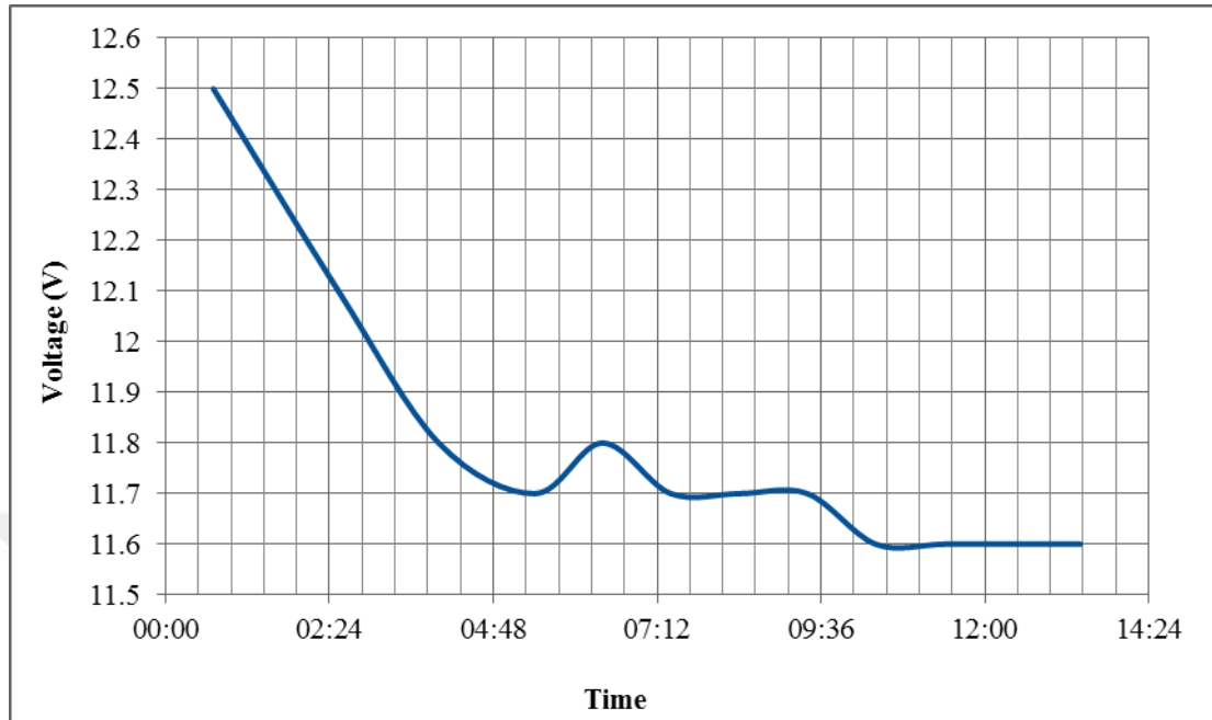
Figure 4.1 Discharge graphic of Eurostar batarries on 9th of July
