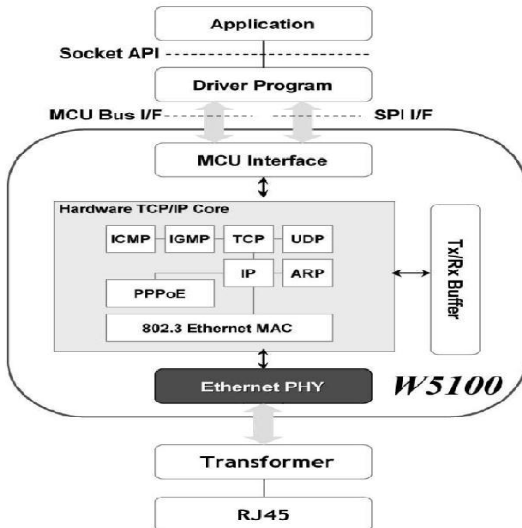
Figure 4.3 W5100 block diagram
