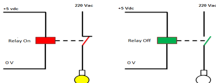
Figure 3.9 Relay and light connection
