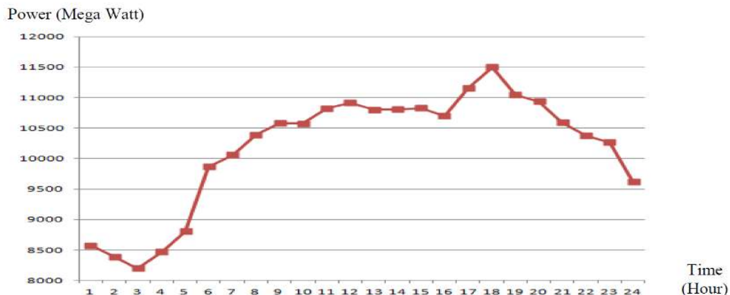
Figure 1.1 Energy consumption profile for (22/7/2012) in Iraq [9]
