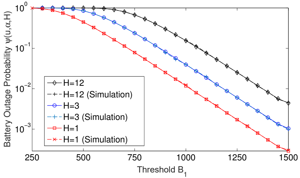
Figure 4.4: Battery outage probability as a function of B_1 for H = 1, 3, 12 and u = 3000 , \lambda_{\min} = 0.4 , \lambda_{\max} = 10 , \alpha = [5/6 \ 1/6] .
