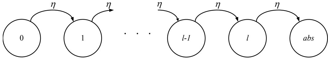
Figure 3.1: l -level Erlangization of the horizon H .
