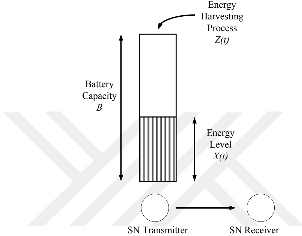
Figure 1.3: Energy harvesting SN model.
