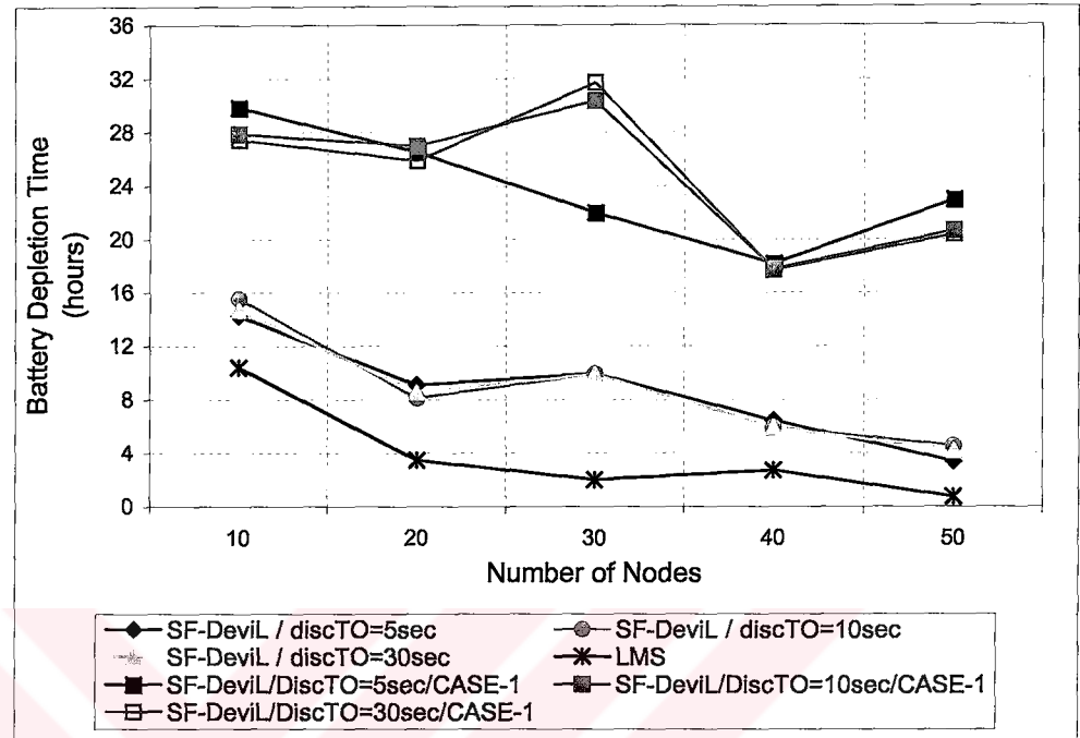
Figure 5.3: Time until the battery of first device depletes with scatternet update CASE-1
