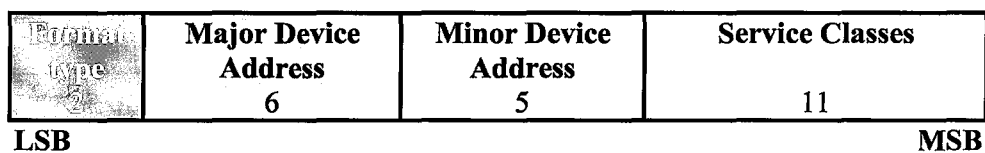
Figure 2.7: Structure of the Class of Device/Service field (first format type)
