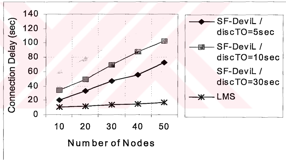
Figure 5.12: Scatternet formation delay
