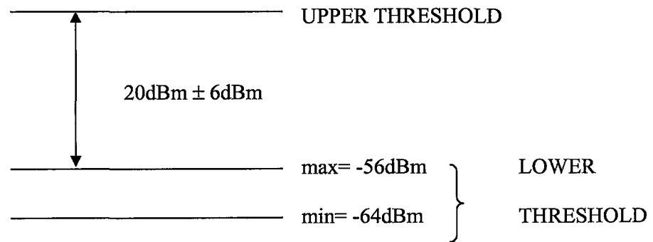
Figure 2.12: RSSI dynamic range and accuracy
