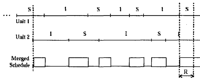
Figure 2.11: Nodes alternate between inquiry (I) and inquiry scan (S) substates until they connect
