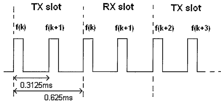
Figure 2.9: RX/TX cycle of Bluetooth transceiver in Inquiry mode
