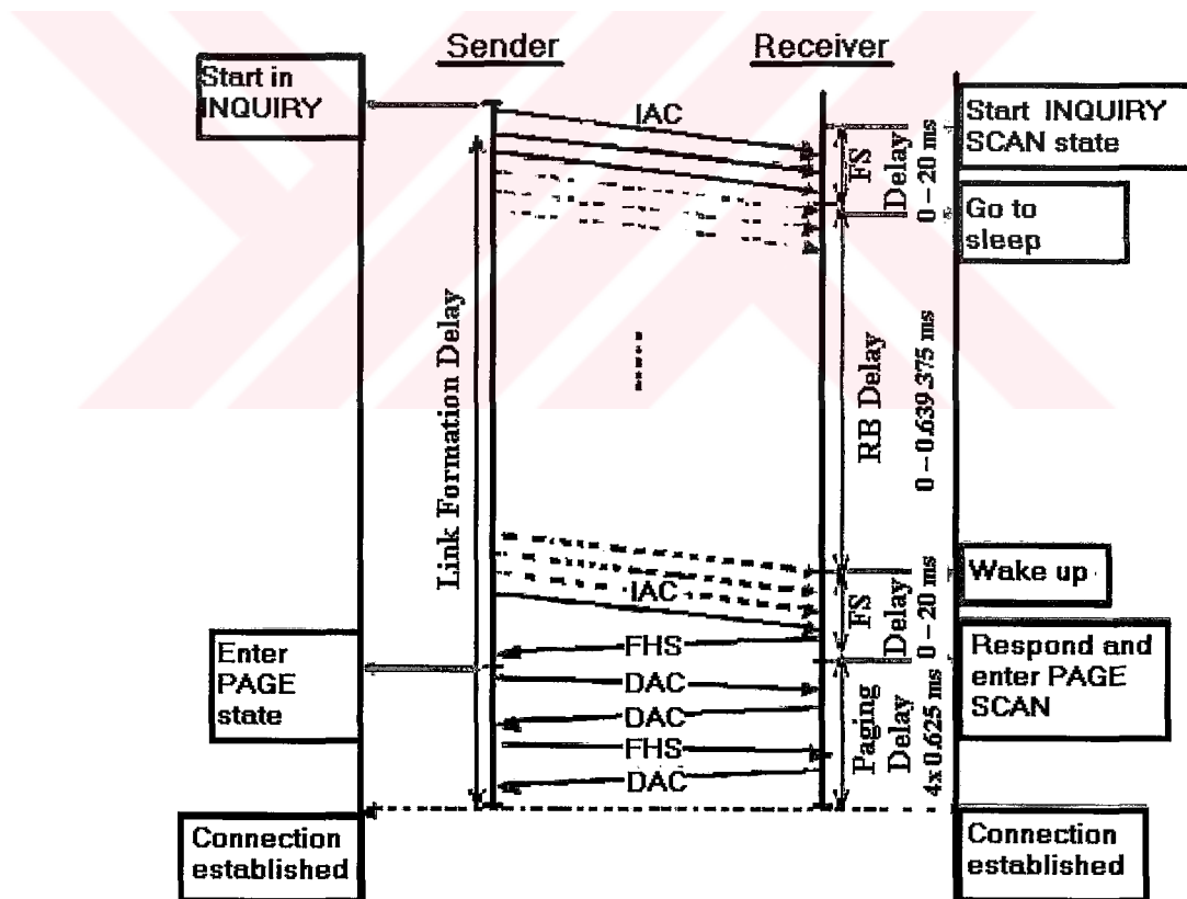
Figure 2.10: Bluetooth link formation
