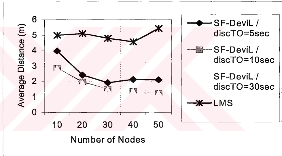
Figure 5.9: Average length of links in the scatternet
