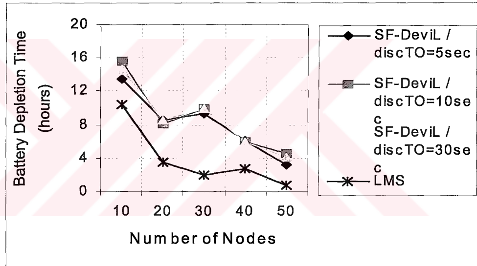
Figure 5.2: Time until the battery of first device depletes
