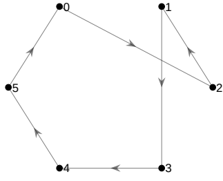
(a) New tour: 0-2-1-3-4-5
