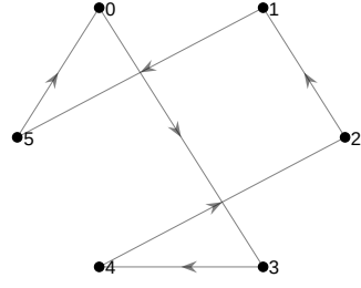
(c) Tour: 0-3-4-2-1-5
