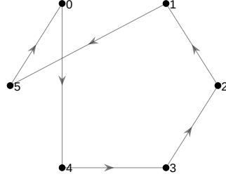
(c) New tour: 0-4-3-2-1-5
