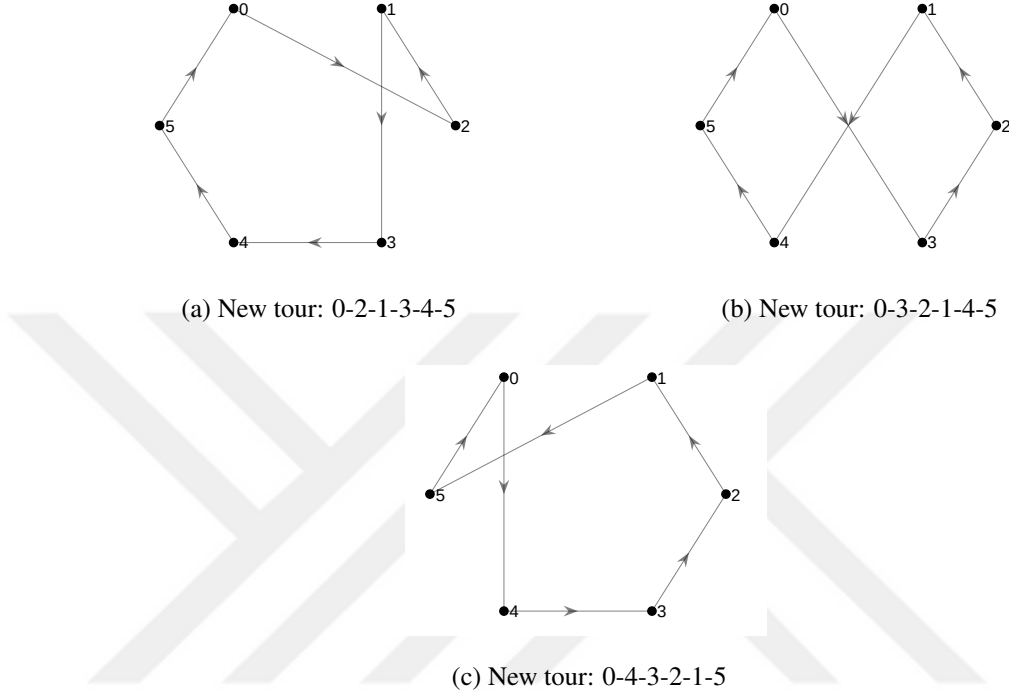
Figure 4.2: The illustrations of the 2-opt moves
