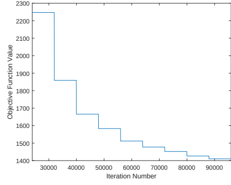
(b) 3-opt algorithm
