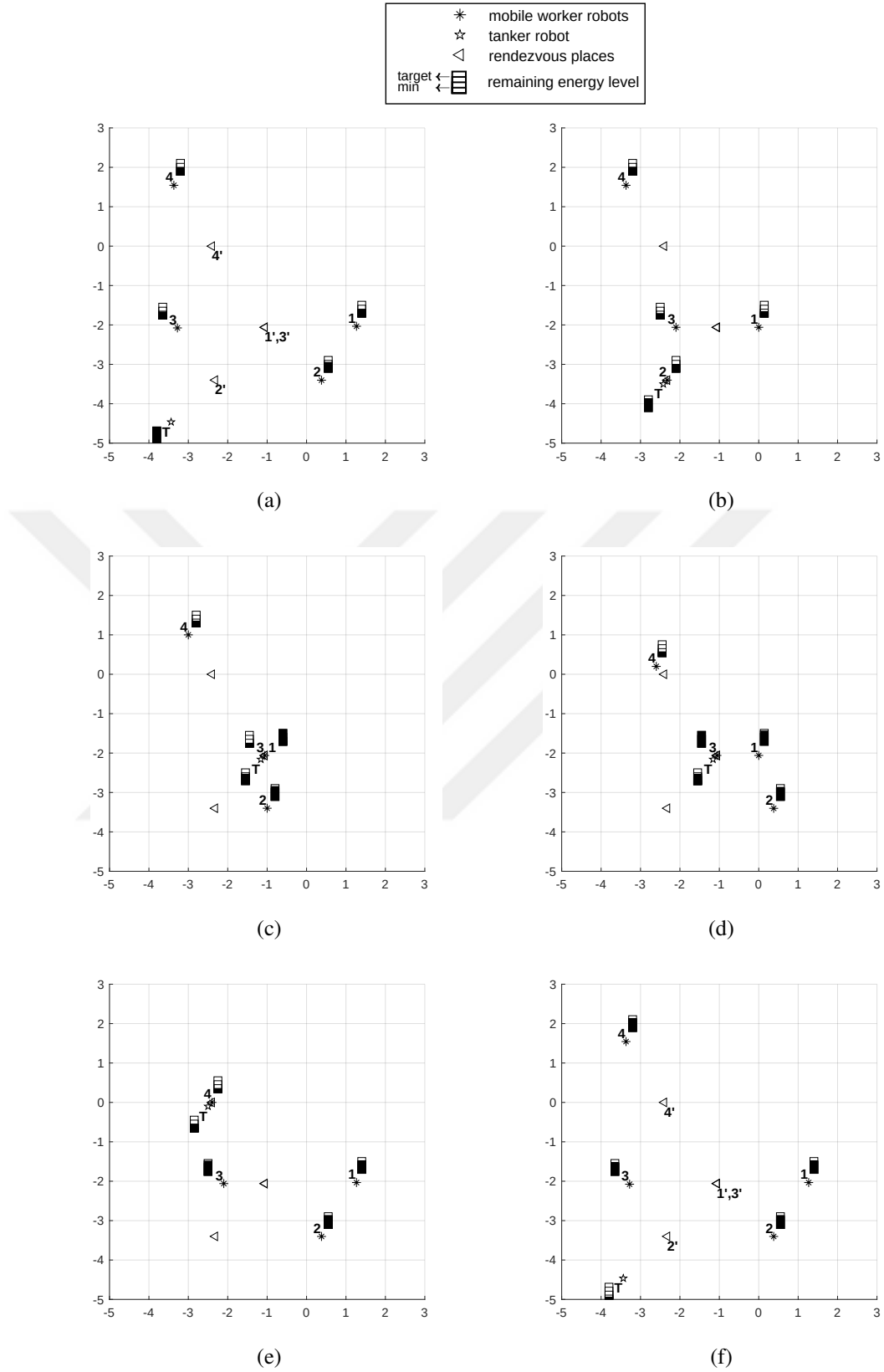
Figure 3.1: Illustrative example where the meeting order is 2 – 1 – 3 – 4
