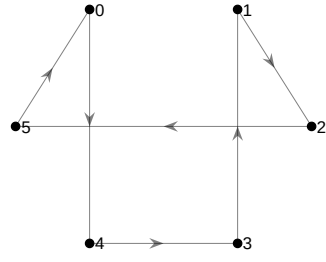
(a) Tour: 0-4-3-1-2-5
