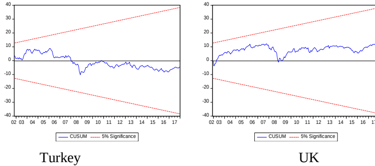
Figure 3. 1. Cusum test
