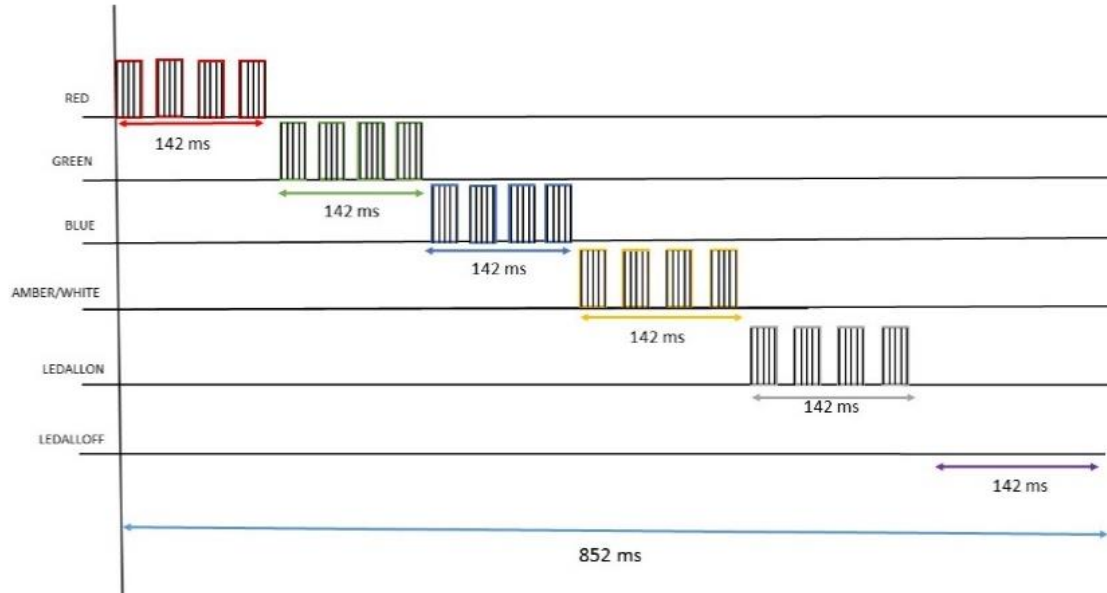
Figure 51 Light pulses of BSSL at 7 Hz
