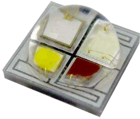
Figure 31 Federal 5050 Series LED chip [48]
