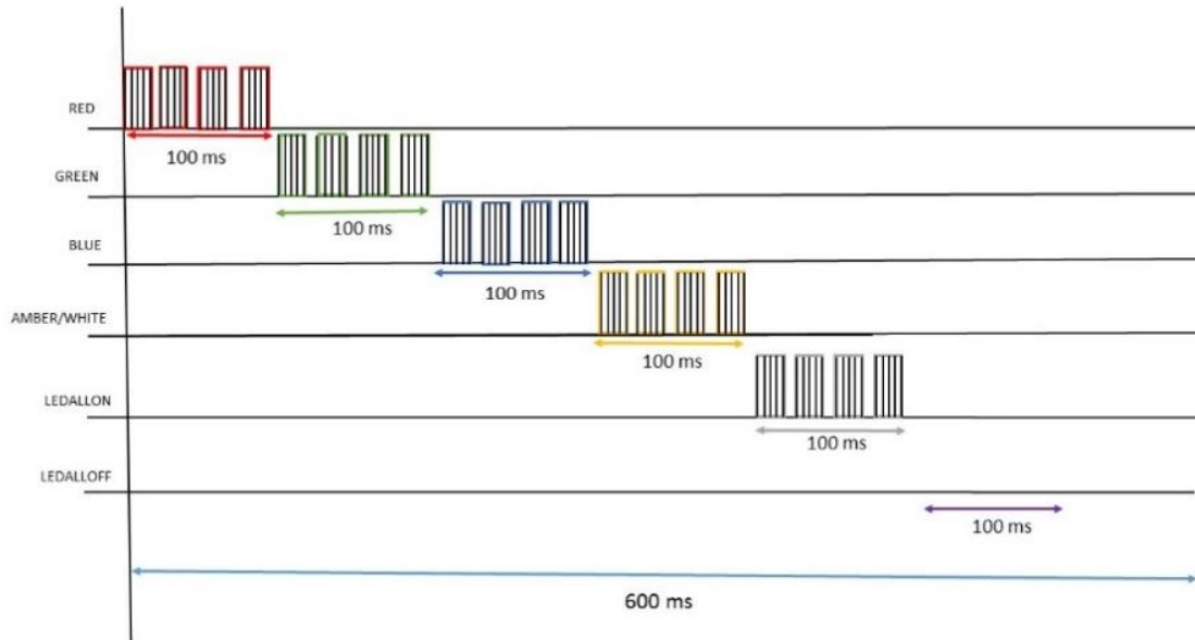
Figure 52 Light pulses of BSSL at 10 Hz
