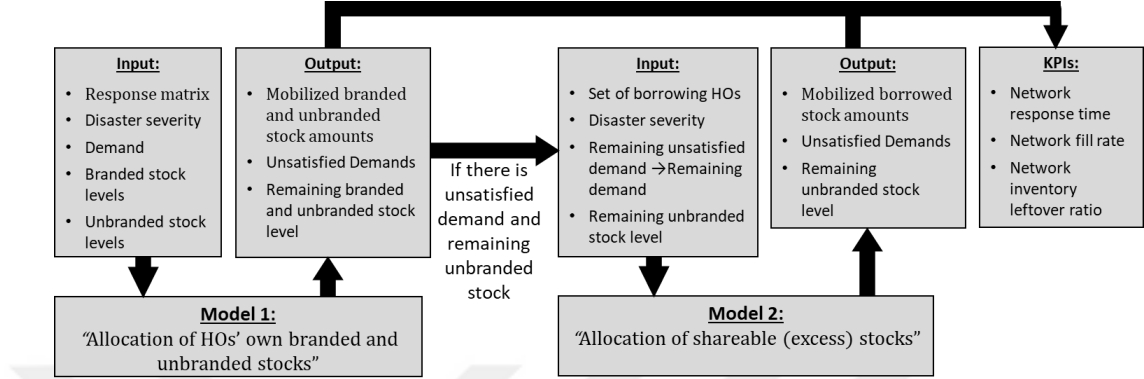
Figure 4: The illustration of the two-phase decision-making framework for inventory allocation
