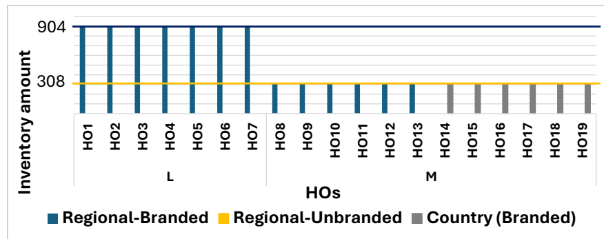
Figure 37: Distribution of each HO’s initial inventory level under the base case
