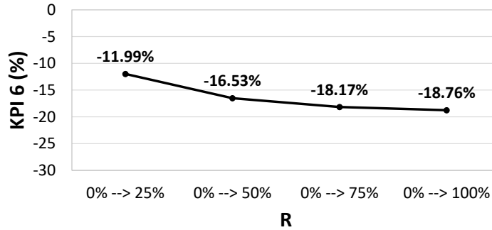
Figure 15: KPI_2^2 values for severe disaster severity level ( \lambda = 2 )
