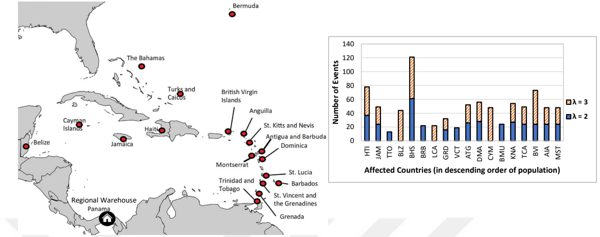
Figure 8: Region of interest and distribution of disaster events
