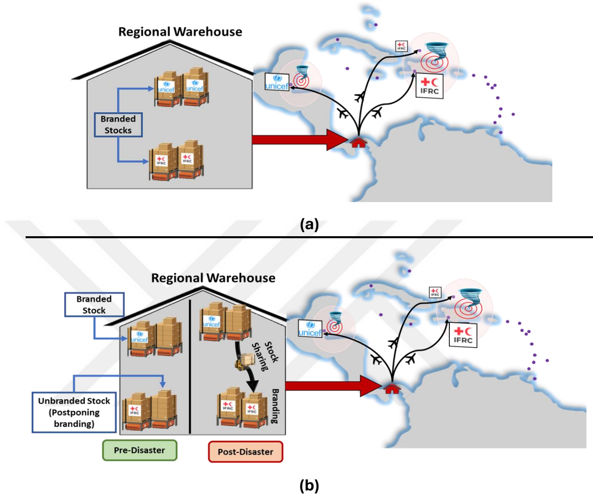
Figure 1: The illustration of the network: (a) current; (b) proposed
