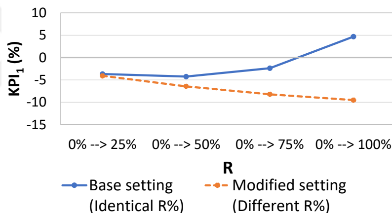
Figure 22: KPI_1 values for base and modified settings
