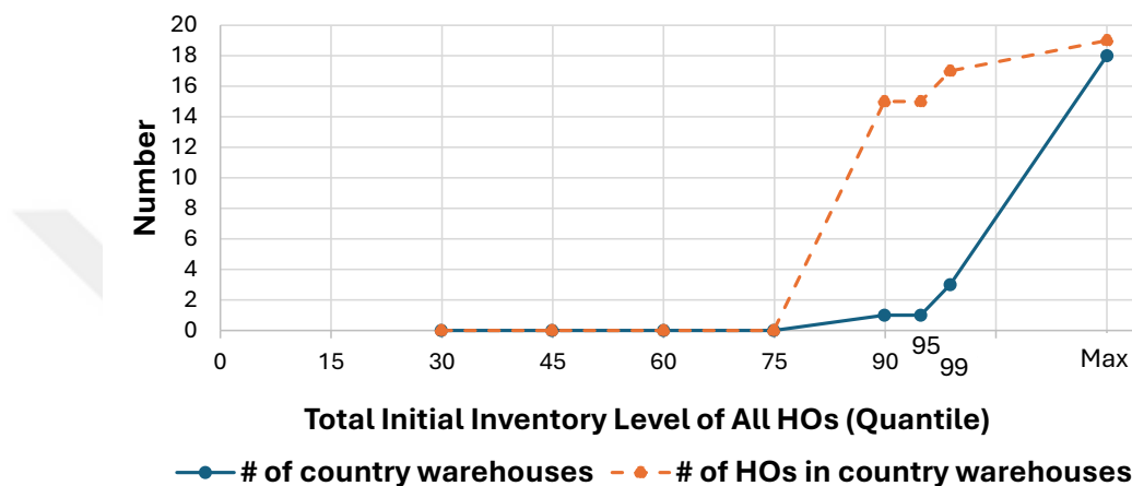
Figure 40: HOs' initial inventory location decisions under varying total initial inventory level
