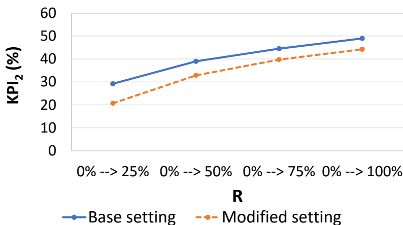
Figure 23: KPI_2 values for base and modified settings
