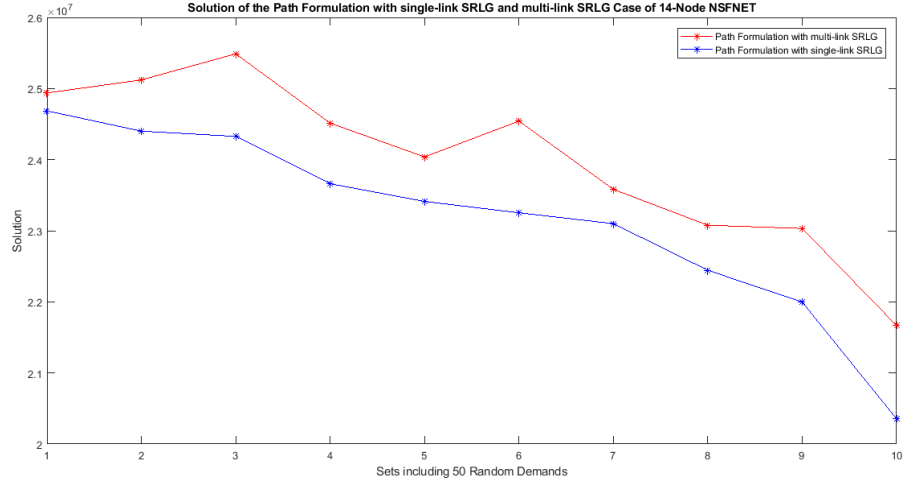
Figure 4.4: Path Formulation with multi-link SRLG and single-link SRLG for 14-Node NSFNET
