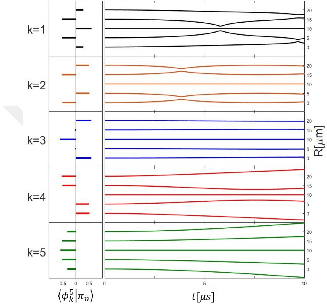
Figure 4.1: The initial electronic eigenvectors of a regular chain with five atoms "left side" and the atomic trajectories "right side", when the system is prepared in the respective eigenvector on the left side.
