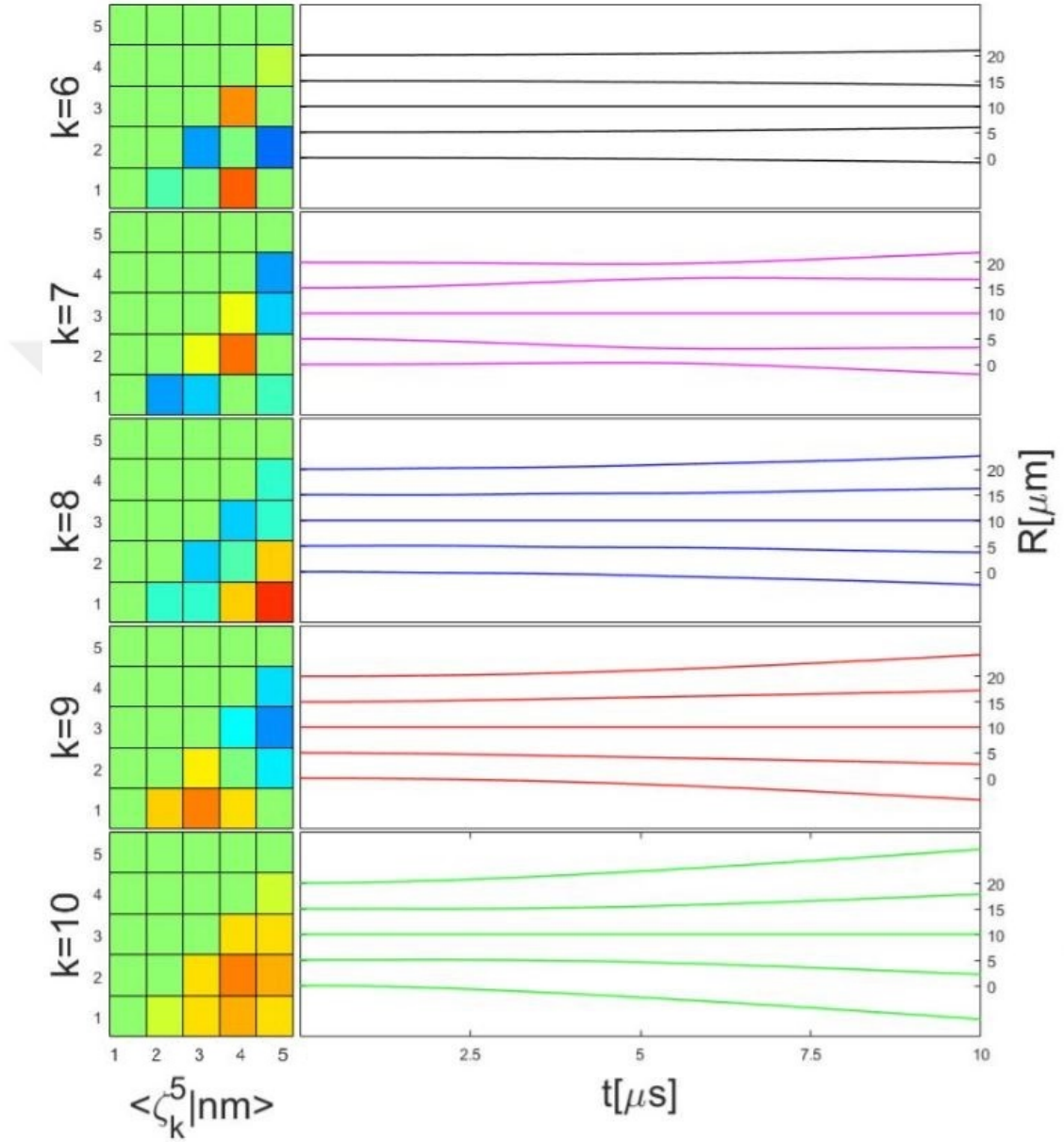
Figure 4.3: The electronic eigenvectors 6-10 of a regular chain of five atoms with two excitations "left side" and the atomic trajectories "right side", when the system is prepared in the respective eigenvector on the left side. The colors on the left side follow the same color pattern as of Fig. 3.6
