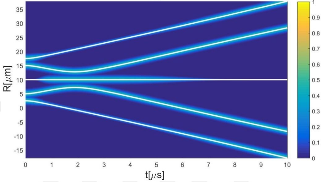
Figure 4.4: Atomic trajectories (white lines) with excitation density for the states \zeta_{10}^5 of a dislocated chain at two ends.
