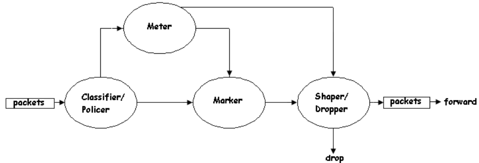
Figure 2.2: DiffServ QoS Traffic Conditioning Flow Chart
