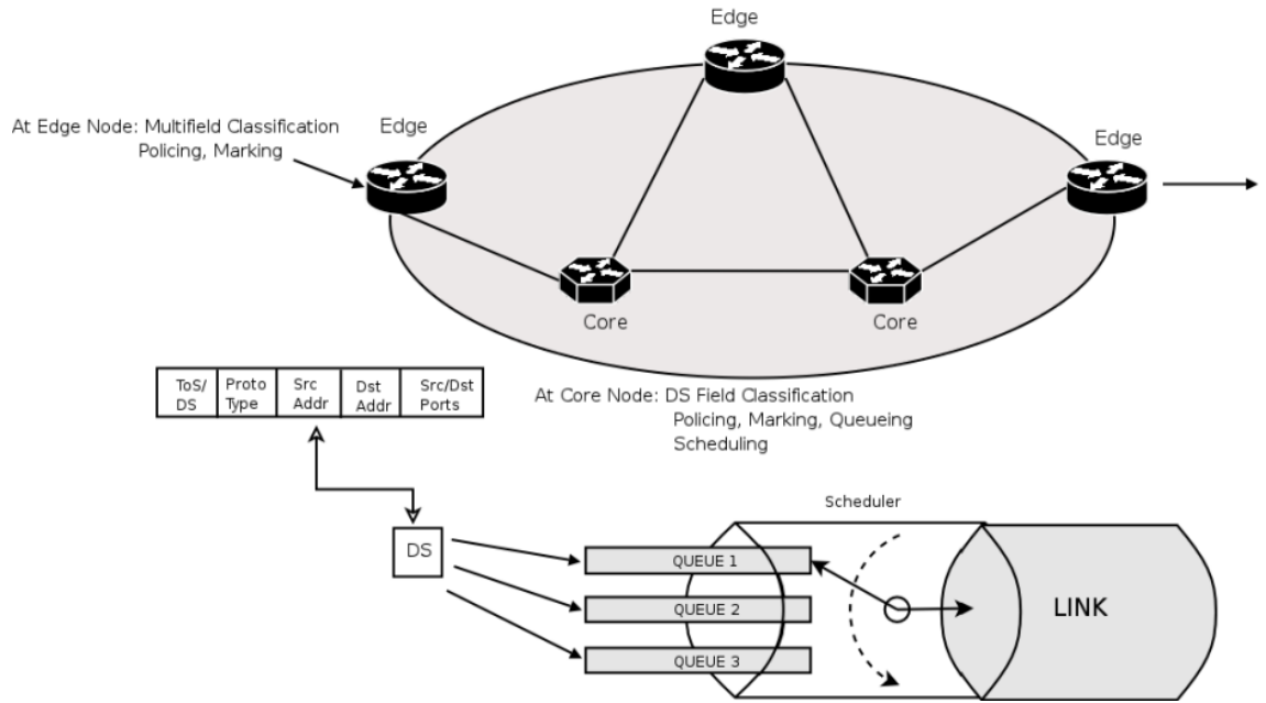
Figure 2.1: DiffServ Architecture
