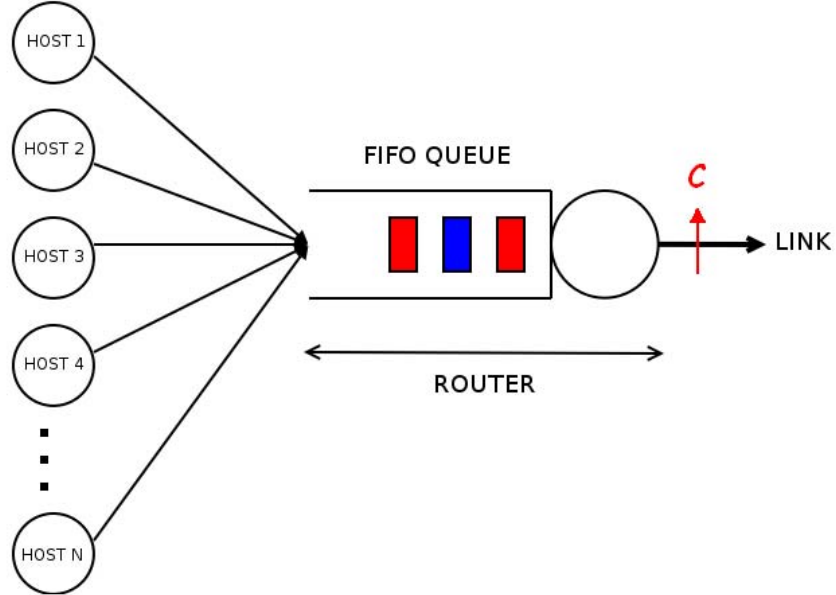
Figure 4.1: System Model
