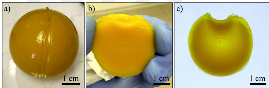
Figure 23. Formation of precipitation patterns in 3D in 8 w% agarose sphere. (a) Agarose sphere removed from 1 M K_2CrO_4 outer electrolyte solution. (b) Cross section of 3D sample. (c) Thin layer cut from sample for rings detection. Inner electrolyte (copper chloride) = 0.01 M, outer electrolyte (potassium chromate) = 1 M, T=20\text{ }^{\circ}C . For details of the gel preparation please see Chapter 2.
