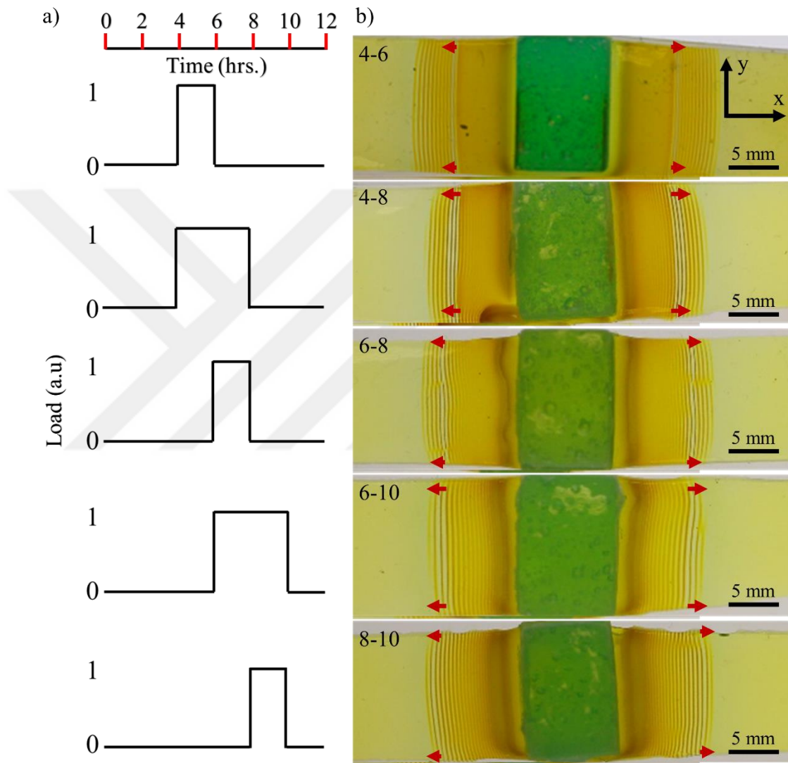
Figure 35. Cyclic deformation in 1D polyacrylamide (PAA) hydrogels. Samples are mechanically loaded/unloaded (stretched/released) in x-direction through cycles as shown in (a); Vertical axis 0 = unloaded (released/unstretched), and 1 = loaded (stretched) sample. (b) The patterns formed in cyclic loading and unloading (x-direction). Inner electrolyte (potassium chromate) = 0.01 M, outer electrolyte (copper chloride) = 1 M, acrylamide = 13.5 w%, BIS = 0.056 w%, KPS = 0.187 w%, TEMED
