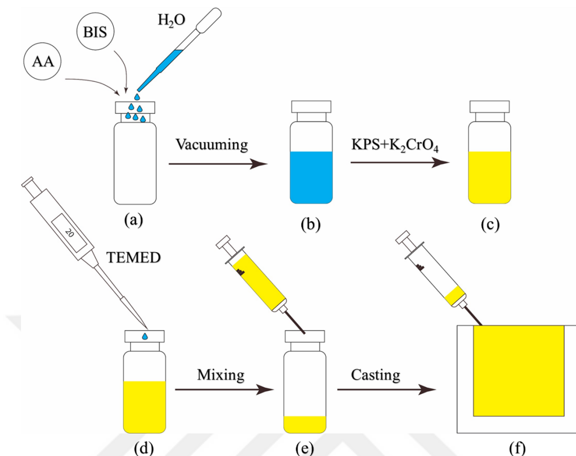
Figure 9. Preparation and cast molding of polyacrylamide (PAA) hydrogel. (a) Acrylamide (AA) and Bis-acrylamide (BIS) are dissolved in deionized water. (b) Solution is degassed under vacuum for 20 minutes. (c) KPS and K_2CrO_4 are added and mixed carefully to the solution not to introduce further oxygen in the sample. (d) Addition of TEMED and gelation initiation in prepared solution after addition of TEMED. (e and f) Casting of solution in plexiglass mold before first gelation stage complete using syringe.
