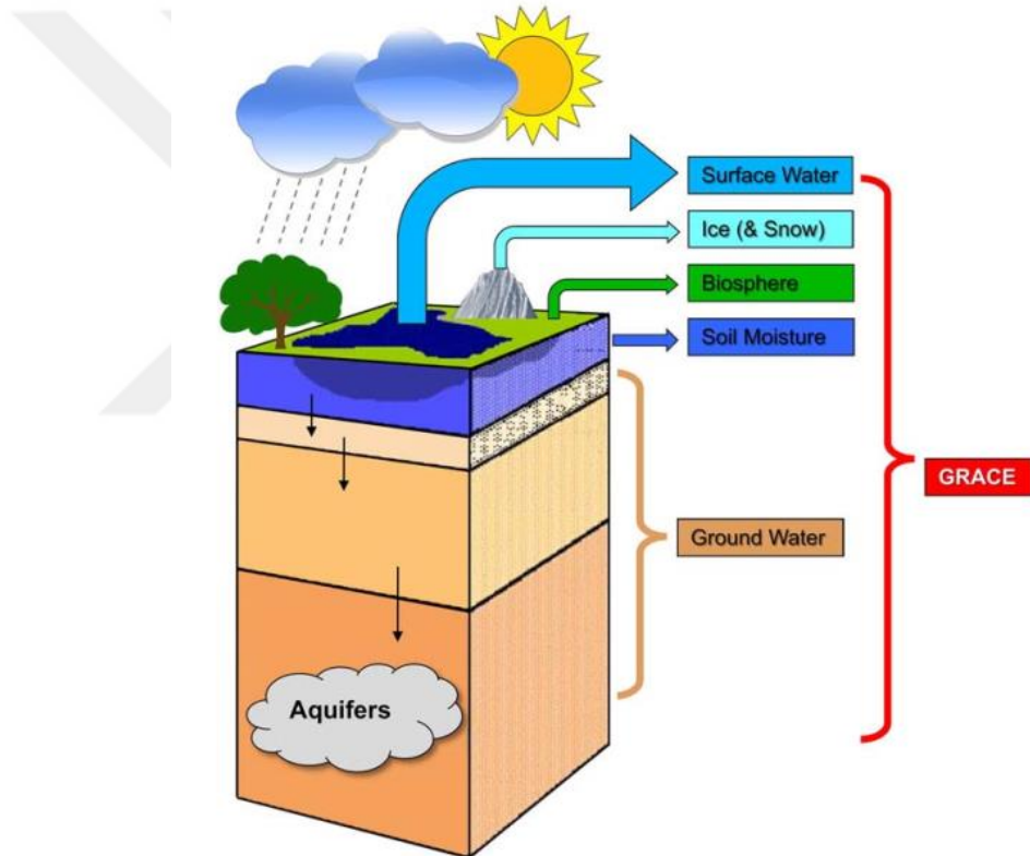
Figure 3.4: The variables of GRACE Terrestrial water storage (Cazenave & Chen, 2010)
