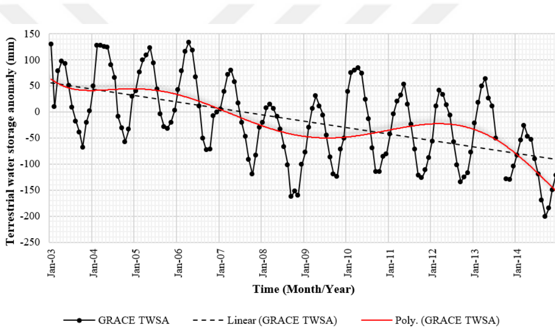
Figure 5.1: Monthly mean Terrestrial water storage anomaly derived from GRACE data.
