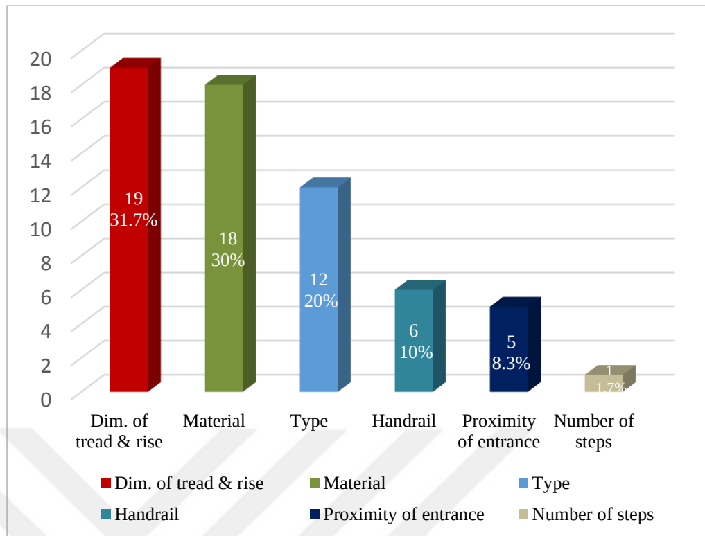
Figure 9. Graph Showing Negatively Affecting Design Characteristics of Staircase (n=60)
