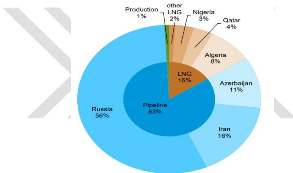
Figure 4-3_Turkey's Natural Gas Supply by Source, 2015
