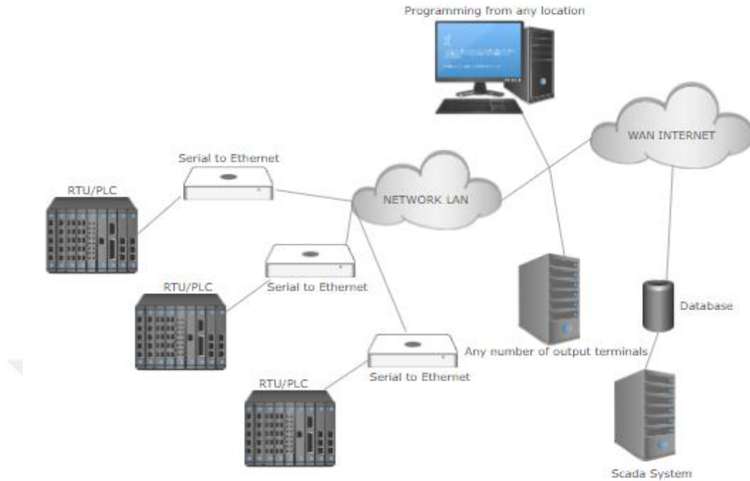
Figure 4.1: Programming from any Location
