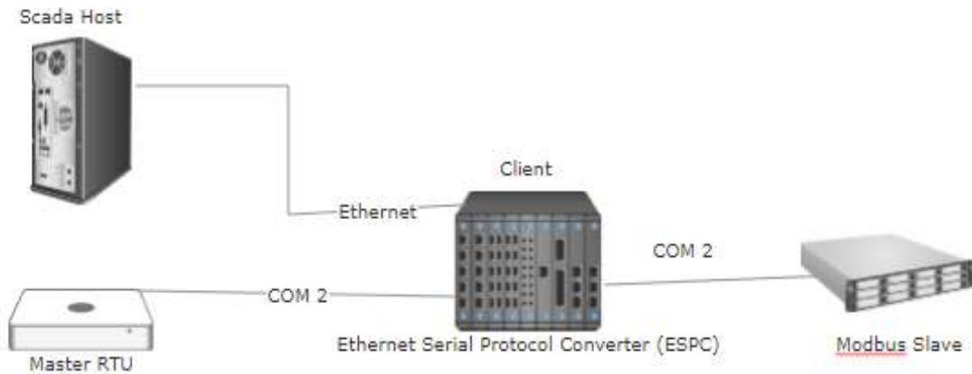
Figure 4.5: Connect methodology of Ethernet serial protocol.
