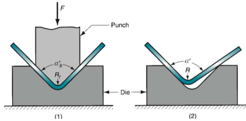
Figure 1.4: Springback Phenomenon.
