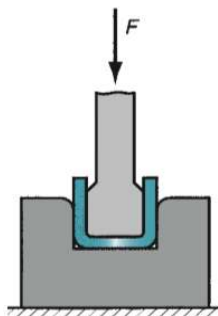
Figure 1.3c: Channel
