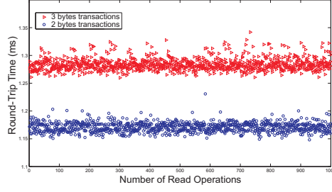
Figure 4.3: Round-trip time between the request and response of 1000 targeted read transactions from 2 and 3 bytes long outboxes.
