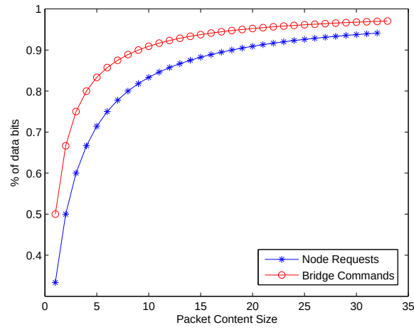
Figure 4.1: Uplink packet overhead.
