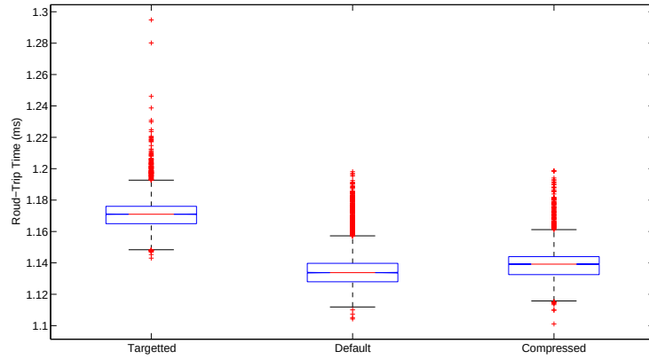
Figure 4.5: Mean and variance of round-trip times between the request and response of 10000 read transactions from 2 bytes long outboxes for each transaction type.
