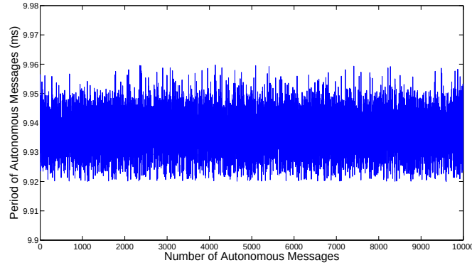
Figure 4.7: Period of 10000 autonomous responses generated for every 10 ms.
