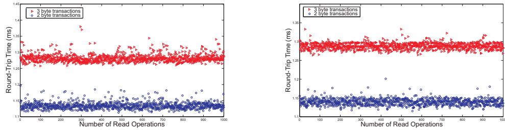
Figure 4.4: Round-trip time between the request and response of 1000 a) default b) compressed read transactions from 2 and 3 bytes long outboxes.
