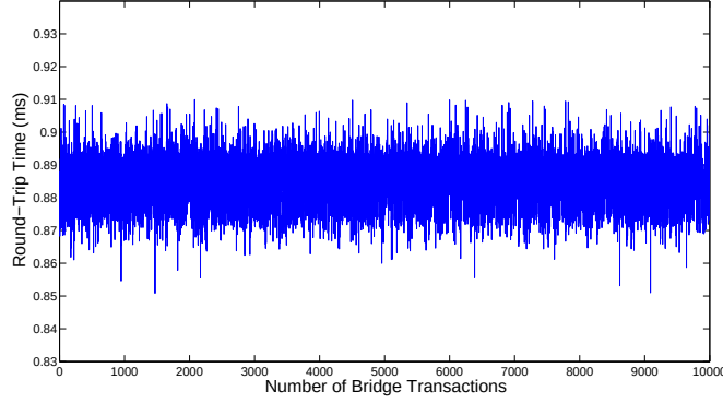
Figure 4.6: Round-trip time between the request and response of 10000 targeted BRG_LED_COMMANDS.
