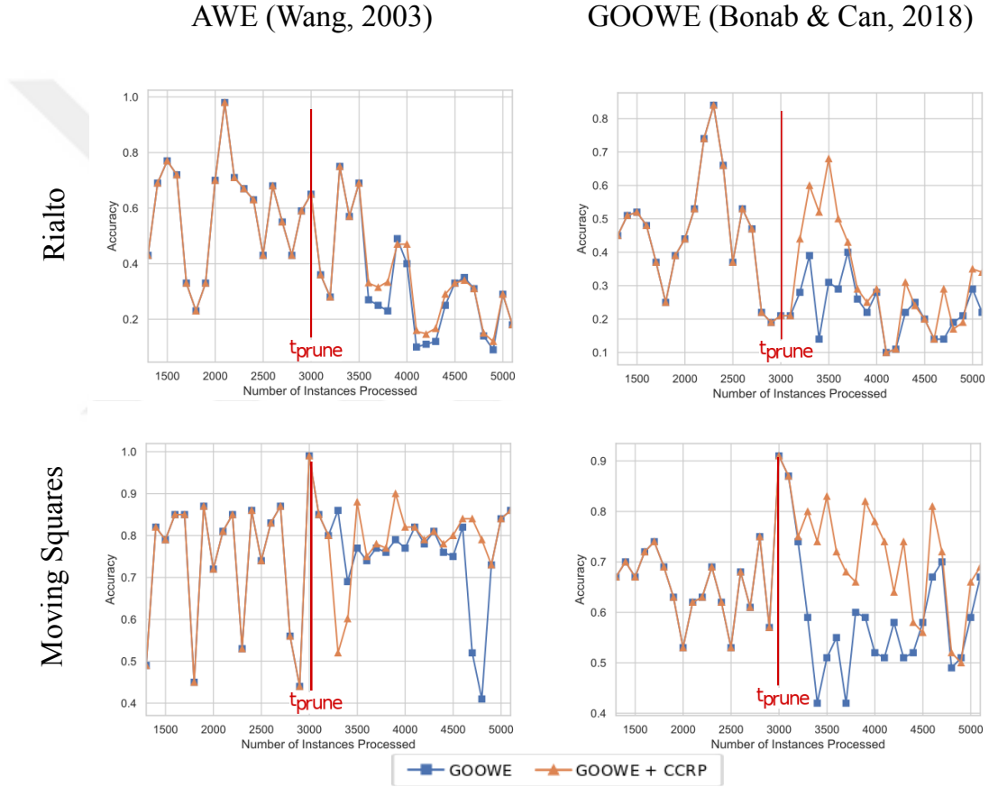
Figure 5.1: The impact of CCRP ( \varphi = L ) on the prequential accuracy over one real and one artificial dataset. Orange lines with triangles represent the CCRP applied models and blue lines with squares represents the models without CCRP. The first occurrence of pruning is denoted with red vertical line which is labeled t_{prune} .
