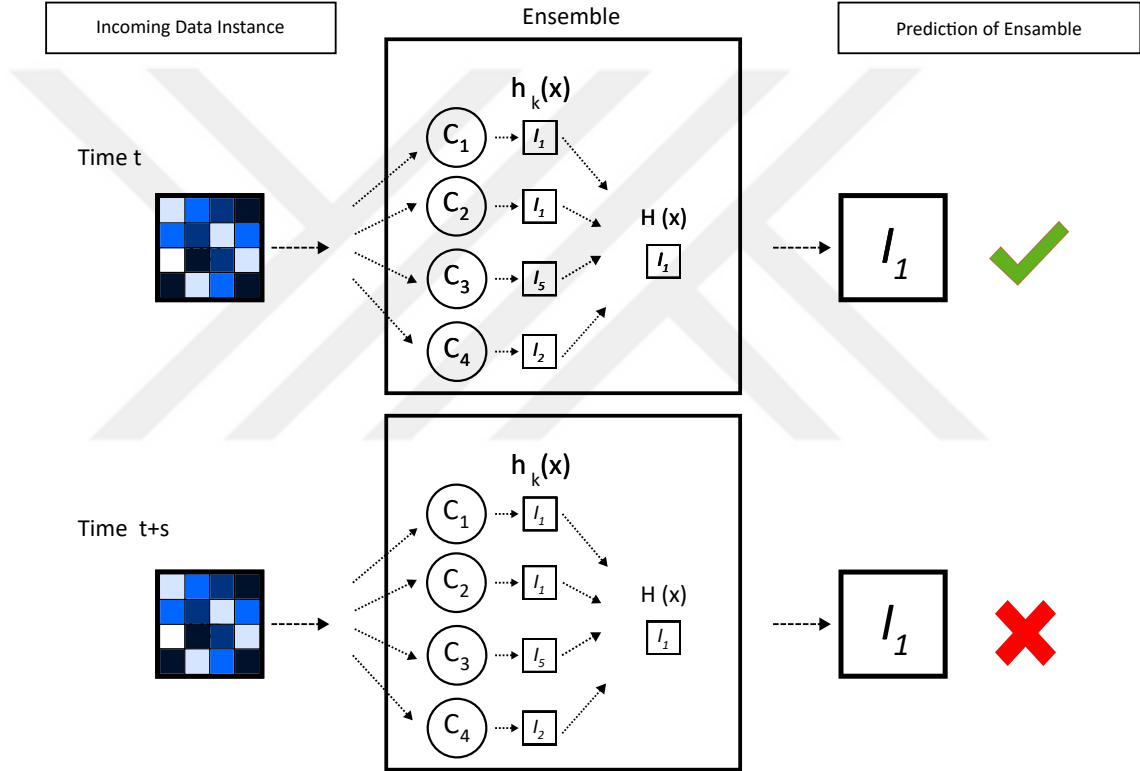
Figure 2.1: Stream data classification under concept drift. Feature-wise the same input data instances are classified by the ensemble at 2 different time points. Ensemble makes the same prediction for the input data; however, the prediction is correct for time t , it is incorrect for time t+s . If this behaviour is consistent for a time period, we can say that a concept drift occurred during the time interval [t, t+s] . Misprediction at time t+s , shows that the learned information by the components of the ensemble became obsolete.
