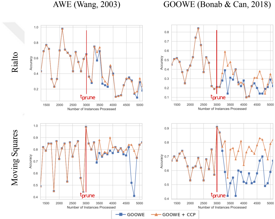
Figure 5.2: The impact of CCP ( \varphi = L ) on the prequential accuracy over one real and one artificial dataset. Orange lines with triangles represent the CCP applied models and blue lines with squares represents the models without CCP. The first occurrence of pruning is denoted with red vertical line which is labeled t_{prune} .
