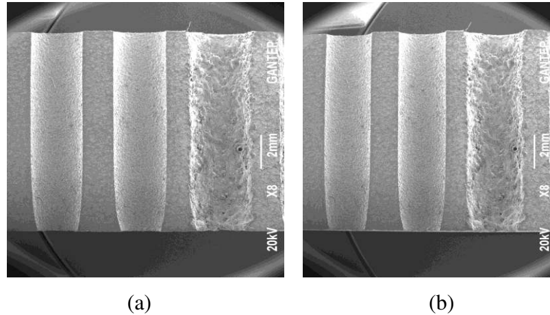
Figure 3.7 SEM images (a) D2NiBr 9-10-11x8 ve (b) D2NiBr 9-10-11x8+10deg with x8 magnification and +10deg tilting
