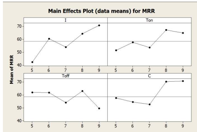
Figure A.4 D2TiBr MRR Main Effects Graphs
