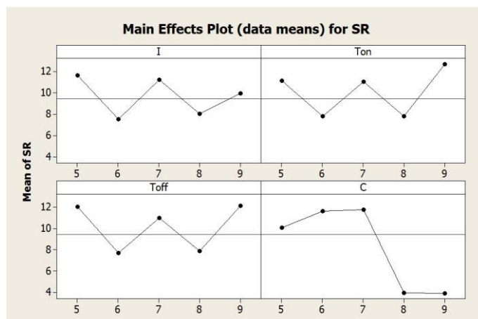
Figure A.6 D2TiBr Ra Main Effects Graphs
