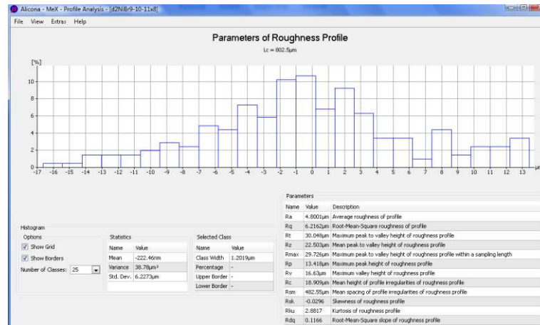
Figure 3.10 Roughness results
