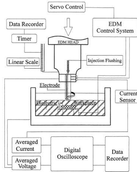
Figure 2.7 Schematic diagram of the experimental set-up for EDMbHd process. [17]
