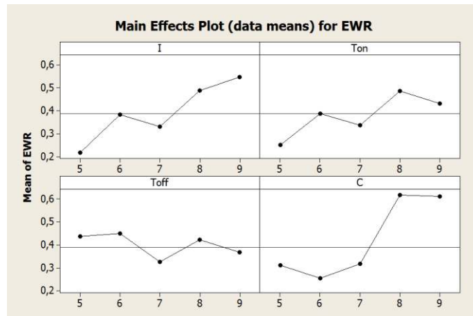
Figure A.5 D2TiBr EWR Main Effects Graphs
