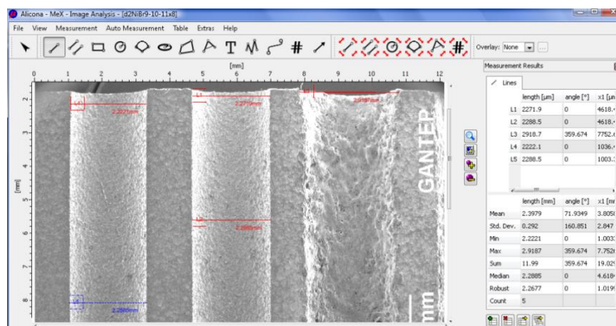
Figure 3.12 Linear measurements
