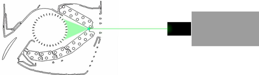
Figure 3.90 The schematic of the EPIV setup for investigating the area between the heat exchanger and the CFF.
