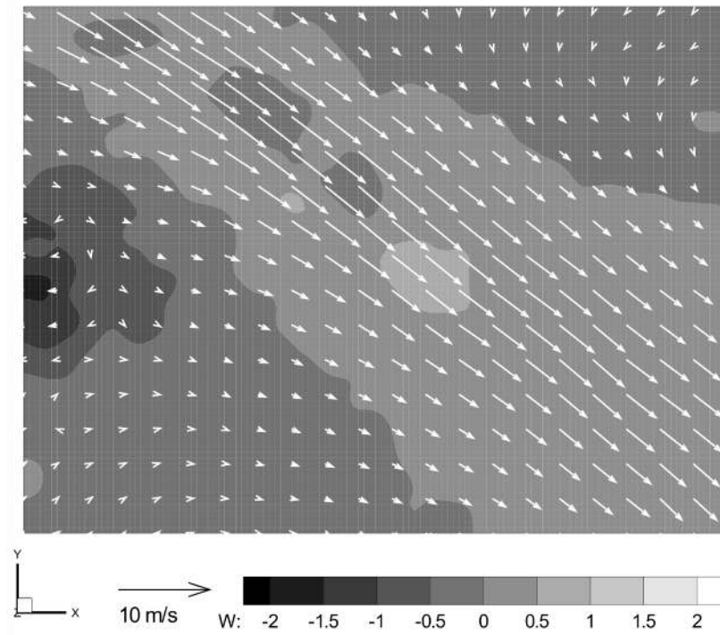
Figure 3.12 Average three dimensional velocity distribution of the skewed CFF used SAC on investigation plane 3.
