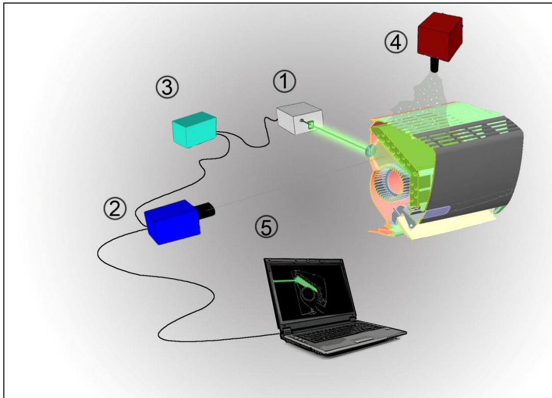
Figure 2.24 Schematic of a EPIV setup that the laser beam sent on a cylindrical lens for creating the light sheet.
