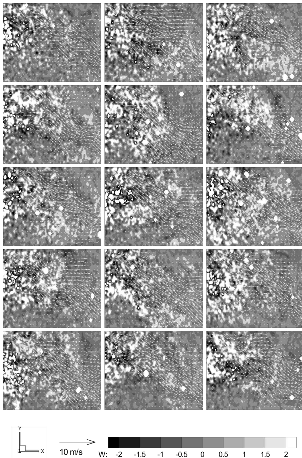
Figure 3.77 The instantaneous SPIV results at investigation plane 7 of a skewed CFF used SAC.
