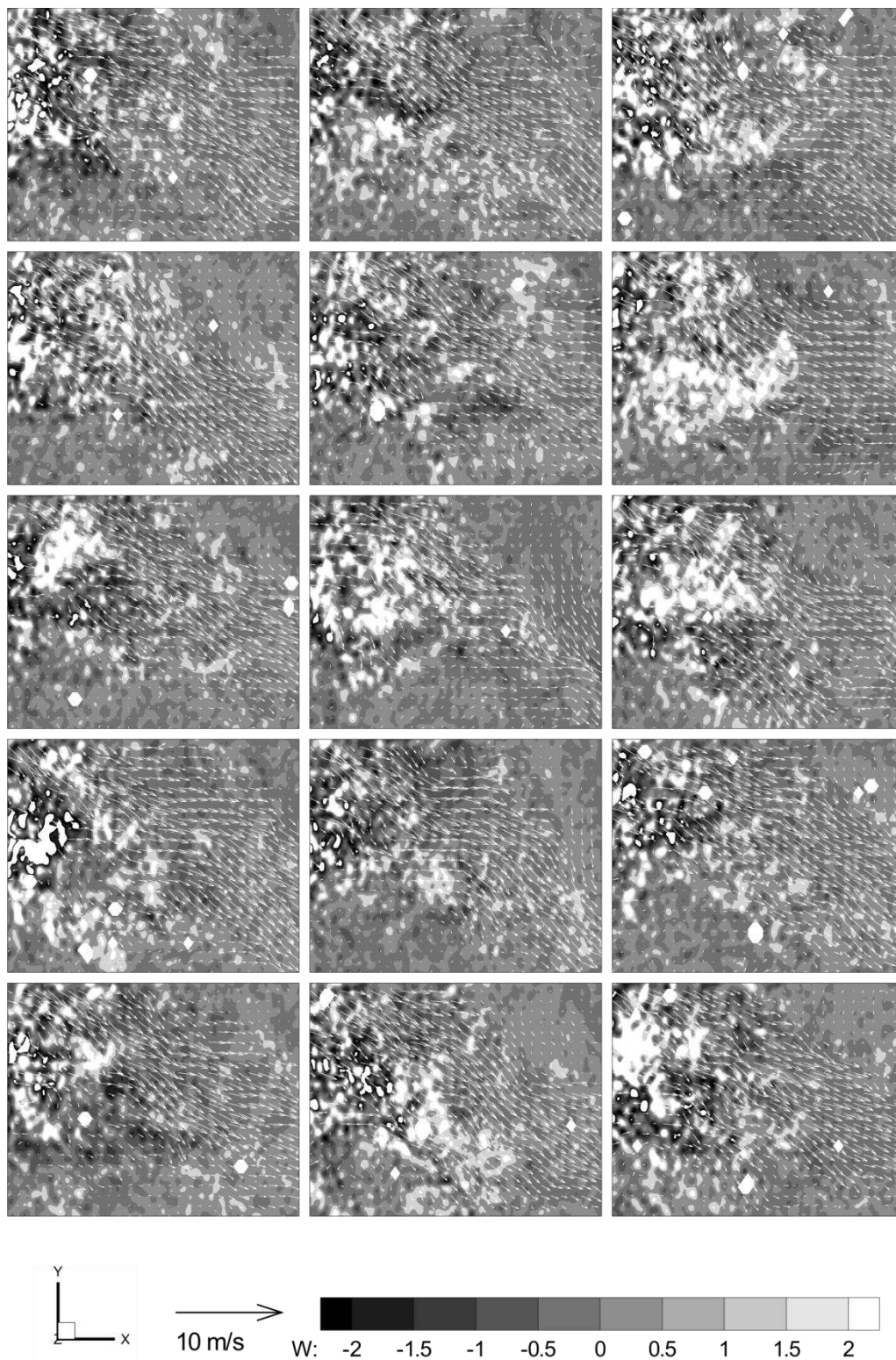
Figure 3.78 The instantaneous SPIV results at investigation plane 7 of a skewed CFF used SAC.
