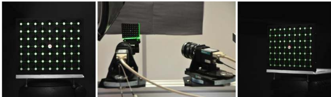
Figure 2.20 Images of the calibration target with both cameras.
