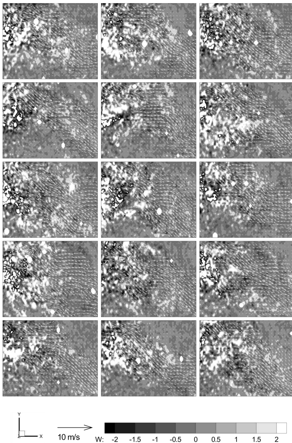
Figure 3.81 The instantaneous SPIV results at investigation plane 7 of a skewed CFF used SAC.
