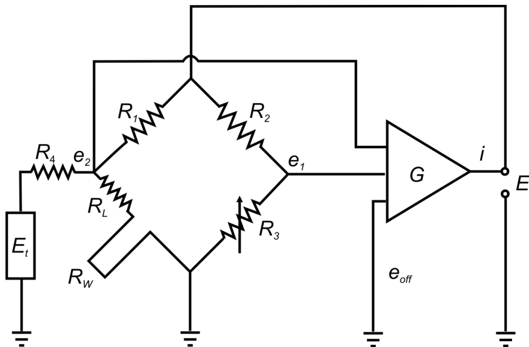
Figure 2.4 The Wheatstone bridge schematics.
