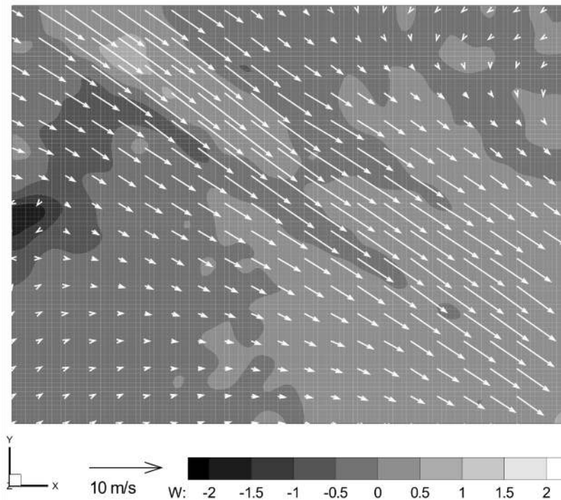
Figure 3.15 Average three dimensional velocity distribution of the skewed CFF used SAC on investigation plane 4.
