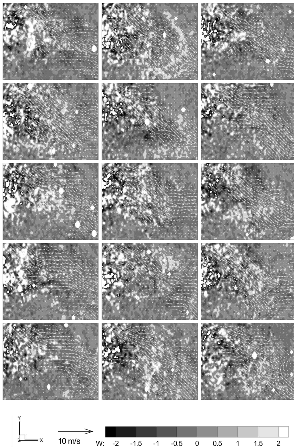
Figure 3.79 The instantaneous SPIV results at investigation plane 7 of a skewed CFF used SAC.
