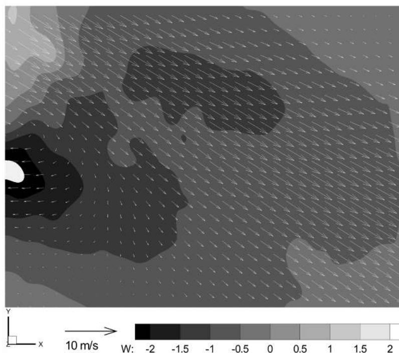
Figure 3.58 Average three dimensional velocity distribution of the straight CFF used SAC on investigation plane 6.
