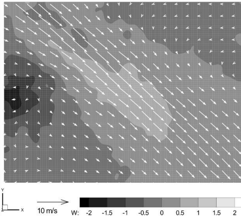
Figure 3.9 Average three dimensional velocity distribution of the skewed CFF used SAC on investigation plane 2.
