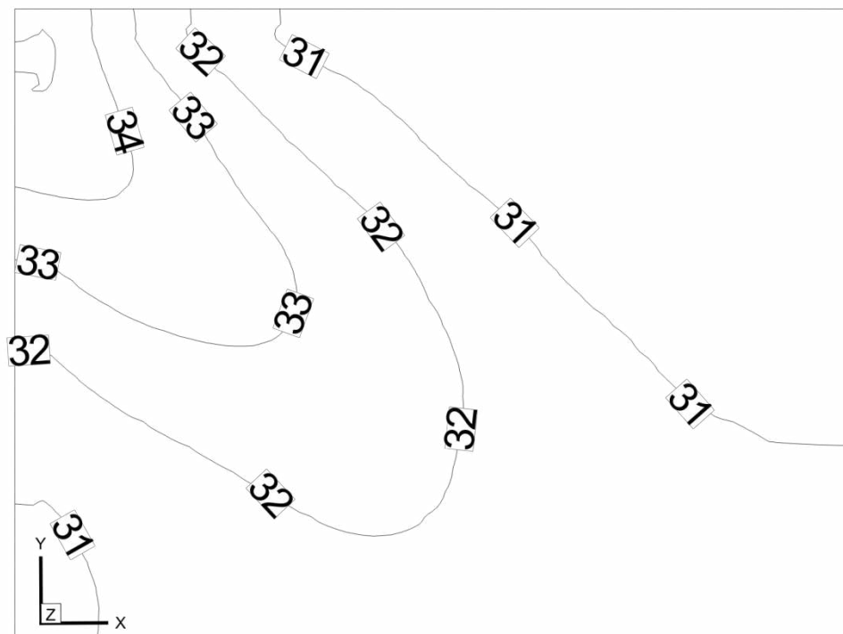
Figure 3.97 Temperature distribution on investigation plane 2.
