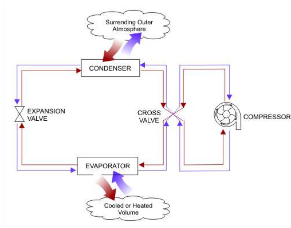
Figure 1.1 Schematic of the SAC.
