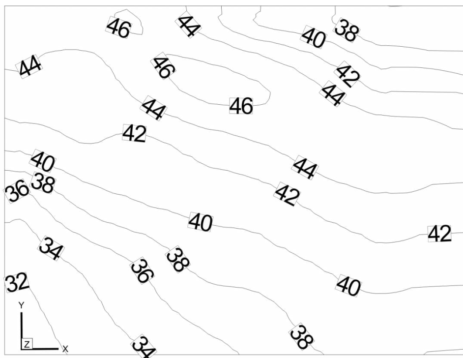
Figure 3.101 Temperature distribution on investigation plane 6.
