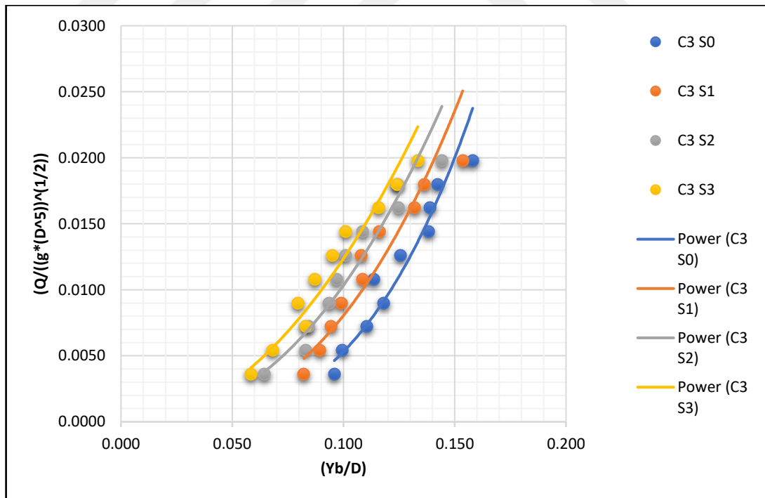
Figure 5.21 The Change of \left(\frac{Q}{\sqrt{g D^5}}\right) with \left(\frac{Y_b}{D}\right) For Rough Bottom Channels (C 3 ) with Different Slopes
