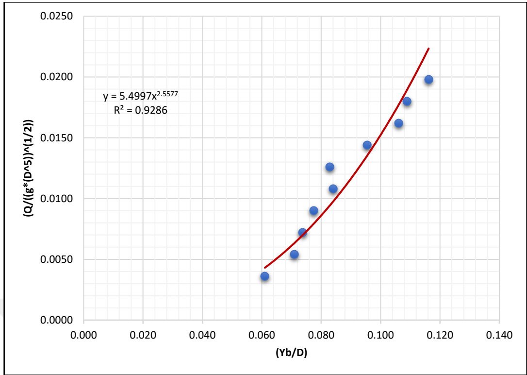
Figure 5.14 The Change of \left(\frac{Q}{\sqrt{g D^5}}\right) with \left(\frac{Y_b}{D}\right) For Rough Bottom Channels ( C_2 ) with Slope ( S_2 = 0.01 )
