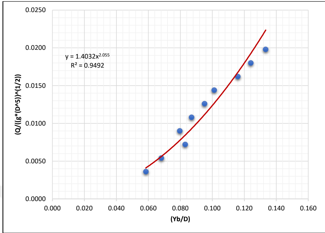
Figure 5.20 The Change of \left(\frac{Q}{\sqrt{g D^5}}\right) with \left(\frac{Y_b}{D}\right) For Rough Bottom Channels (C 3 ) with Slope ( S_3 = 0.015 )
