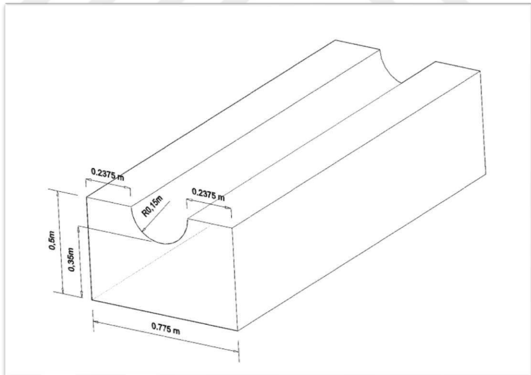
Figure 4.9 (b) Semicircular Channel (3D)
