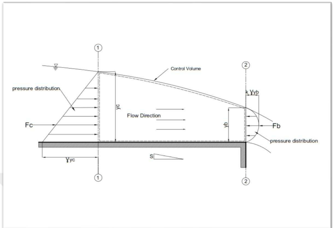
Figure 3.1 Theoretical Control Volume
