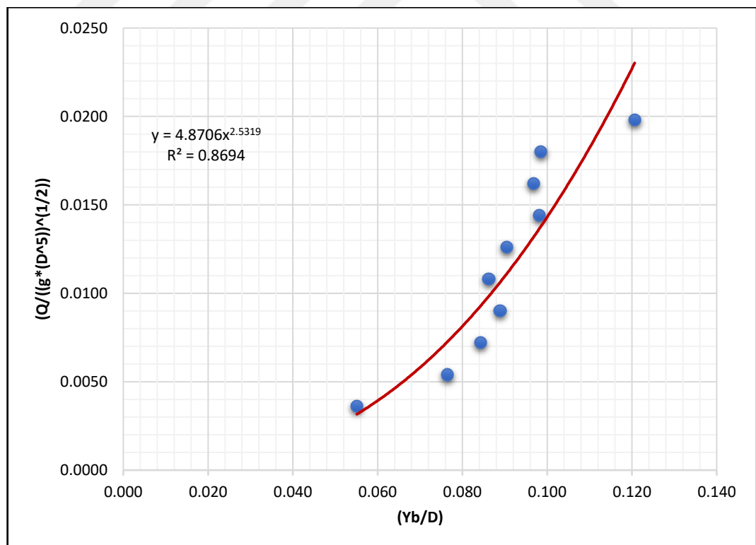
Figure 5.9 The Change of (\frac{Q}{\sqrt{g D^5}}) with (\frac{Yb}{D}) For Rough Bottom Channels ( C_1 ) with Slope ( S_2 = 0.01 )
