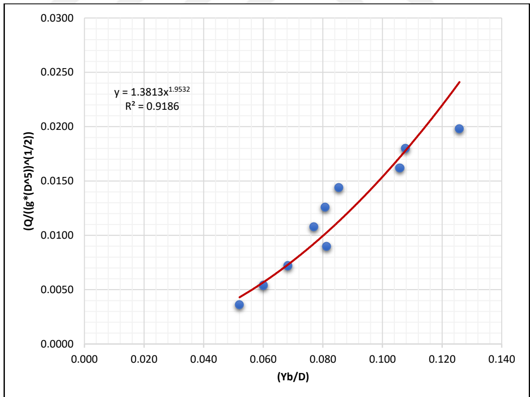
Figure 5.15 The Change of \left(\frac{Q}{\sqrt{g D^5}}\right) with \left(\frac{Y_b}{D}\right) For Rough Bottom Channels ( C_2 ) with Slope ( S_3 = 0.015 )
