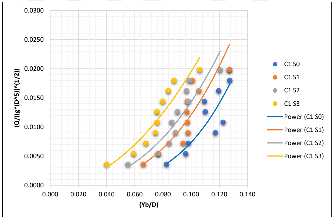
Figure 5.11 The Change of \left(\frac{Q}{\sqrt{g D^5}}\right) with \left(\frac{y_b}{D}\right) For Rough Bottom Channels (C 1 ) with Different Slopes
