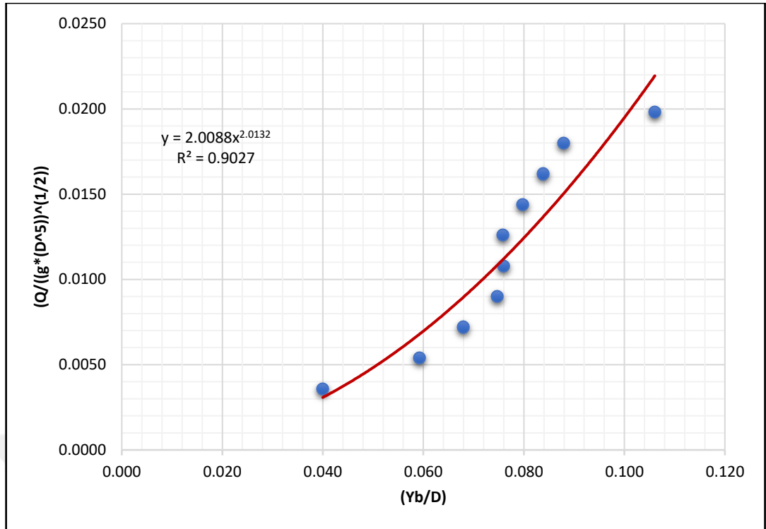
Figure 5.10 The Change of \left(\frac{Q}{\sqrt{g D^5}}\right) with \left(\frac{y_b}{D}\right) For Rough Bottom Channels (C 1 ) with Slope ( S_3 = 0.015 )
