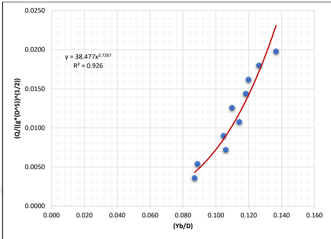
Figure 5.12 The Change of (\frac{Q}{\sqrt{g D^5}}) with (\frac{Y_b}{D}) For Rough Bottom Channels (C 2 ) with Slope ( S_0 = 0 )
