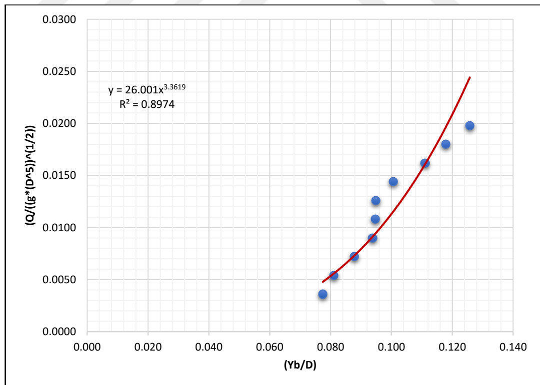
Figure 5.13 The Change of (\frac{Q}{\sqrt{g D^5}}) with (\frac{Y_b}{D}) For Rough Bottom Channels (C 2 ) with Slope ( S_1 = 0.005 )
