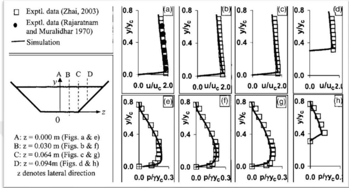
Figure 2.6 Velocity and pressure distribution at brink with y/y_c
