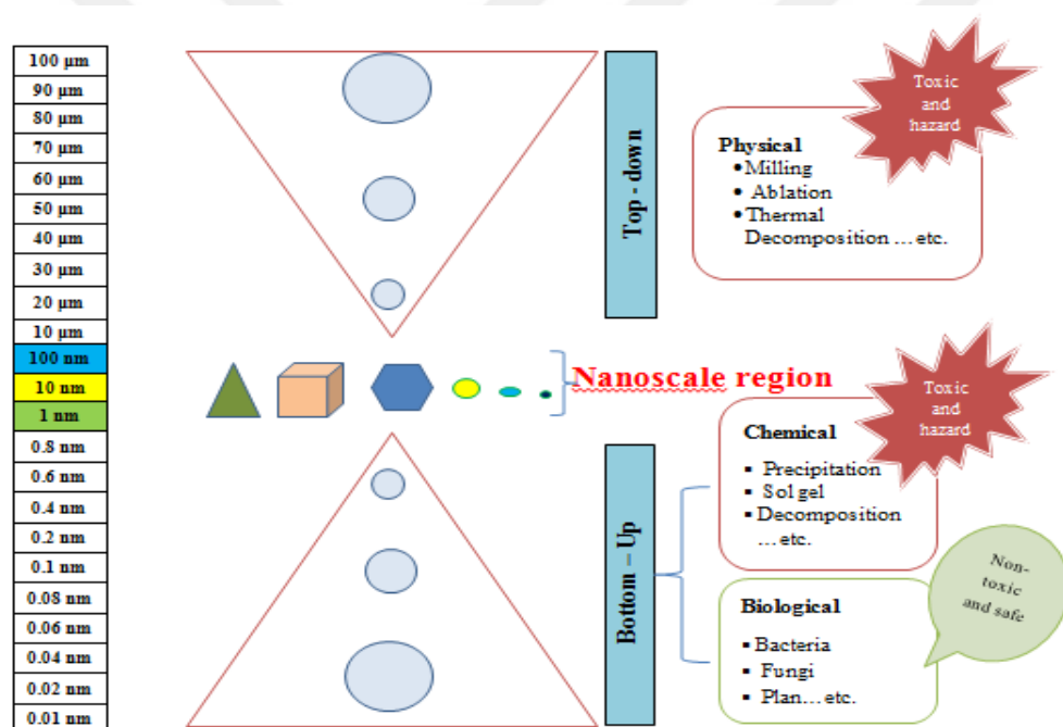
Figure 2.1. Top-down and bottom-up approaches for synthesis inorganic nanoparticles, this figure deduced by Azharuddin et al. (2019).
