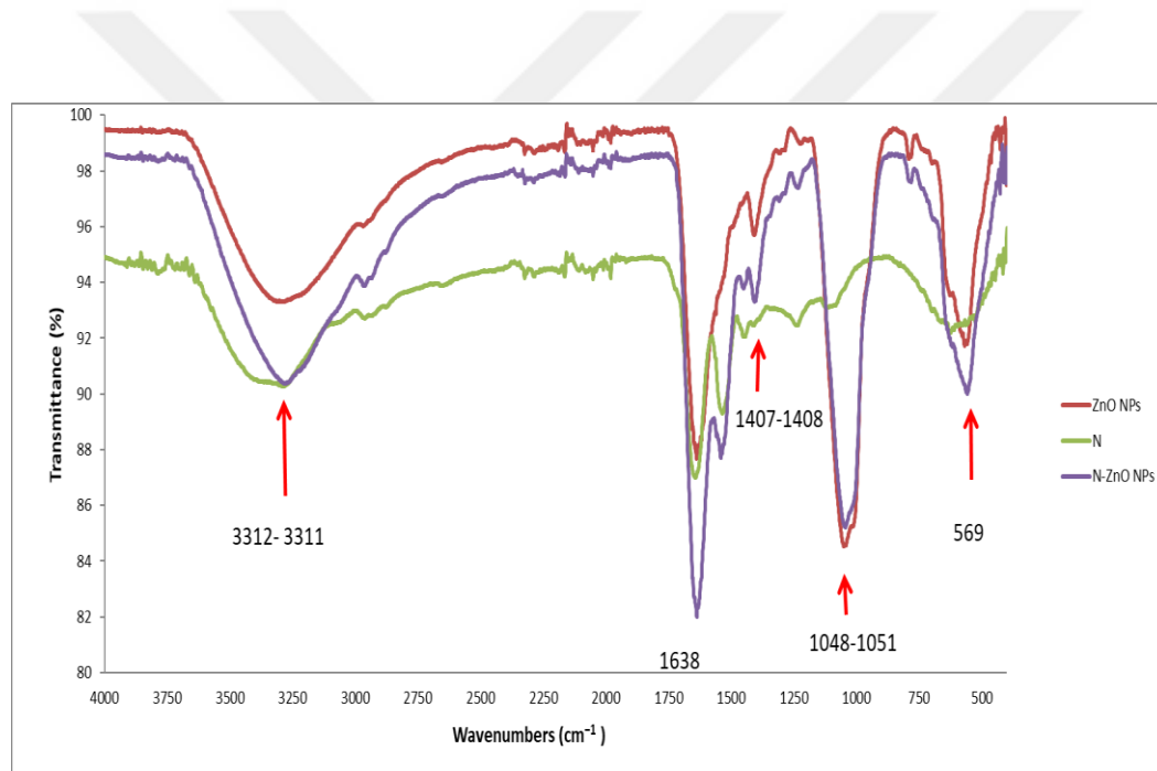
Figure 4.15. The Fourier transforms infrared (FTIR) spectroscopy measurement of ZnO NPs, nisin and N-ZnO NPs.
