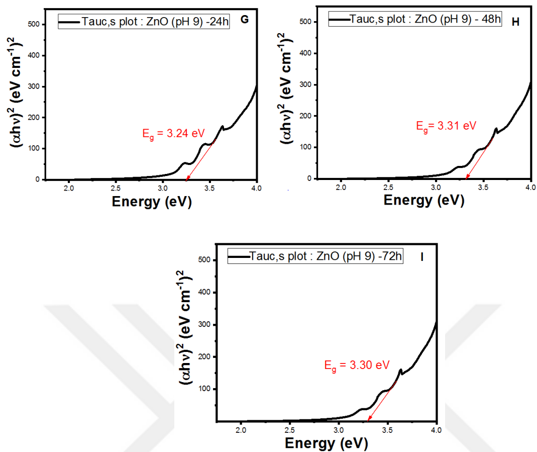
Figure B. Effect pH values on energy bandgap of ZnO NPs at different times.
