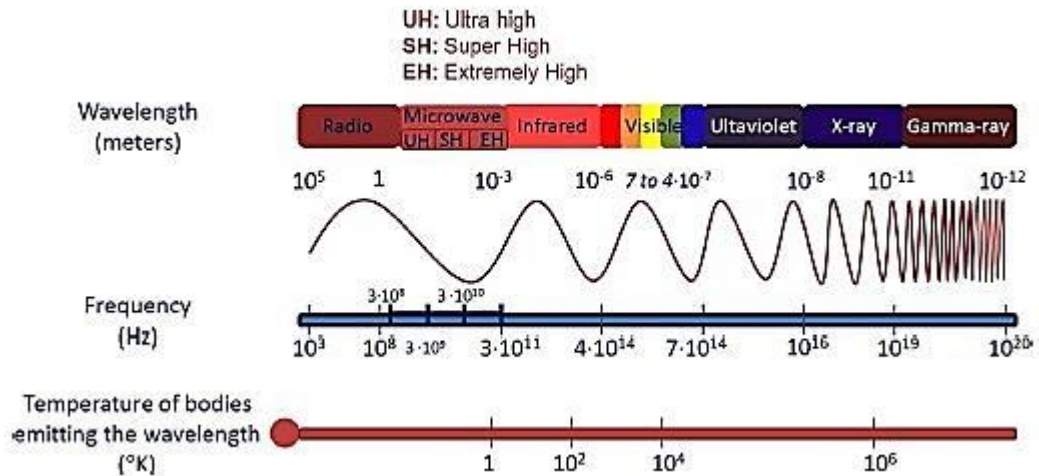
Figure 2.9 Electromagnetic Spectrum
