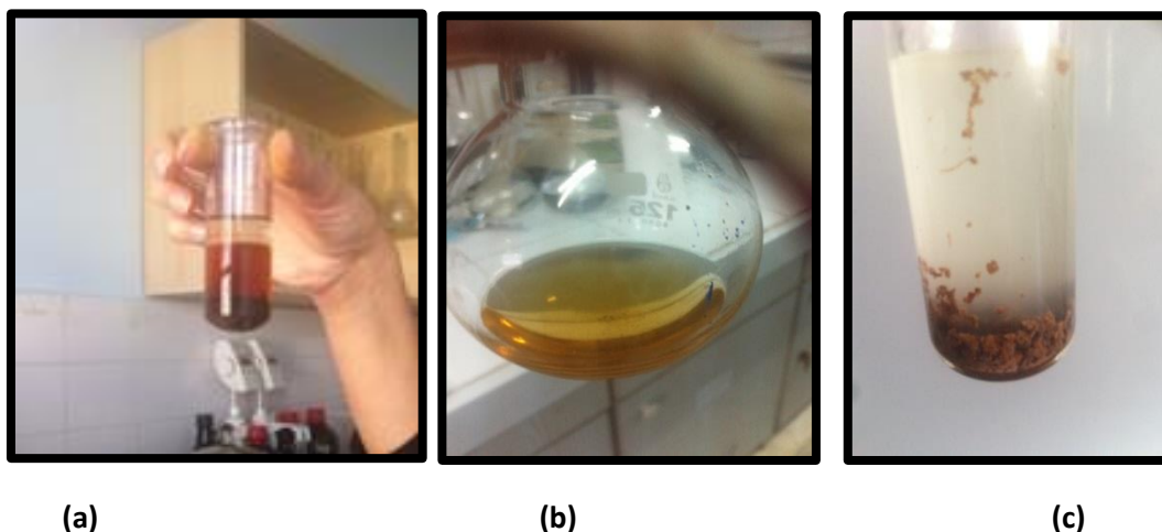
Figure 4.1 Olive pomace after (a) Microwave Assisted Extraction (Polar Solvent) (b) Centrifugation (Polar Solvent) (c) Microwave Assisted Extraction (Non-polar Solvent)
