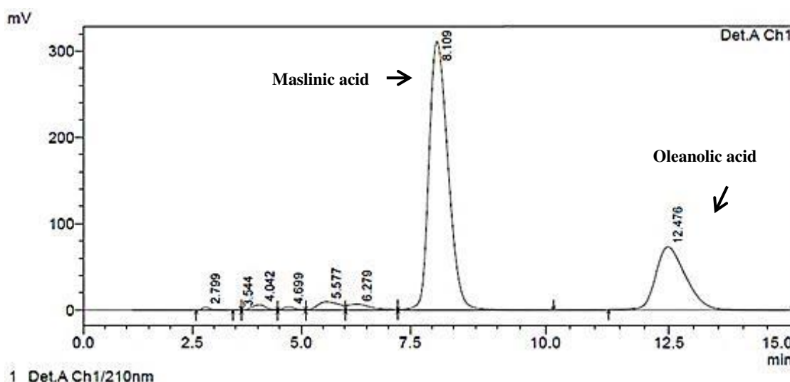
Figure 4.4 HPLC chromatogram at 210 nm of maslinic acid and oleanolic acid after microwave assisted extraction by using hexane
