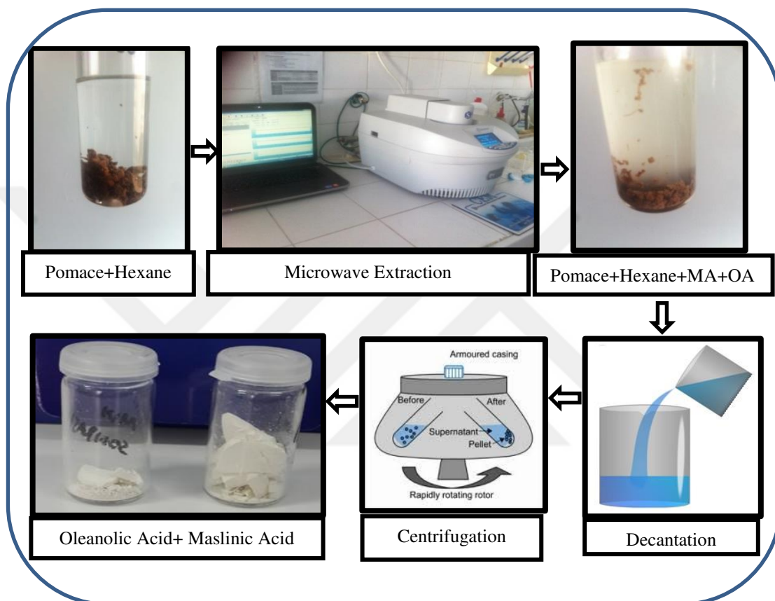
Figure 3.1 Shematic representation of extraction of MA and OA by using microwave assisted extraction
