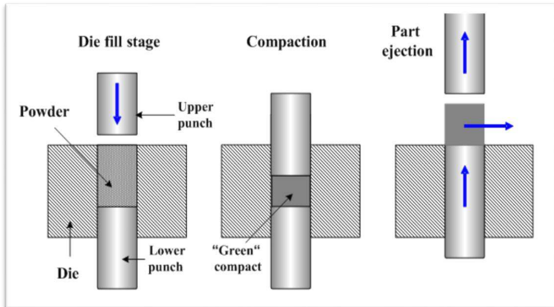
Figure 3.8. Compression process
