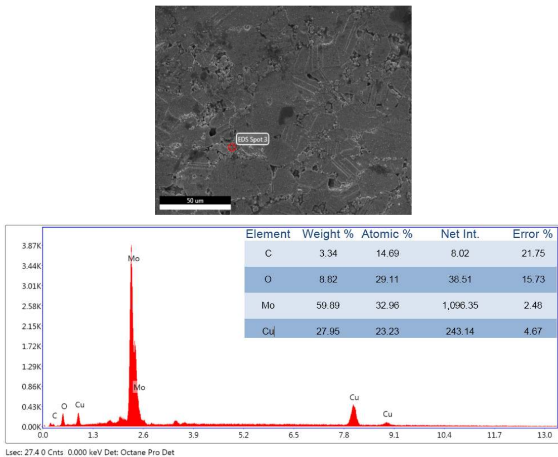
Graph 8.4. EDS analysis of the reinforcement in Mo 2 C reinforced bronze matrix FGM composite
