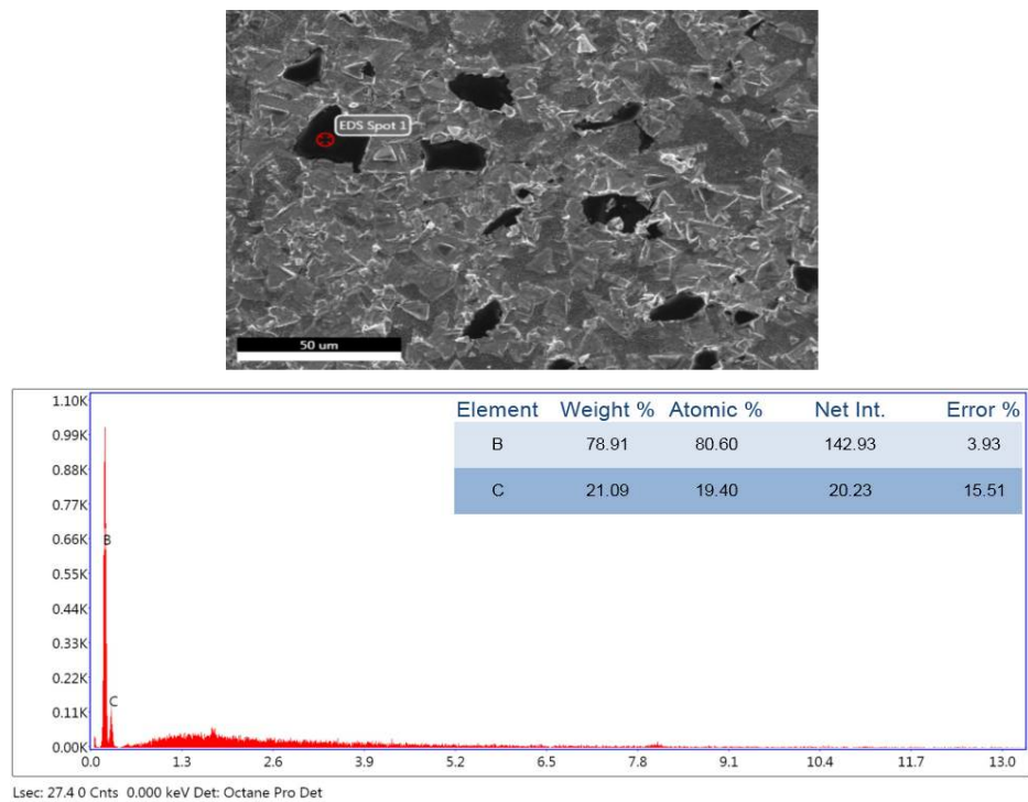
Graph 8.2. EDS analysis of the reinforcement in B 4 C reinforced bronze matrix FGM composite
