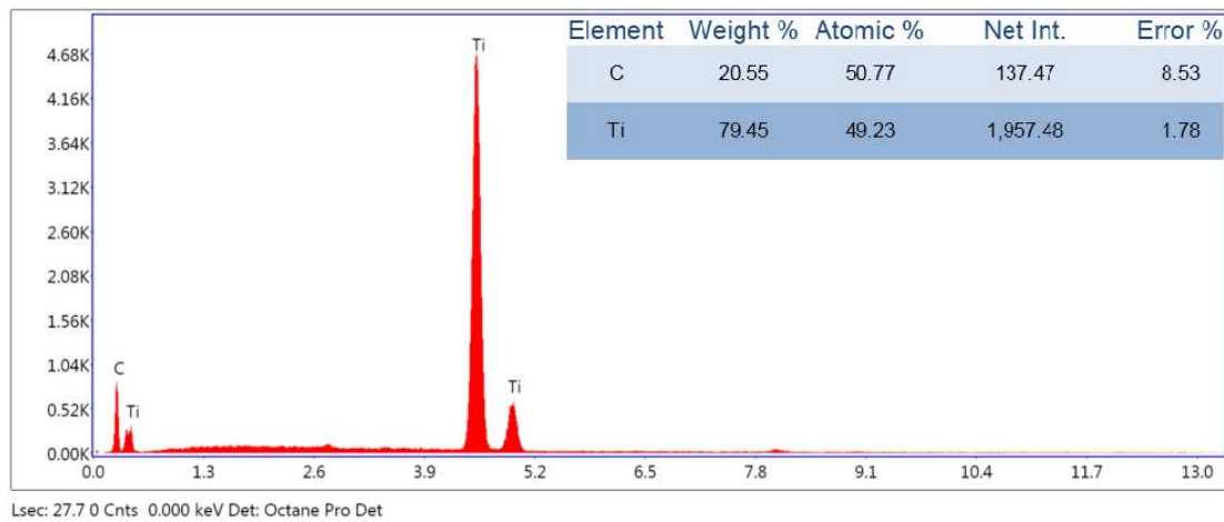
Graph 8.6. EDS analysis of the reinforcement in TiC reinforced bronze matrix FGM composite
