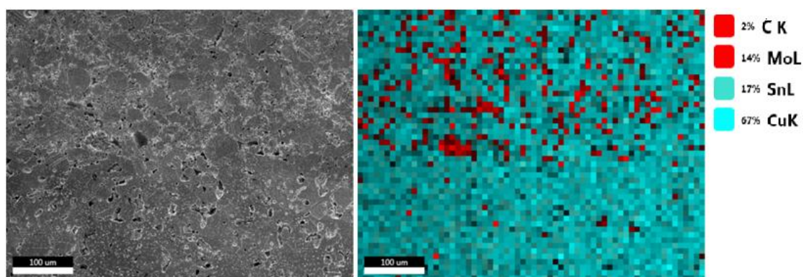
Photo 8.11. EDS analysis of \text{Mo}_2\text{C} reinforced bronze matrix FGM composite
