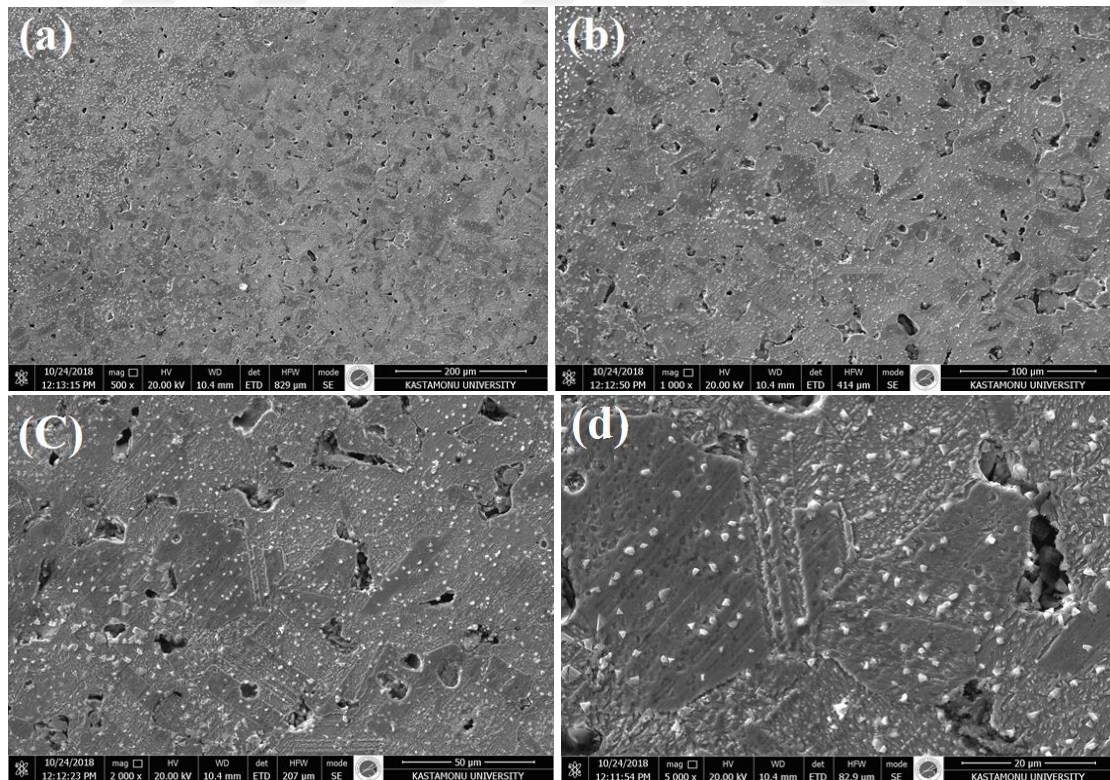
Photo 8.4. SEM images of \text{TiC} reinforcement bronze matrix FGM: (a) 500X, (b) 1000X, (c) 2000X, and (D) 5000X
