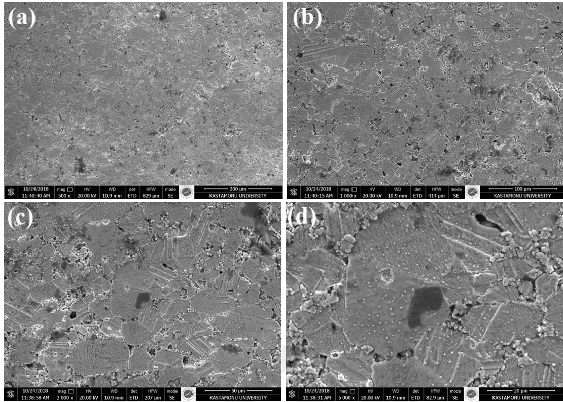
Photo 8.3. SEM images of \text{Mo}_2\text{C} reinforcement bronze matrix FGM: (a) 500X, (b) 1000X, (c) 2000X, and (D) 5000X
