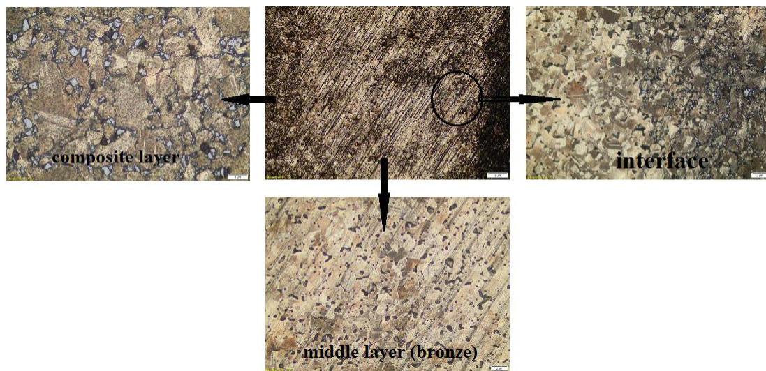
Photo 8.8. Optical microscope images of TiC reinforced bronze matrix FGM composite
