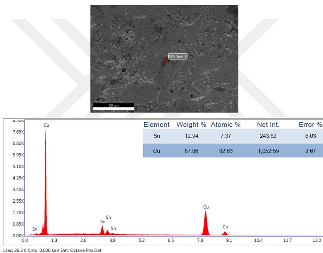
Graph 8.3. EDS analysis of the matrix in \text{Mo}_2\text{C} reinforced bronze matrix FGM composite
