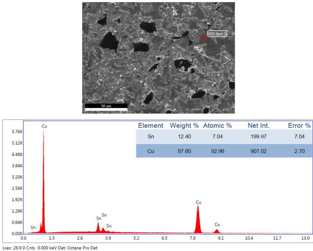
Graph 8.1. EDS analysis of the matrix in B 4 C reinforced bronze matrix FGM composite
