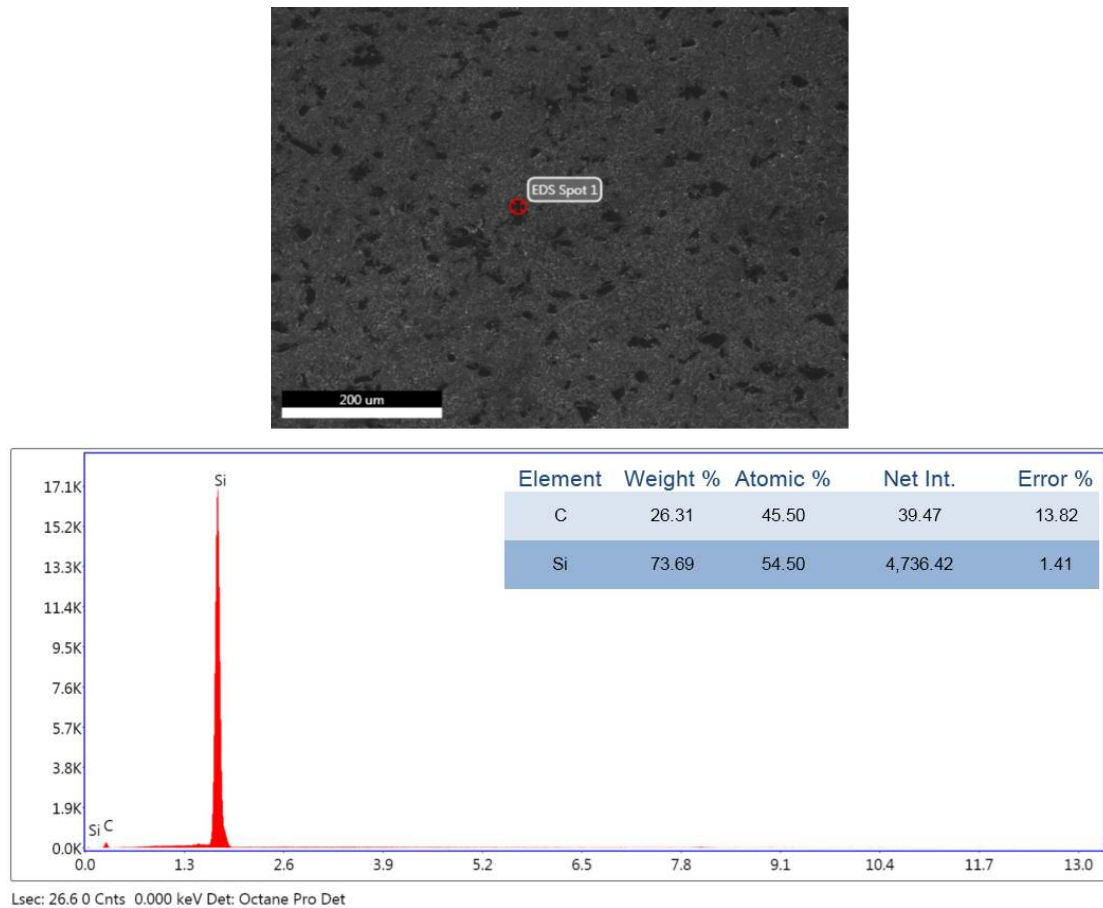
Graph 8.8. EDS analysis of the reinforcement in SiC reinforced bronze matrix FGM composite
