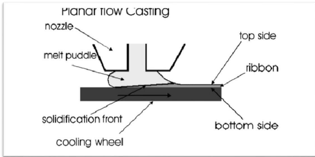
Figure 3.4. Ribbon casting process
