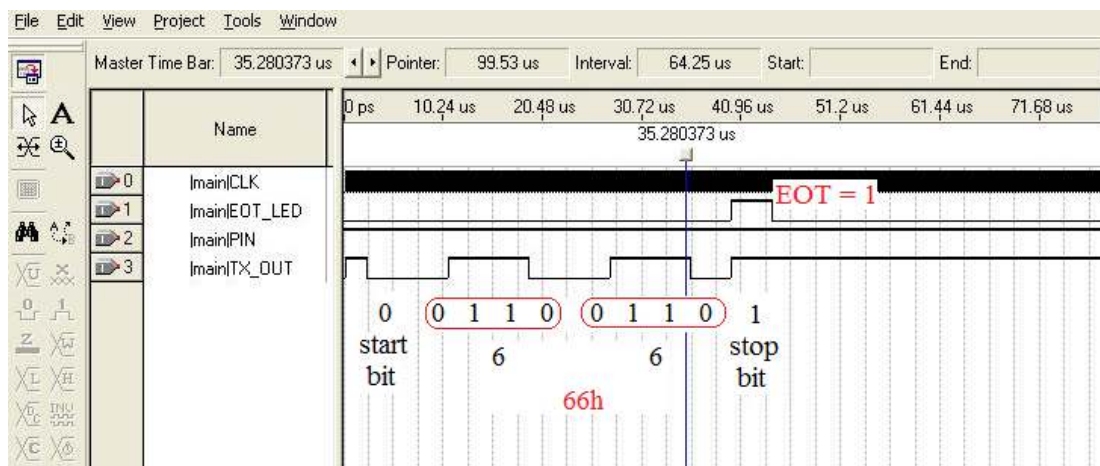
Figure 5.22 Transmitter simulation when datainput is 66h.
