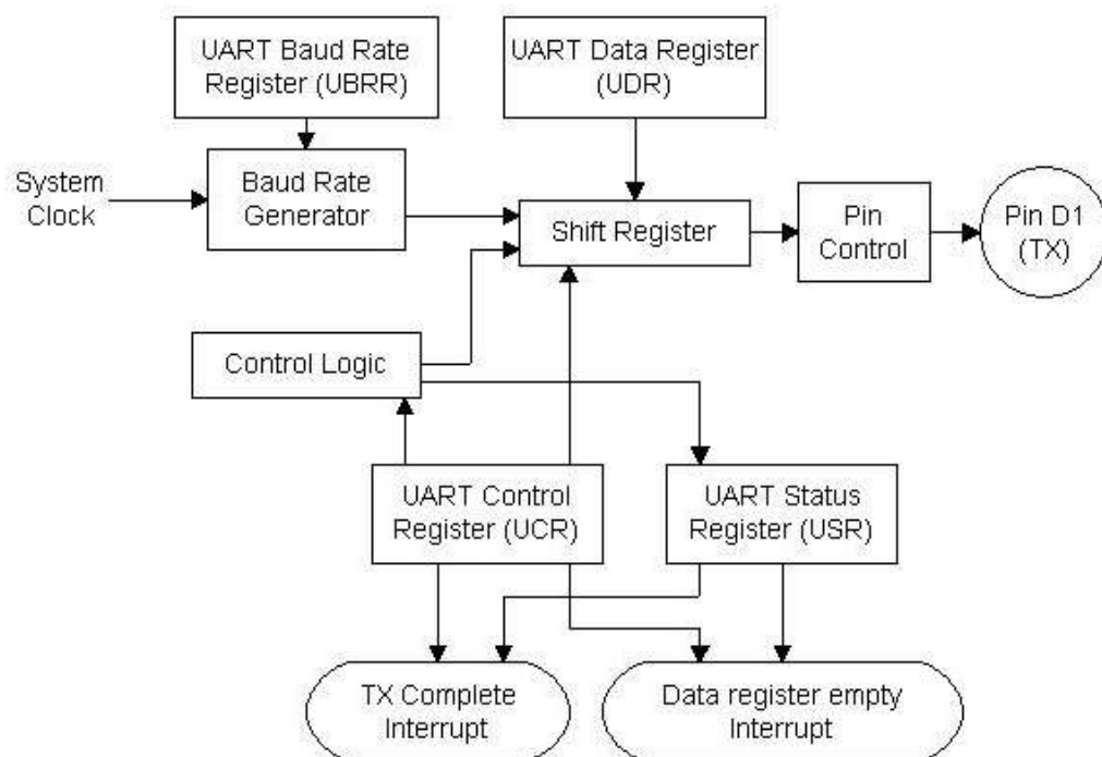
Figure 5.13 Internal structure of UART transmitter (Weinstein, Volz, & Redecker, 2004).
