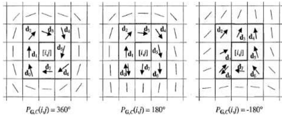
Figure 3.7 Example of computation of the Poincaré index in the 8-neighborhood of points belonging (from the left to the right) to a whorl, loop, and delta singularity, respectively.
