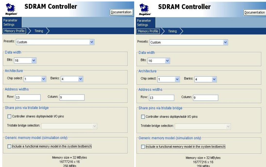
Figure 5.34 SDRAM controllers, sdram_0 and sdram_1 , configurations.
