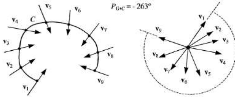
Figure 3.6 The Poincarè index computed over a curve C immersed in vector field G (Maltoni, Maio, Jain, & Prabhakar, 2003).
