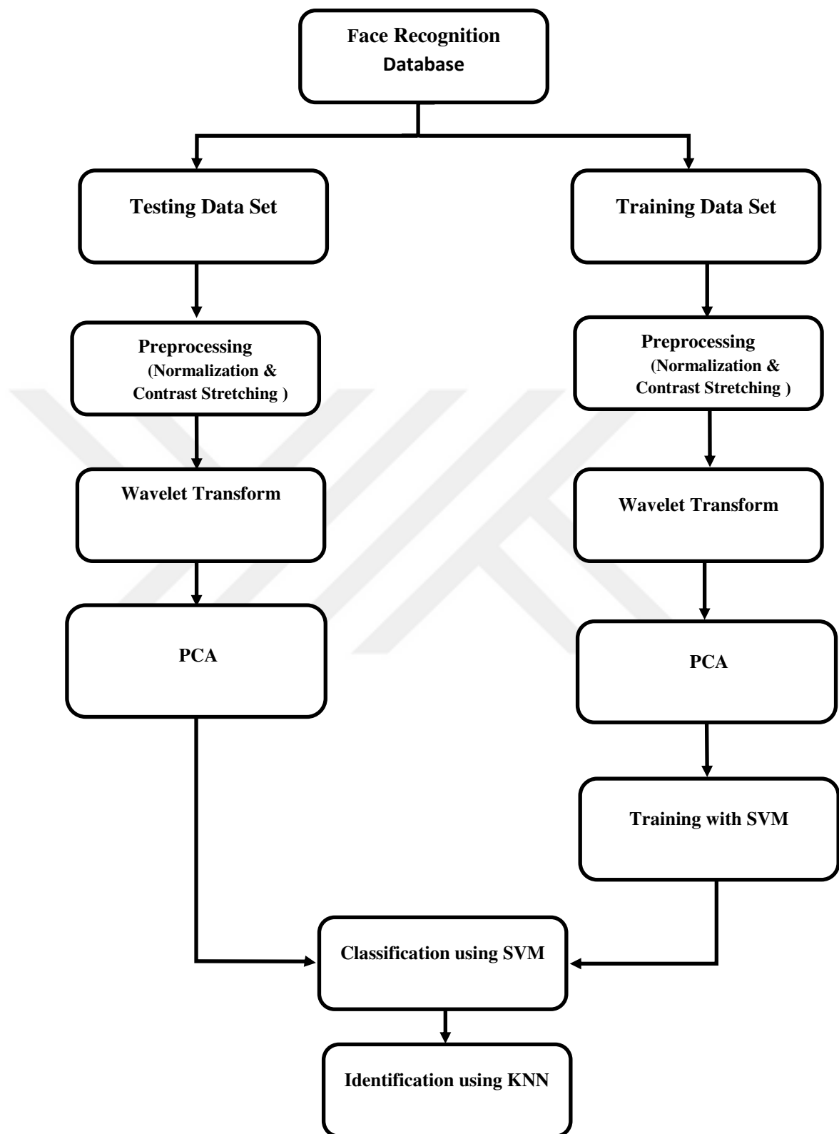
Figure (4-2): The structure of a proposed system
