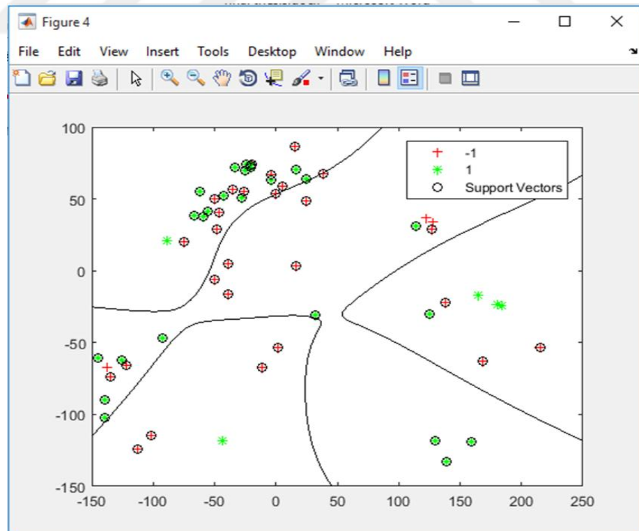
Figure (4-9): Multilayer Perceptron kernel in YALE database
