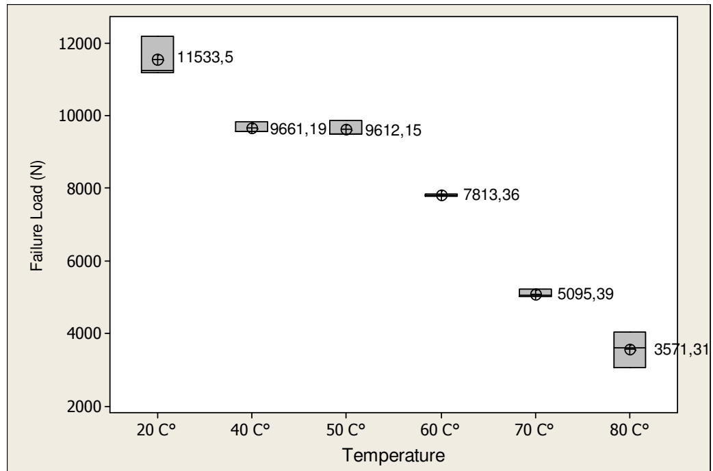
Figure 7.10 Box plots of failure loads, occurring at different temperatures under M= 6 Nm
