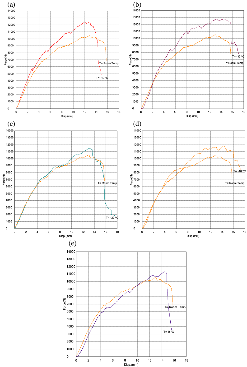
Figure 8.3 The effect of temperature on load/displacement curves in tensile tests of bolted glass fiber / epoxy composite joint under M = 0 Nm tightening torque. Curves of (a) -40^\circ\text{C} (b) -30^\circ\text{C} , (c) -20^\circ\text{C} , (d) -10^\circ\text{C} (e) 0^\circ\text{C} in comparison with that obtained at \sim 20^\circ\text{C} (room temperature)
