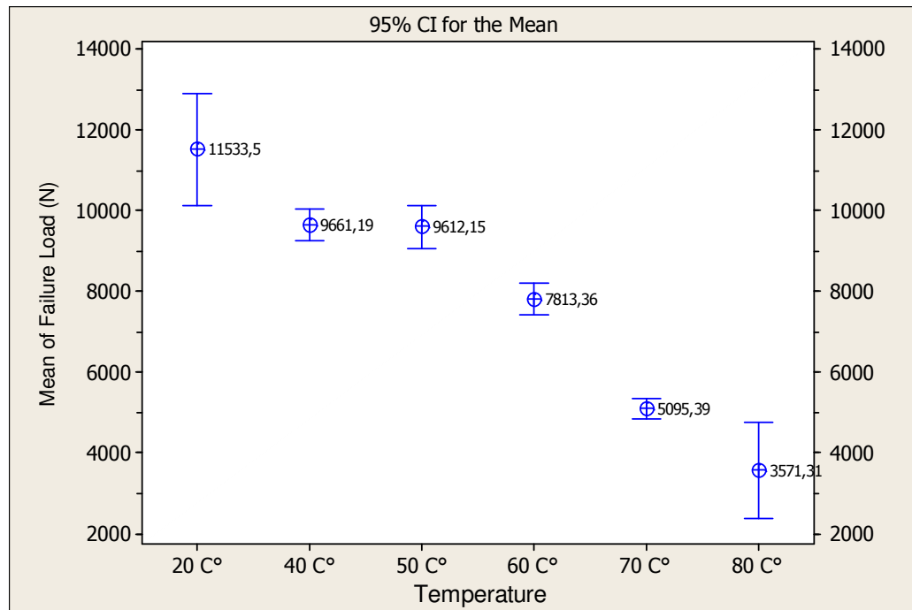
Figure 7.11 Confidence interval (CI) plots for mean values of failure loads, occurring at different temperatures under M= 6 Nm
