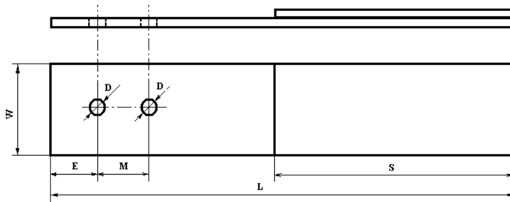
Figure 7.1 Composite specimen geometry for single lap double fastener bearing test
