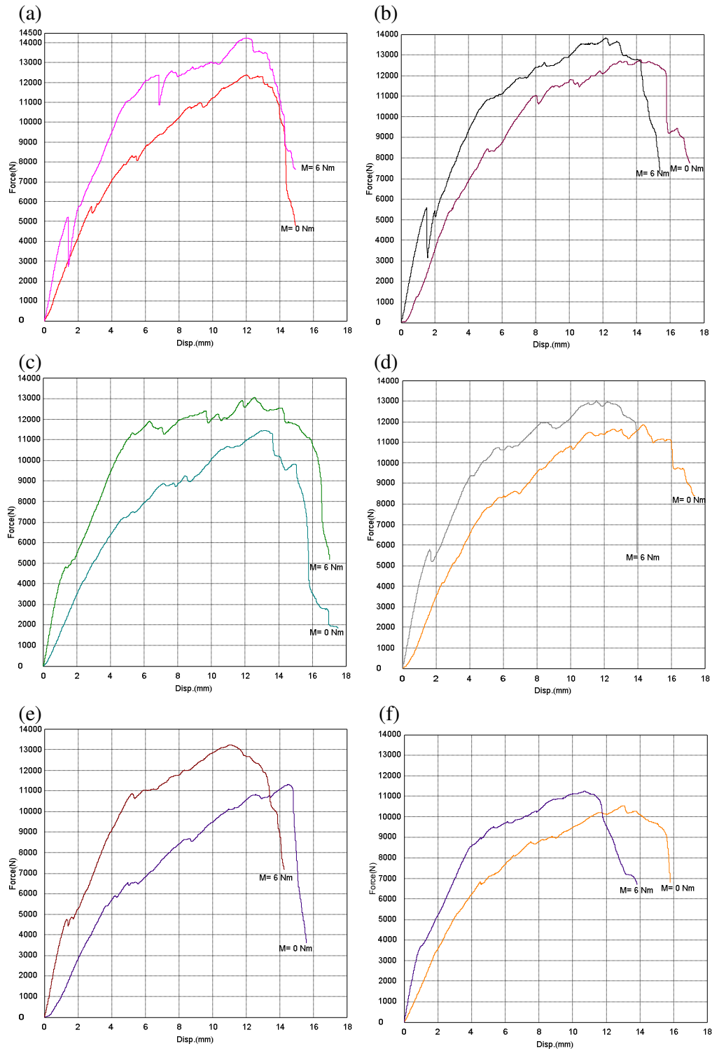
Figure 8.5 The effect of bolt tightening torques on load/displacement curves in tensile tests of bolted glass fiber / epoxy composite joint (a)-40°C, (b) -30 °C, (c) -20 °C, (d) -10 °C,(e) 0 °C (f) ~20°C (room temperature)
