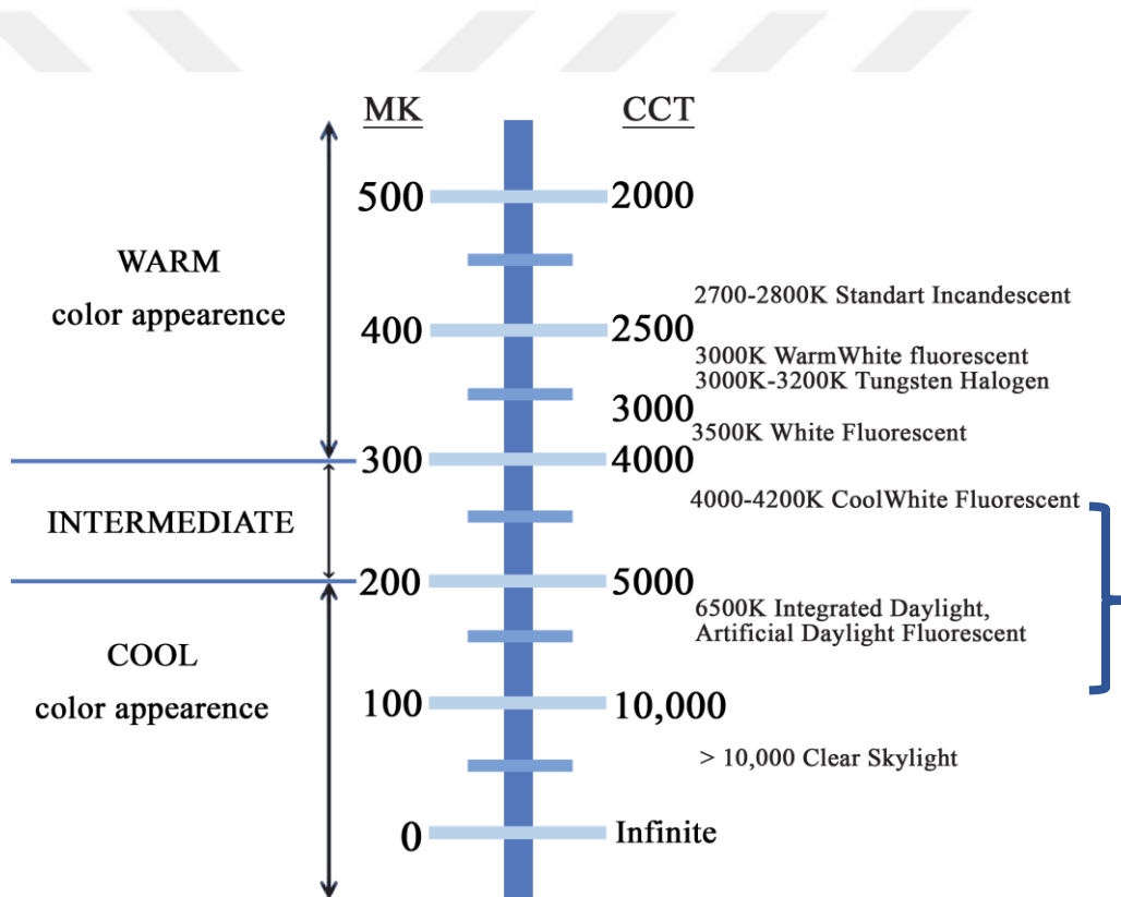
Figure 12: Color temperatures and familiar light sources from CIBSE (Boyce et al., 1989).
