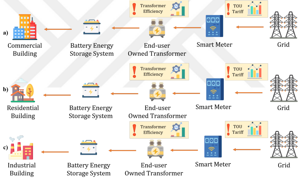
Figure 21: Time-of-Use & Transformer Loss Oriented Battery Installation General Structure: a) Commercial, b) Residential and c) Industrial
