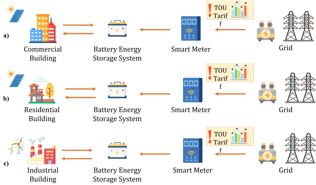
Figure 28: Without Contract for Power Sell Oriented Battery Installation General Structure: a) Commercial, b) Residential and c) Industrial
