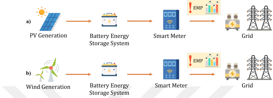
Figure 26: Electricity Market Participating Oriented Battery Installation General Structure: a) PV Generation and b) Wind Generation
