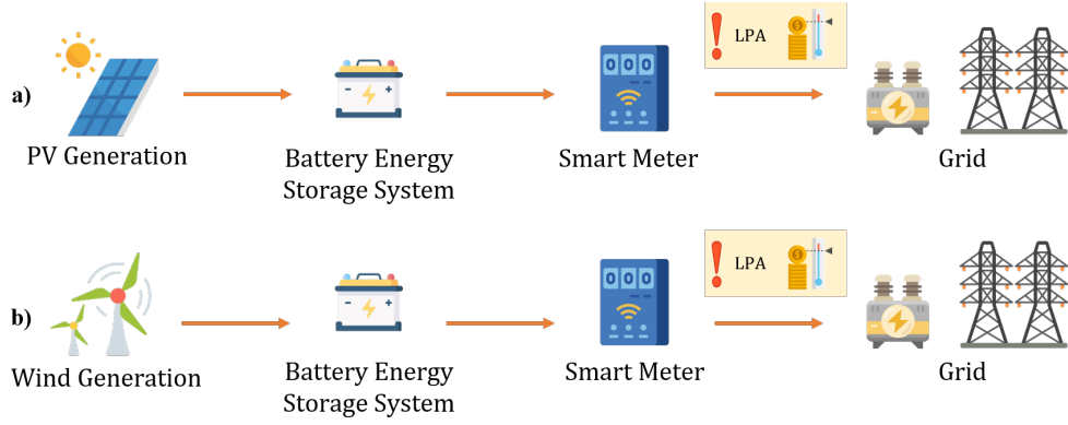
Figure 24: Limited Purchase Agreement Oriented Battery Installation General Structure: a) PV Generation and b) Wind Generation
