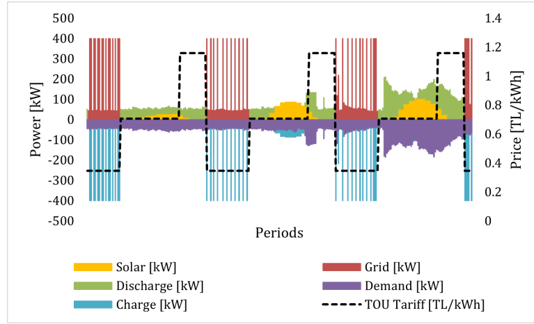
Figure 29: Without Power Selling Prosumer Power Balance.
