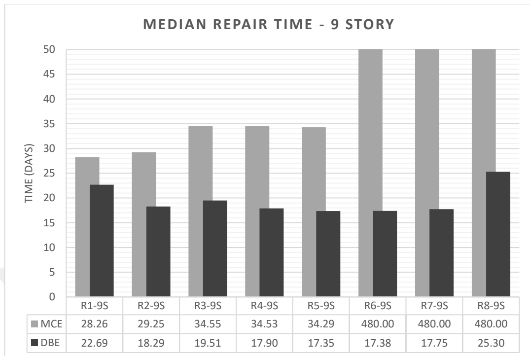
Figure 4.17. Median repair time values for 9-Story archetypes
