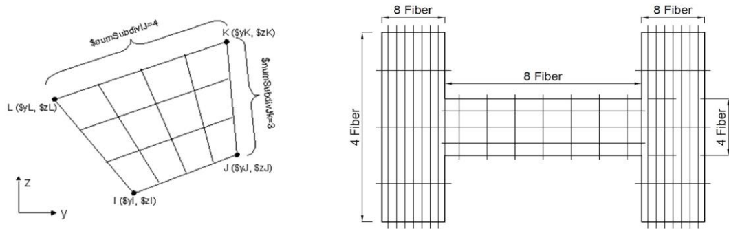
Figure 3.7. Fiber section definition and column section fiber representation
