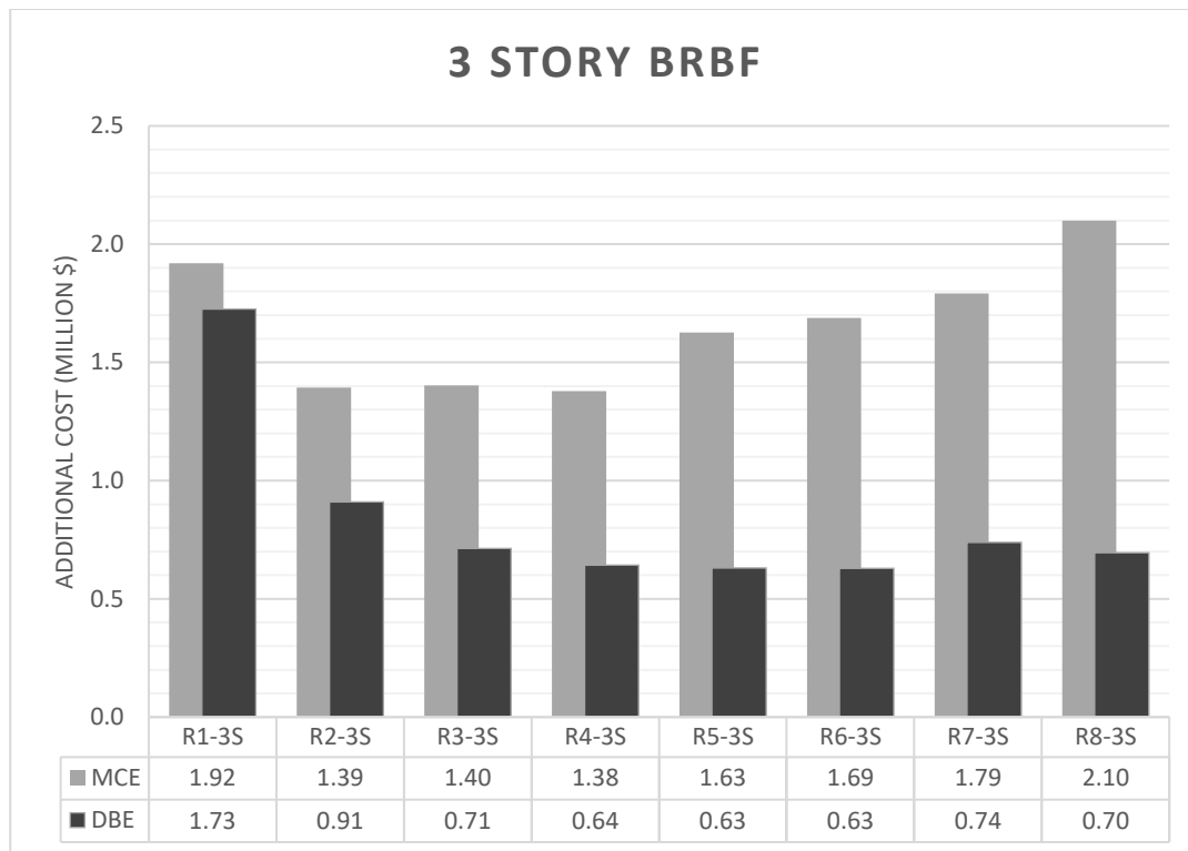
Figure 5.1. Additional Cost Analysis of 3 Story BRBF Archetypes
