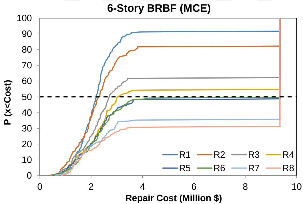
Figure 4.5. The repair cost non-exceedance probabilistic distribution (6-Story)
