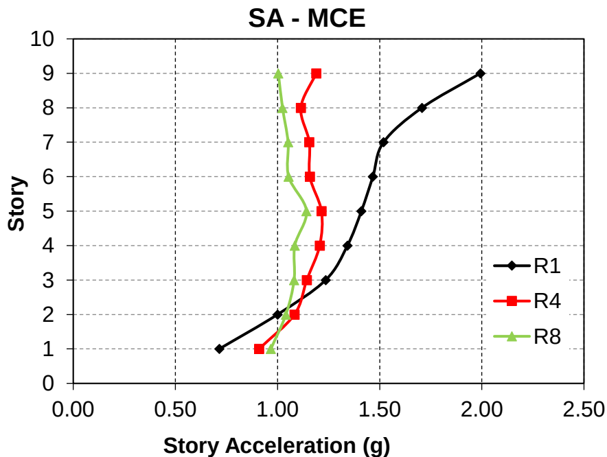
Figure 3.21. Story Acceleration response of 9-story Archetypes - MCE
