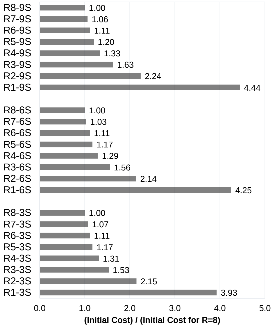
Figure 2.8. Initial cost of SFRSs in terms of initial cost of R=8 archetypes
