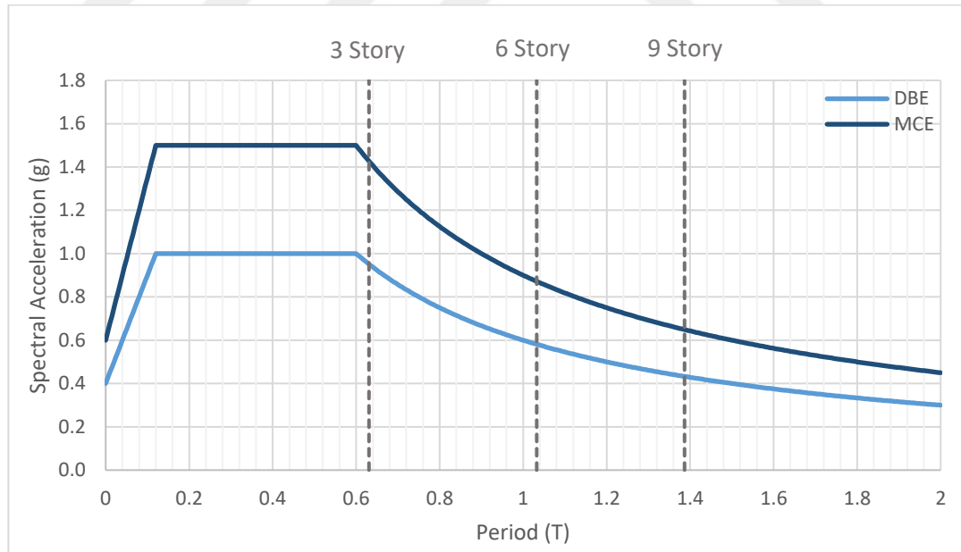
Figure 2.4. DBE and MCE spectrum
