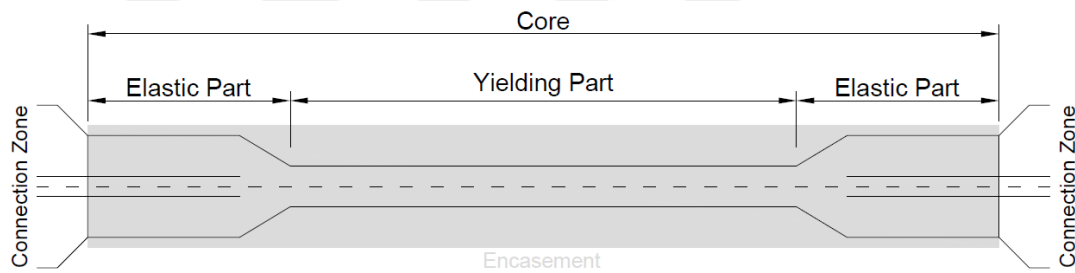
Figure 1.4. Sections of BRBs
