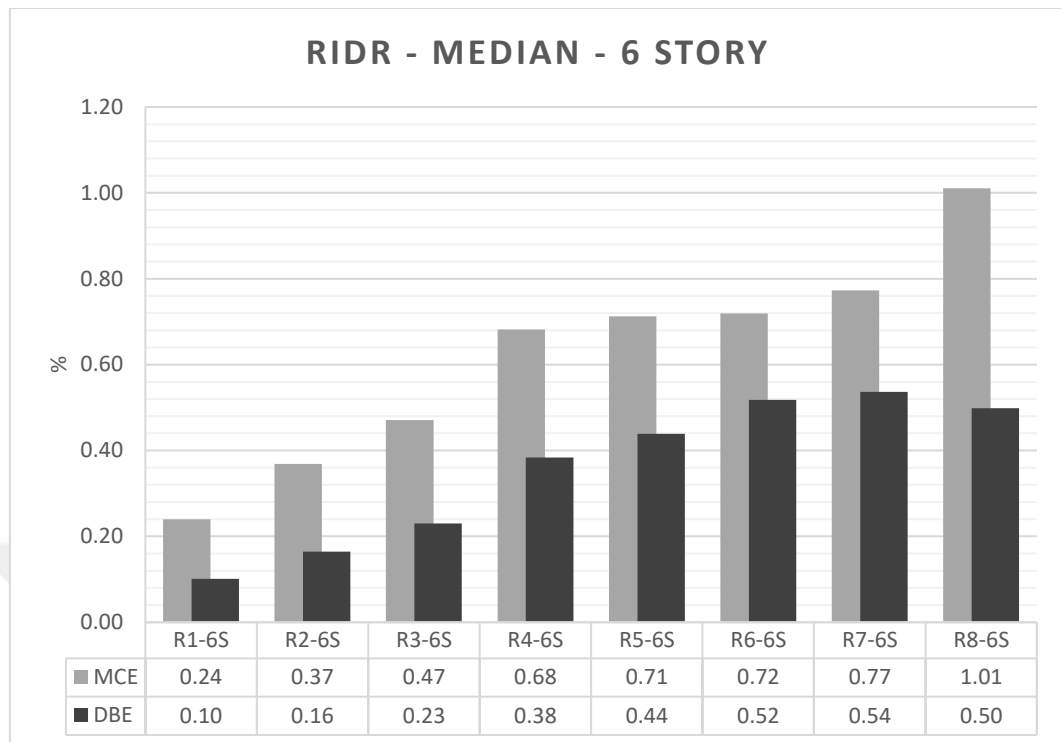
Figure 3.17. R-IDR demands for 6 Story archetypes (Median)
