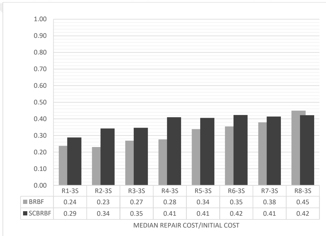
Figure 6.5. Median repair cost comparison of SCBRB and BRB (3-Story)
