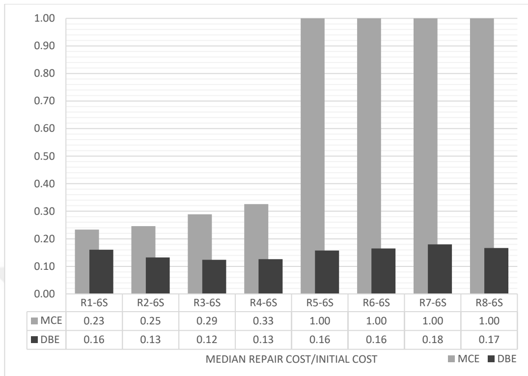
Figure 4.8. Normalized Median repair cost values for 6-Story archetypes
