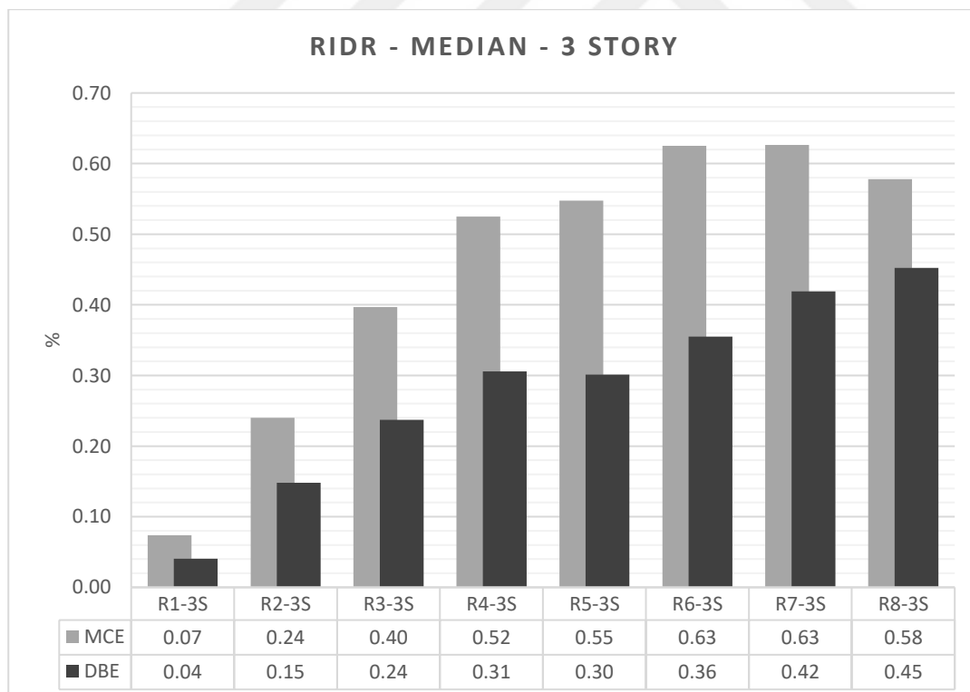
Figure 3.16. R-IDR demands for 3 Story archetypes (Median)
