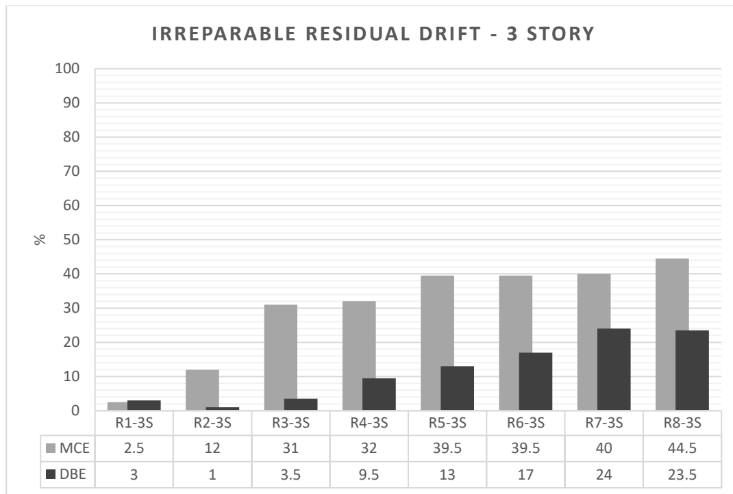
Figure 4.12. Irreparable residual drift probabilities for 3-Story archetypes
