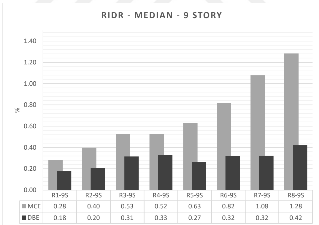
Figure 3.18. R-IDR demands for 9 Story archetypes (Median)
