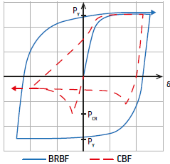
Figure 1.1. Comparison of Hysteretic behaviors (Star Seismic Europe Ltd.)
