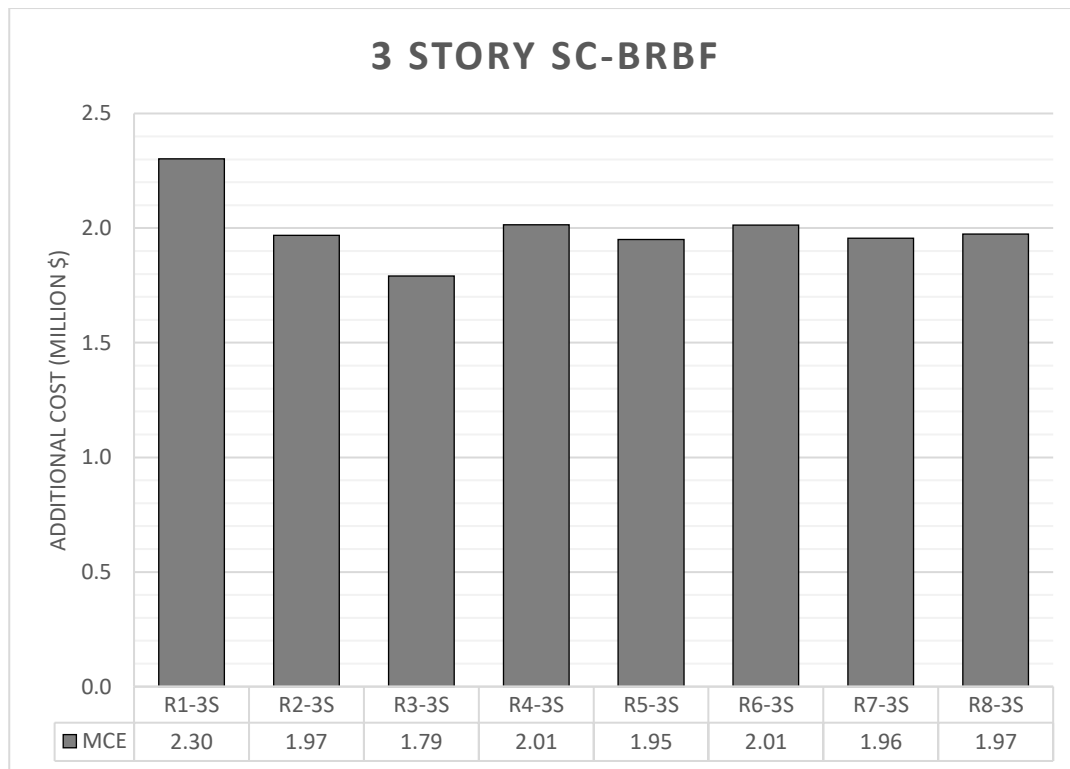
Figure 6.8. Additional Cost Analysis of 3 Story SC-BRBF Archetypes
