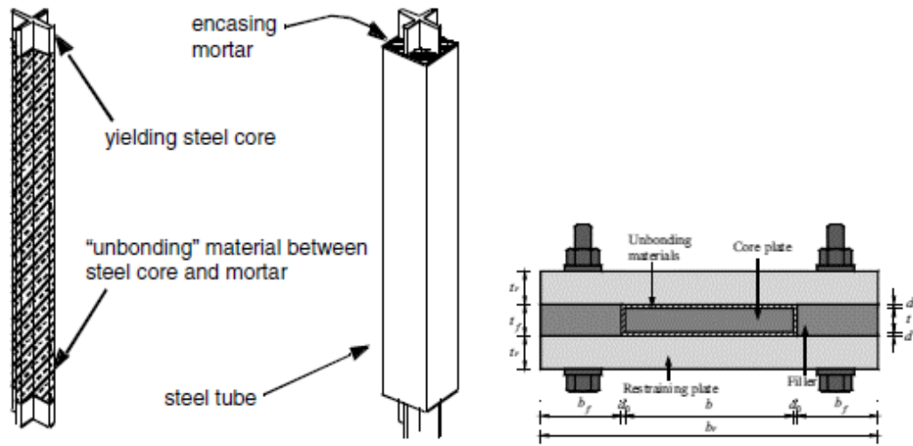
Figure 1.5. Types of BRBs: (a) Mortar Filled BRB, (b) All-Steel BRB
