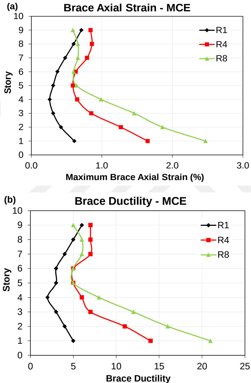
Figure 3.28. Maximum Brace Axial Strain and Ductility for 9-story Archetypes
