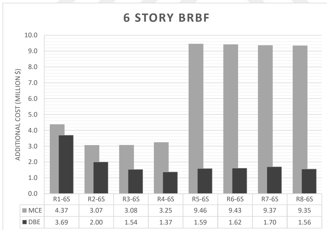
Figure 5.2. Additional Cost Analysis of 6 Story BRBF Archetypes
