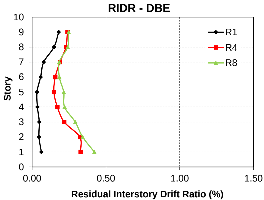
Figure 3.15. RIDR response of 9-story Archetypes - DBE
