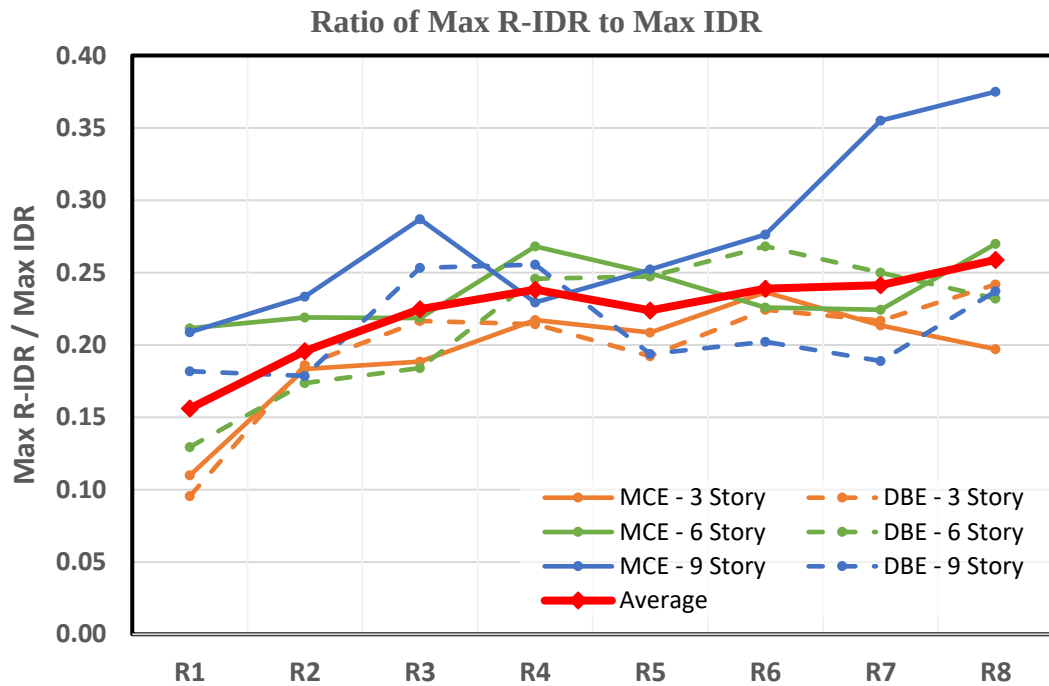
Figure 3.20. Max R-IDR to Max IDR Ratio (Median)
