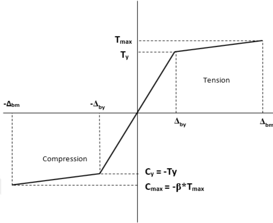
Figure 2.5. BRB strength adjustment
