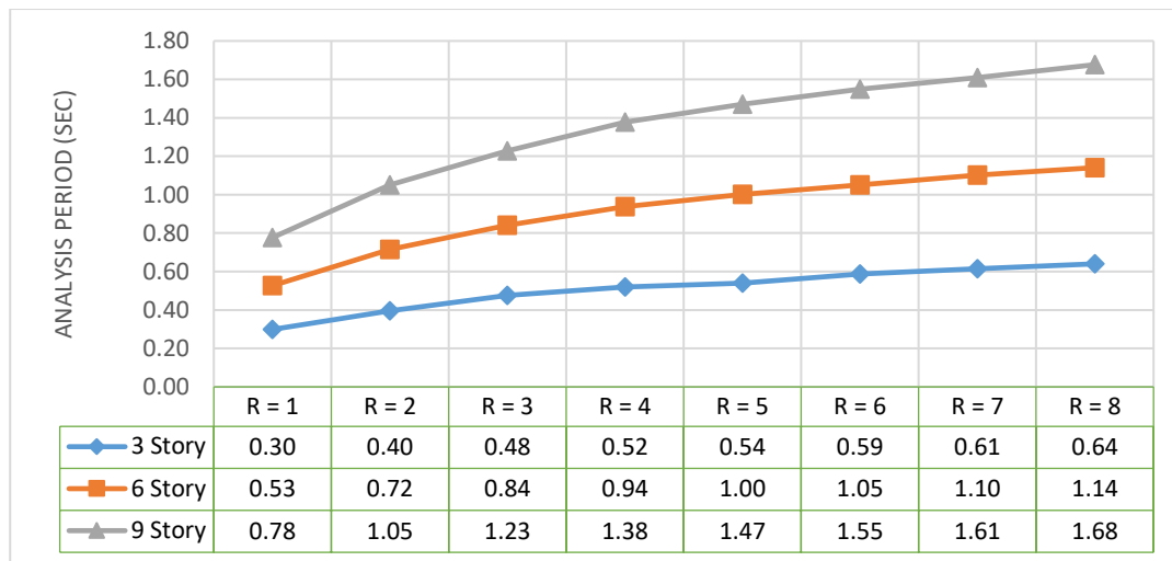
Figure 3.5. Fundamental periods of archetypes
