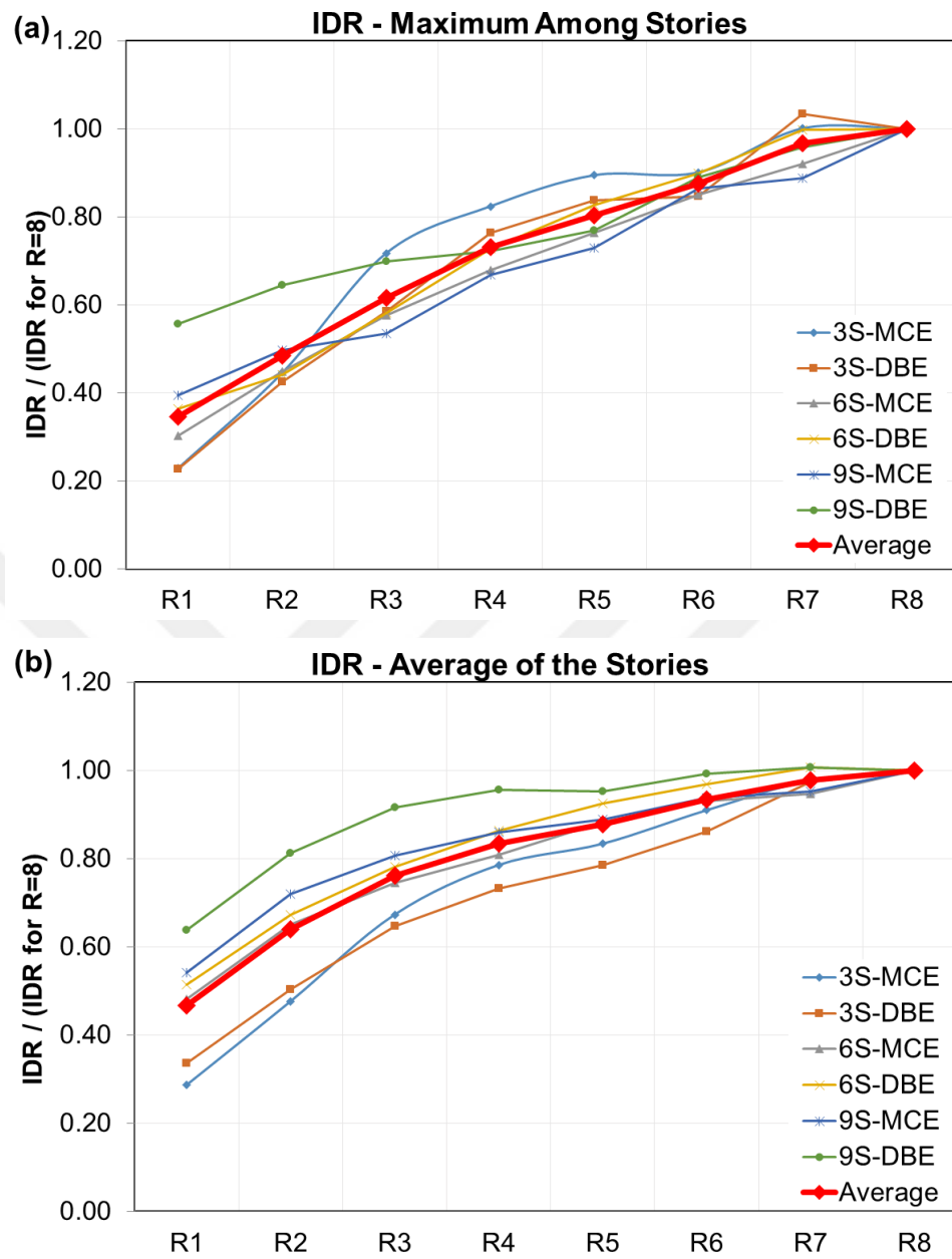
Figure 3.13. Variation of Normalized IDRs
