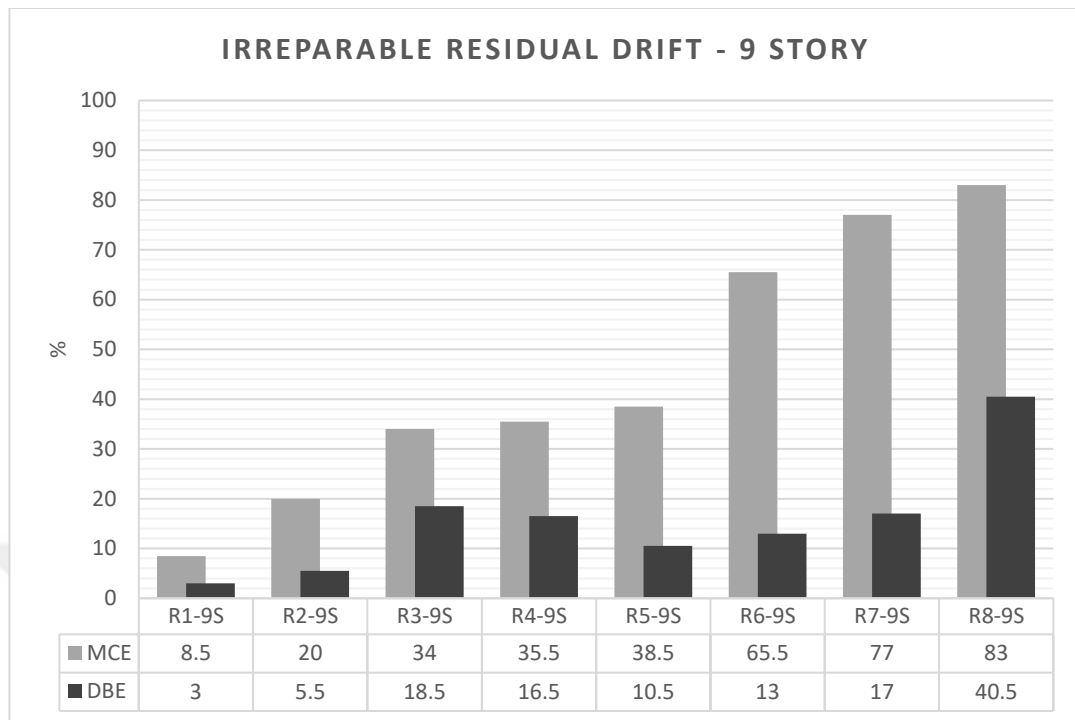
Figure 4.14. Irreparable residual drift probabilities for 9-Story archetypes
