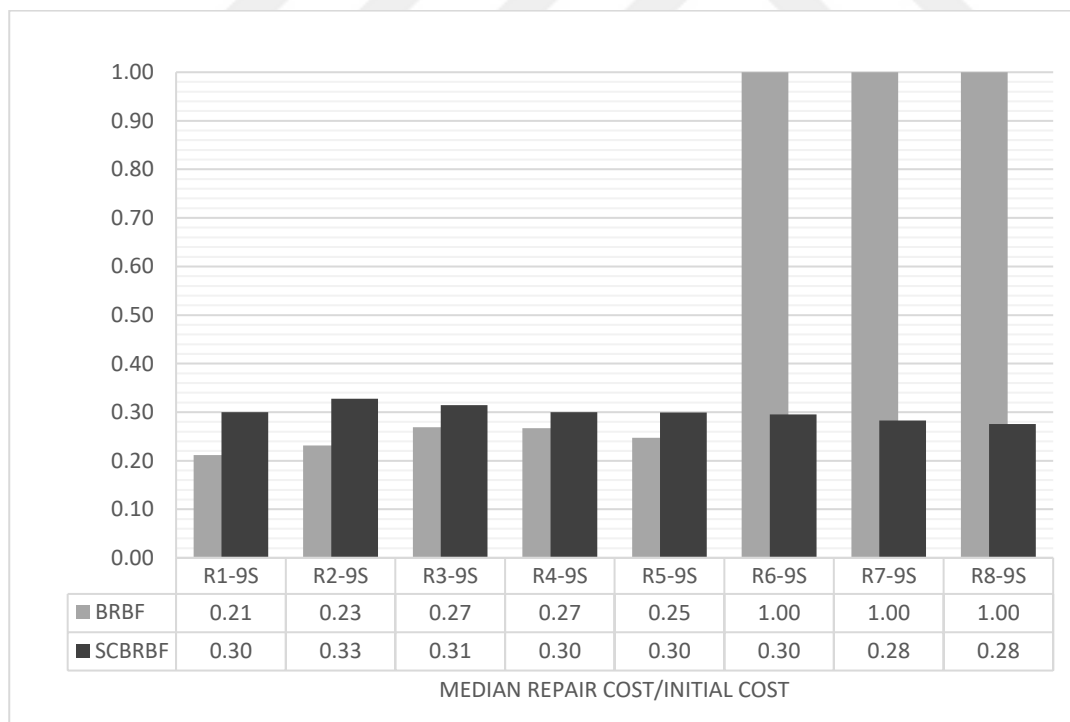
Figure 6.7. Median repair cost comparison of SCBRB and BRB (9-Story)
