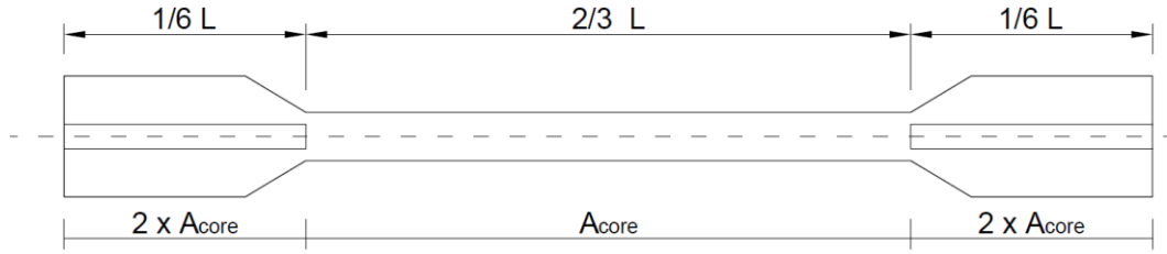
Figure 2.3. BRB core details
