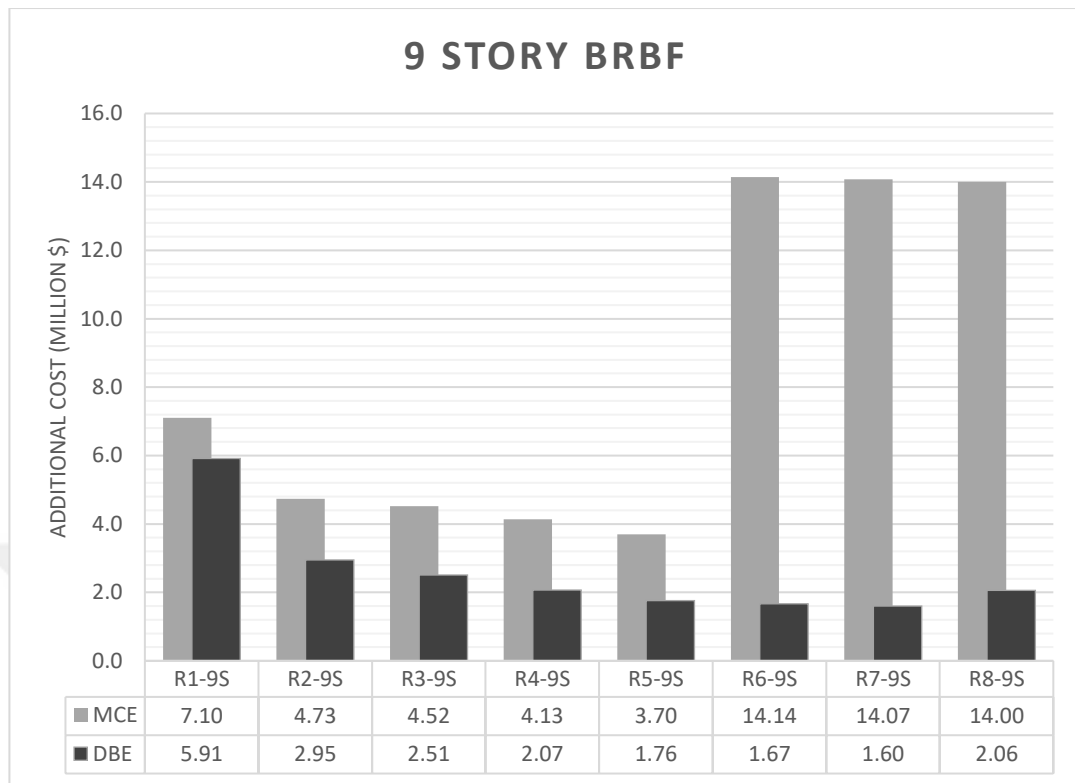
Figure 5.3. Additional Cost Analysis of 9 Story BRBF Archetypes
