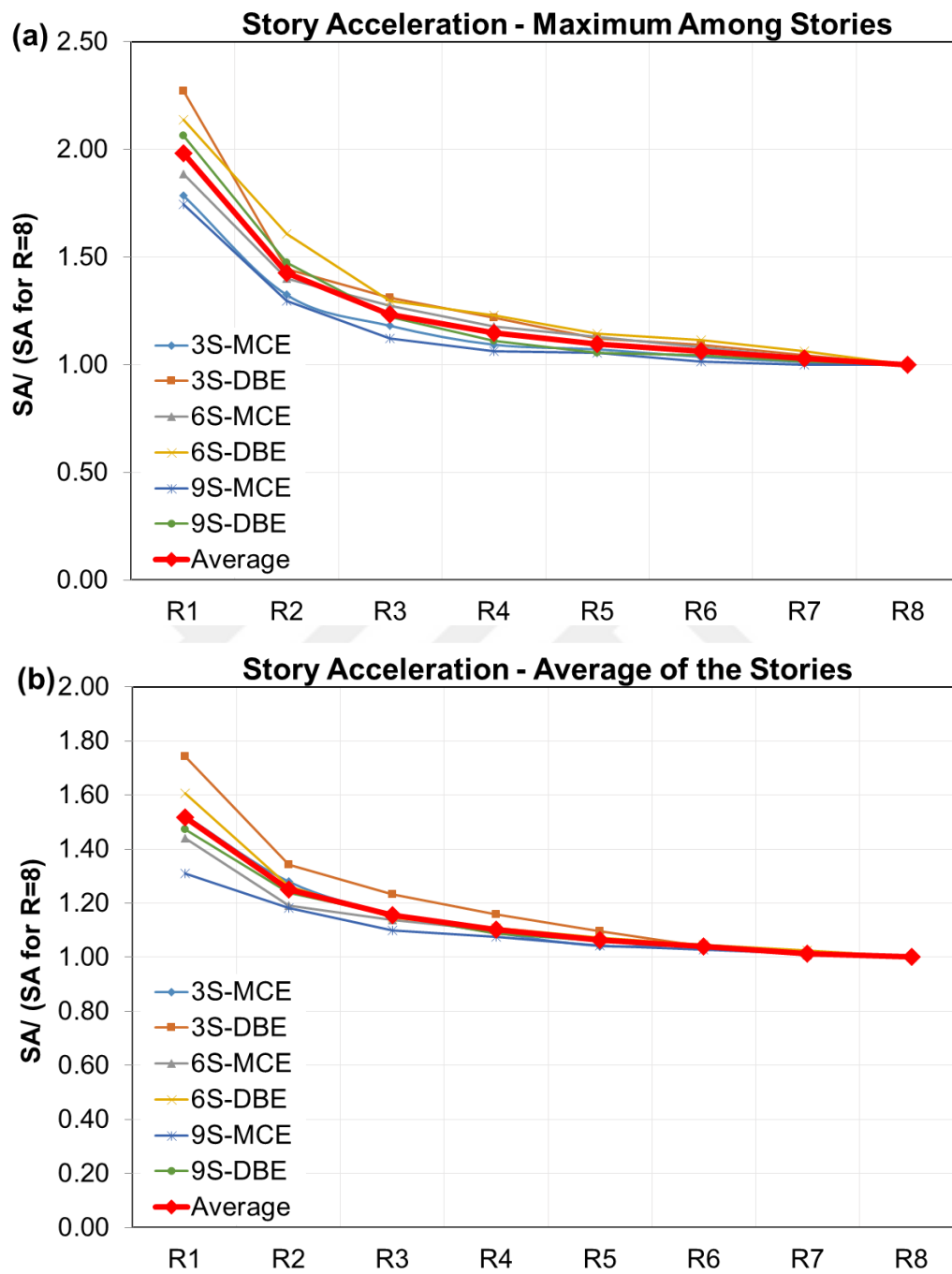
Figure 3.26. Variation of Normalized Story Accelerations
