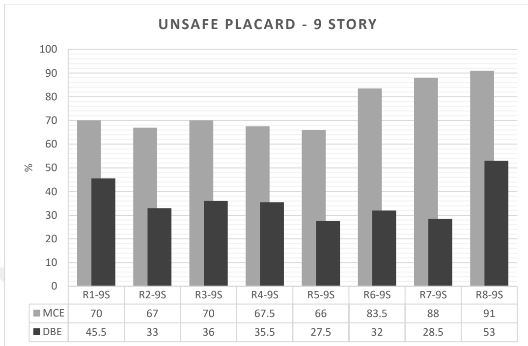
Figure 4.20. Unsafe placard probabilities for 9-Story archetypes
