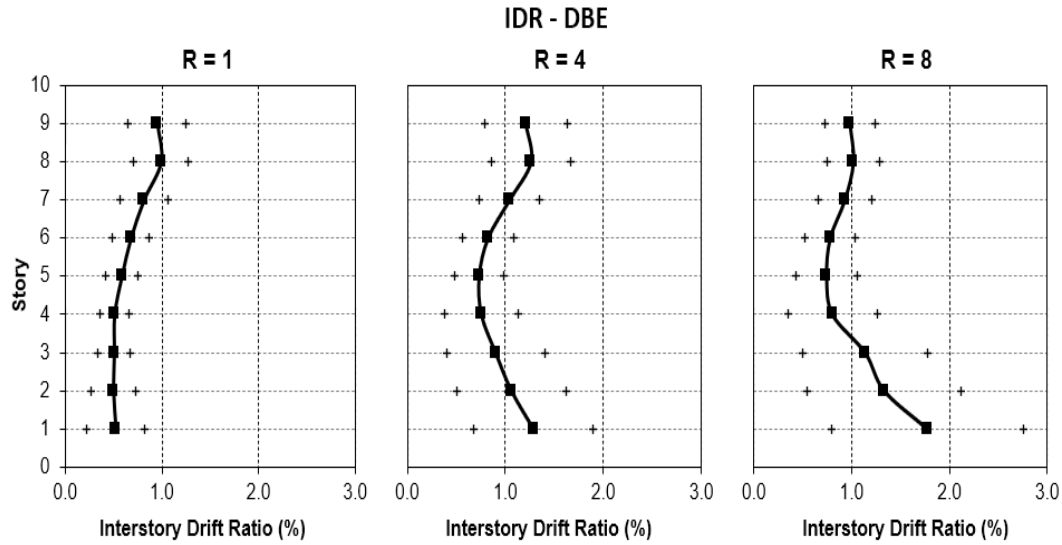
Figure 3.9. IDR Response of 9 Story Archetypes - DBE
