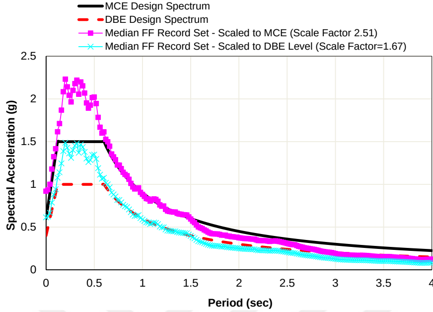
Figure 3.2. Scaling of the Far-Field Record Set for 9-story Archetypes
