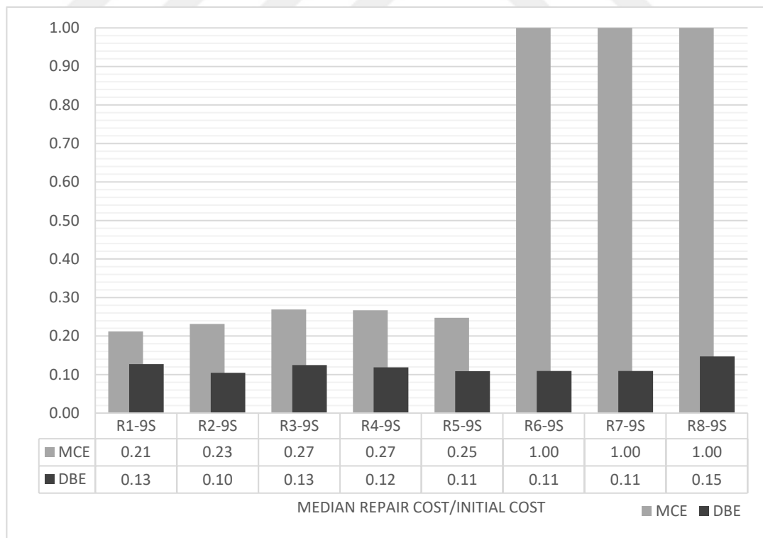
Figure 4.9. Normalized Median repair cost values for 9-Story archetypes
