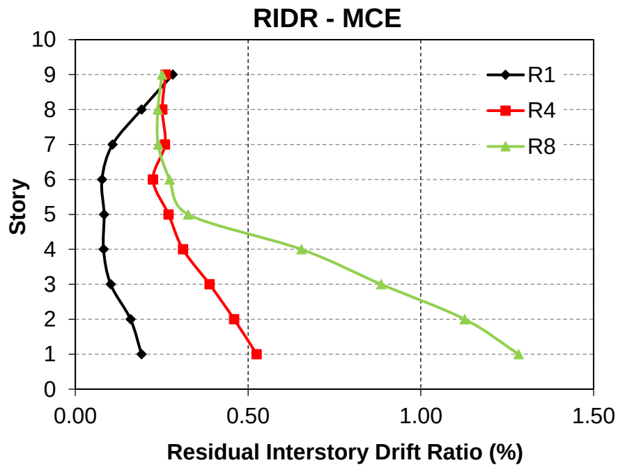
Figure 3.14. RIDR response of 9-story Archetypes - MCE
