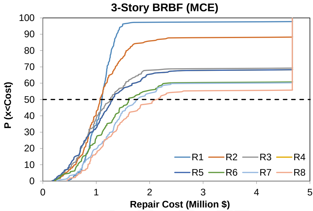
Figure 4.4. The repair cost non-exceedance probabilistic distribution (3-Story)
