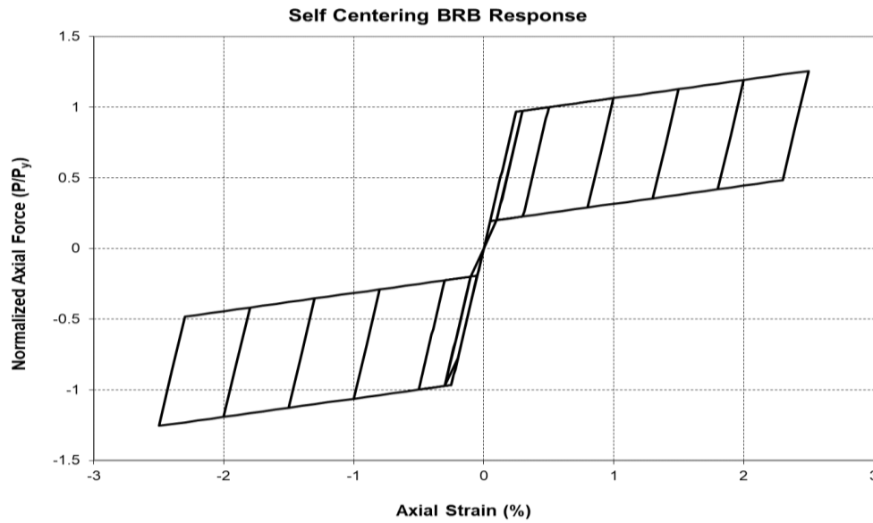
Figure 6.1. Response of Self-Centering BRB from OpenSees (Mazzoni et al. , 2006)
