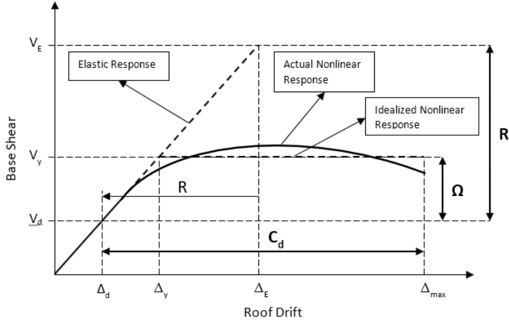
Figure 1.7. Inelastic Design Spectrum and Response Factors
