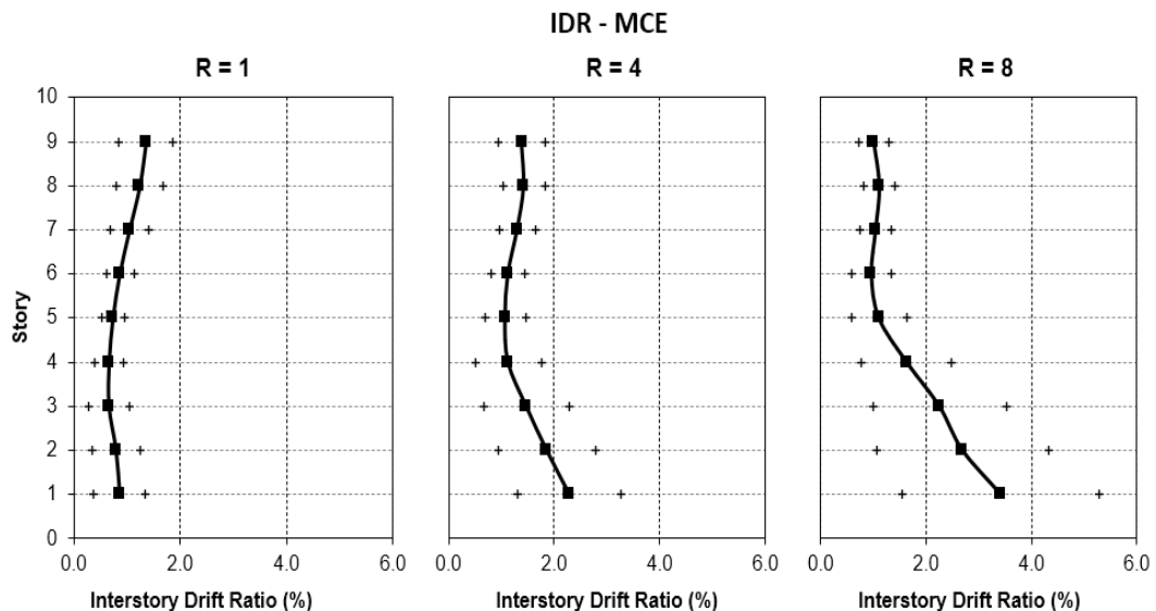
Figure 3.8. IDR Response of 9 Story Archetypes - MCE
