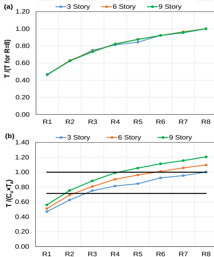
Figure 3.6. Normalized Fundamental Natural Periods of Archetypes
