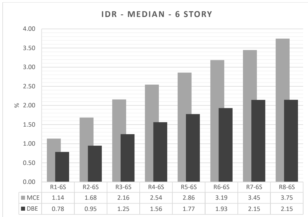
Figure 3.11. IDR demands for 6 Story archetypes (Median)
