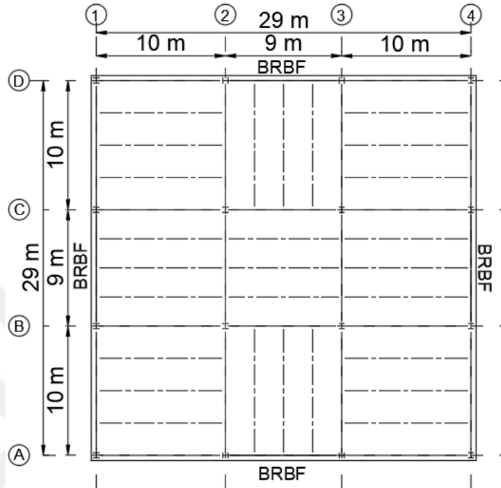
Figure 2.2. Floor plan
