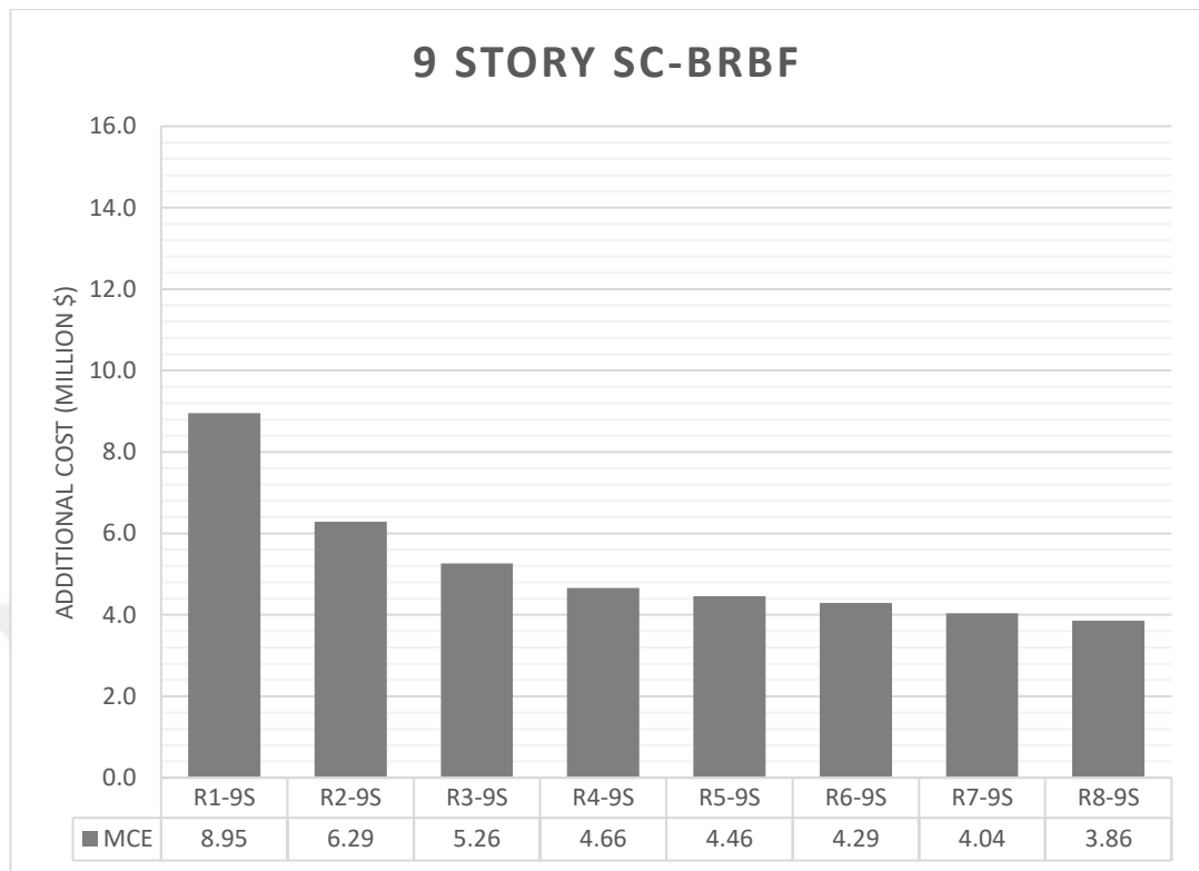
Figure 6.10. Additional Cost Analysis of 9 Story SC-BRBF Archetypes
