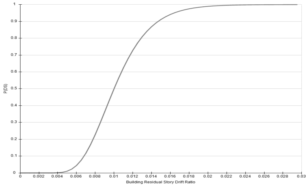
Figure 4.3. Irreparable damage probability distribution depends on R-IDR (FEMA, 2018c)
