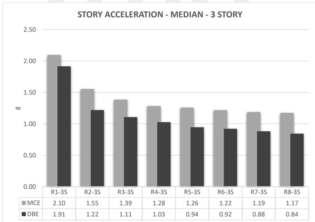
Figure 3.23. Peak story acceleration demands for 3 Story archetypes (Median)
