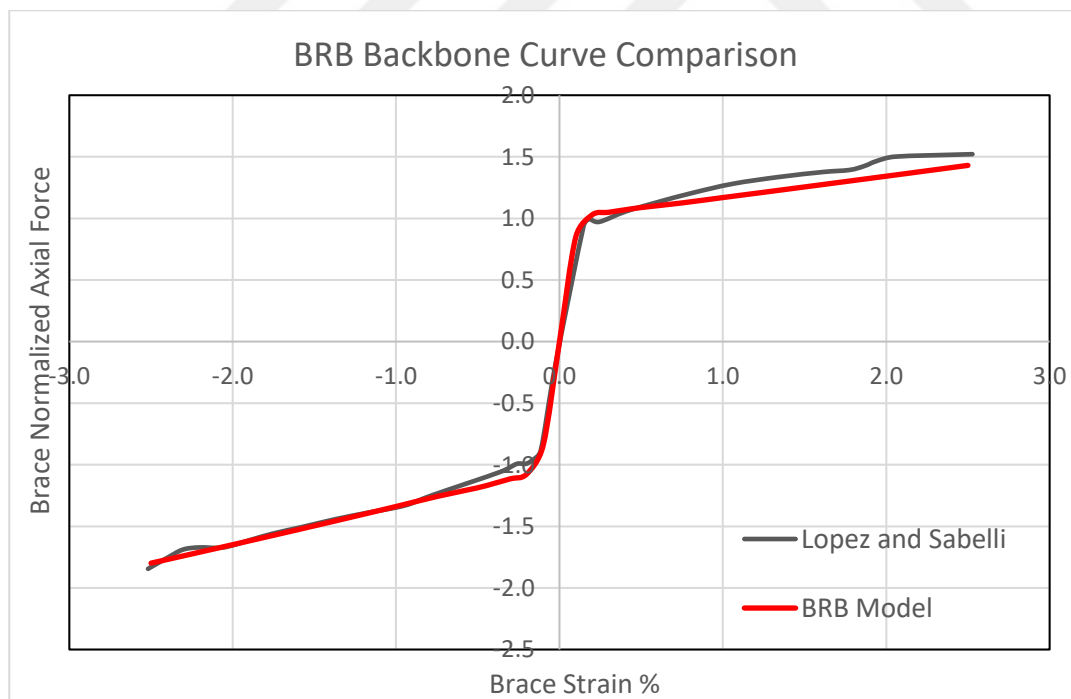
Figure 3.4. Backbone Curve Comparison of BRB numerical model and Lopez and Sabelli (2004) model
