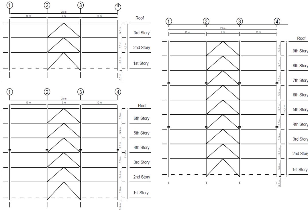
Figure 2.1. Elevation plan for archetypes
