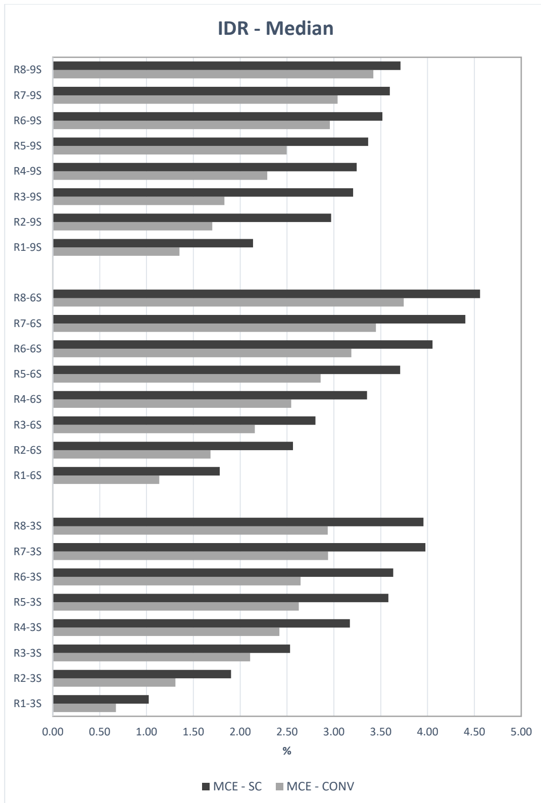
Figure 6.2. IDR Comparison of SCBRB and BRB at MCE (Max. among stories)
