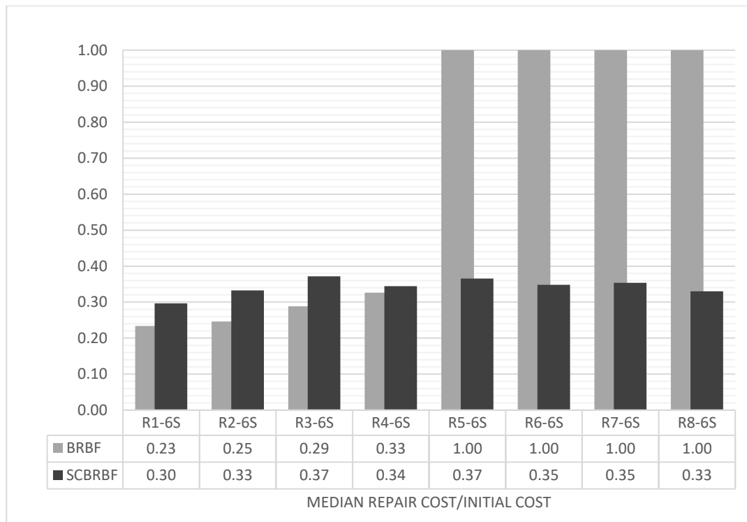
Figure 6.6. Median repair cost comparison of SCBRB and BRB (6-Story)
