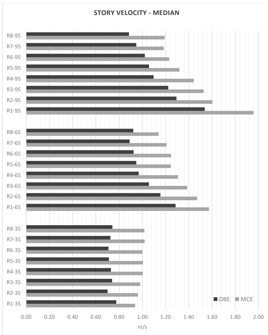
Figure 3.27. Peak story velocity demands (Median)
