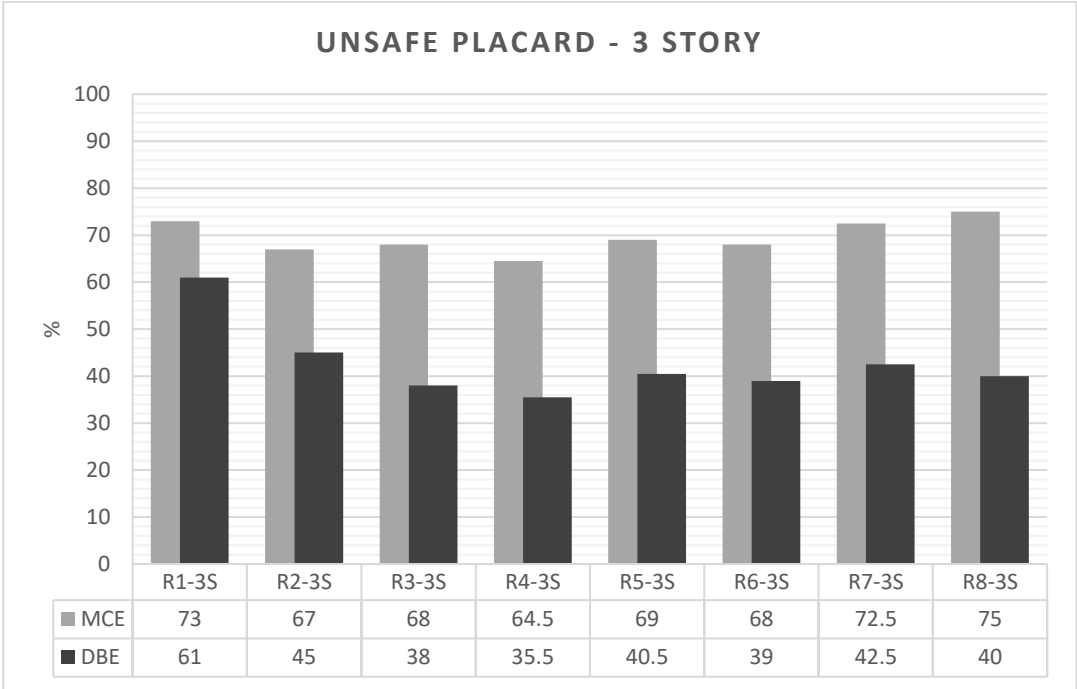
Figure 4.18. Unsafe placard probabilities for 3-Story archetypes
