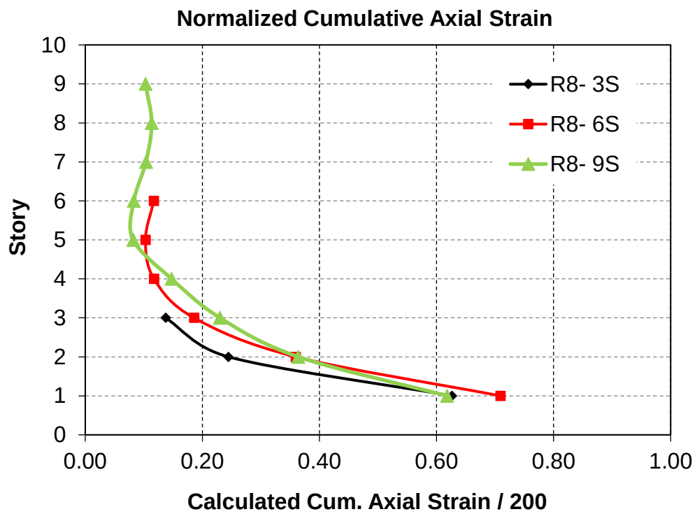
Figure 3.29. Normalized cumulative brace axial strain demands
