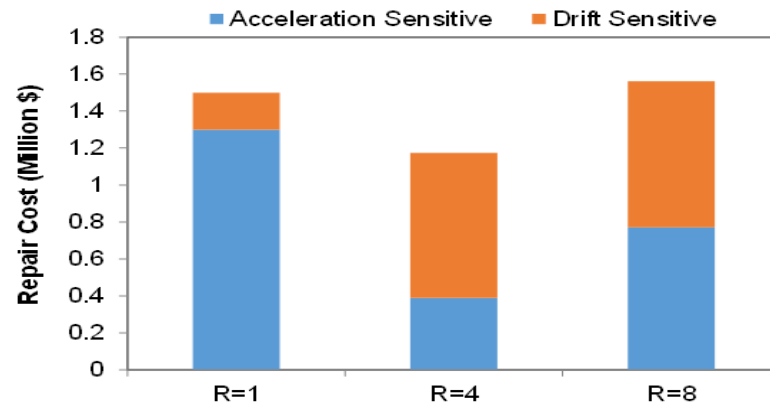
Figure 4.11. Decomposition of Repair Costs for 6-story Archetypes Subjected to DBE Level Ground Motions
