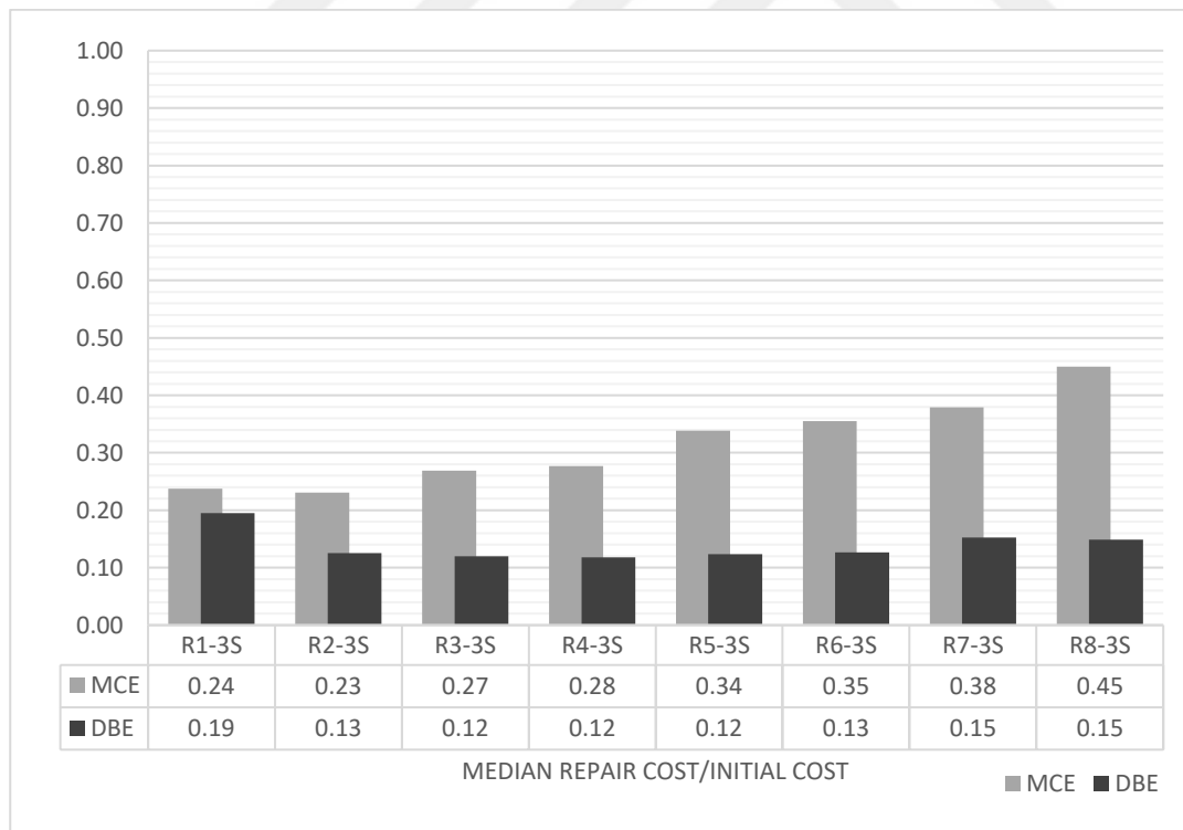
Figure 4.7. Normalized Median repair cost values for 3-Story archetypes
