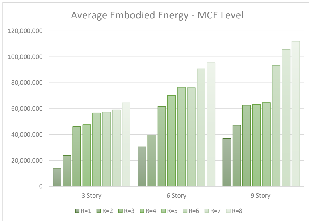
Figure 4.24. Average embodied energy values
