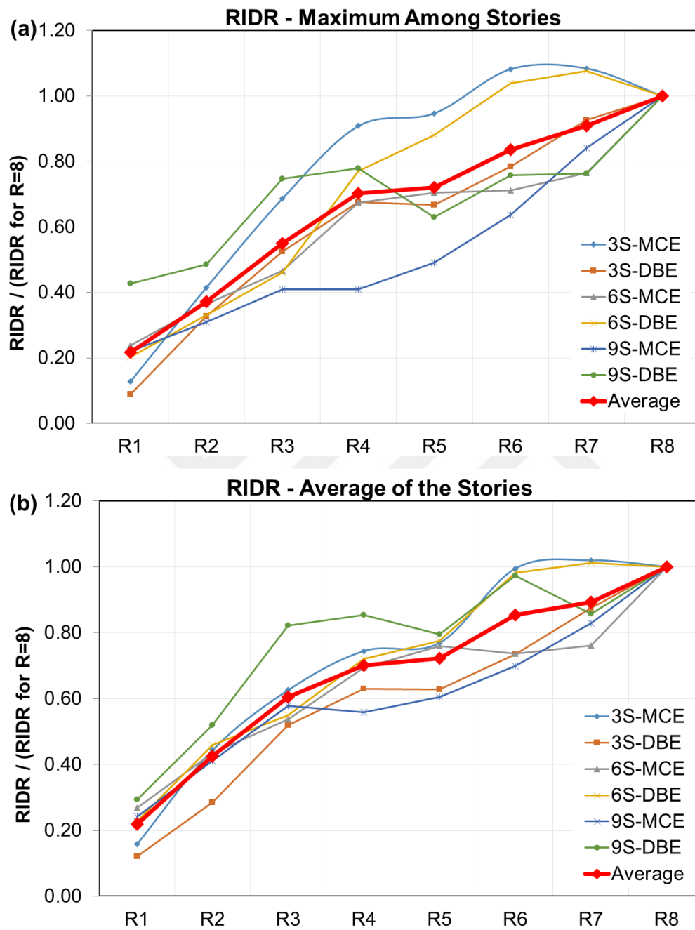
Figure 3.19. Variation of Normalized RIDRs
