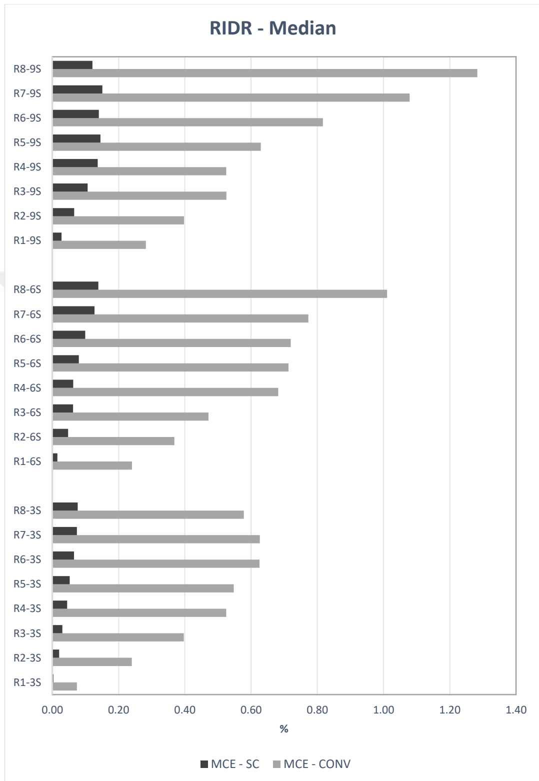
Figure 6.3. RIDR Comparison of SCBRB and BRB at MCE (Max. among stories)
