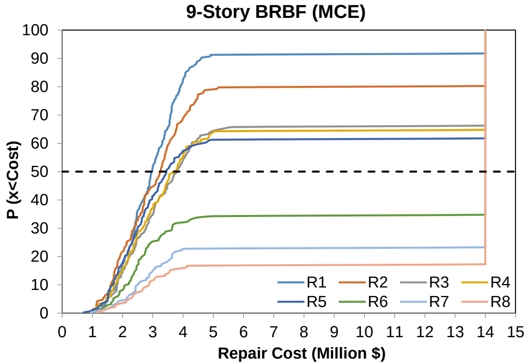
Figure 4.6. The repair cost non-exceedance probabilistic distribution (9-Story)
