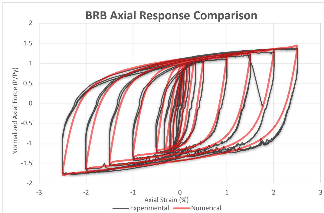
Figure 3.3. Comparison of BRB numerical model and experimental model
