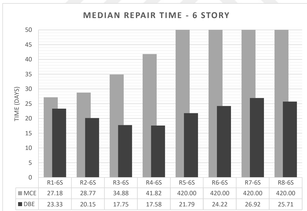
Figure 4.16. Median repair time values for 6-Story archetypes
