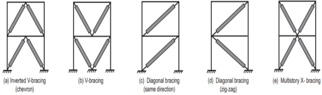
Figure 1.6. Common BRB configurations
