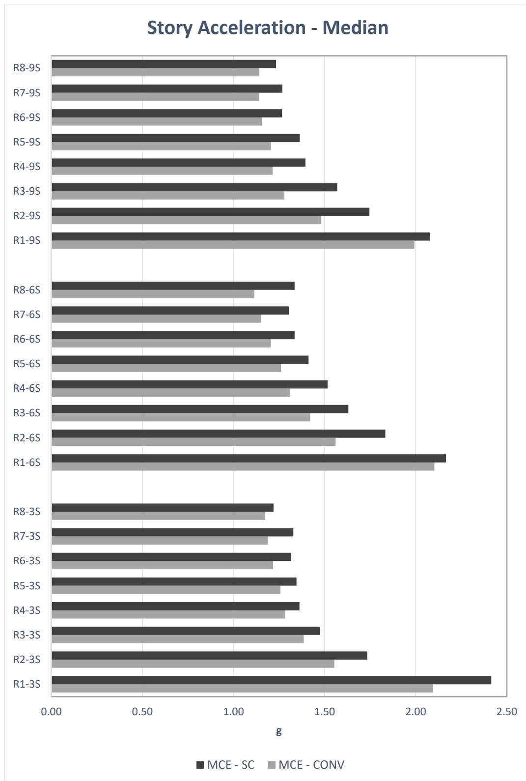
Figure 6.4. SA Comparison of SCBRB and BRB at MCE (Max. among stories)
