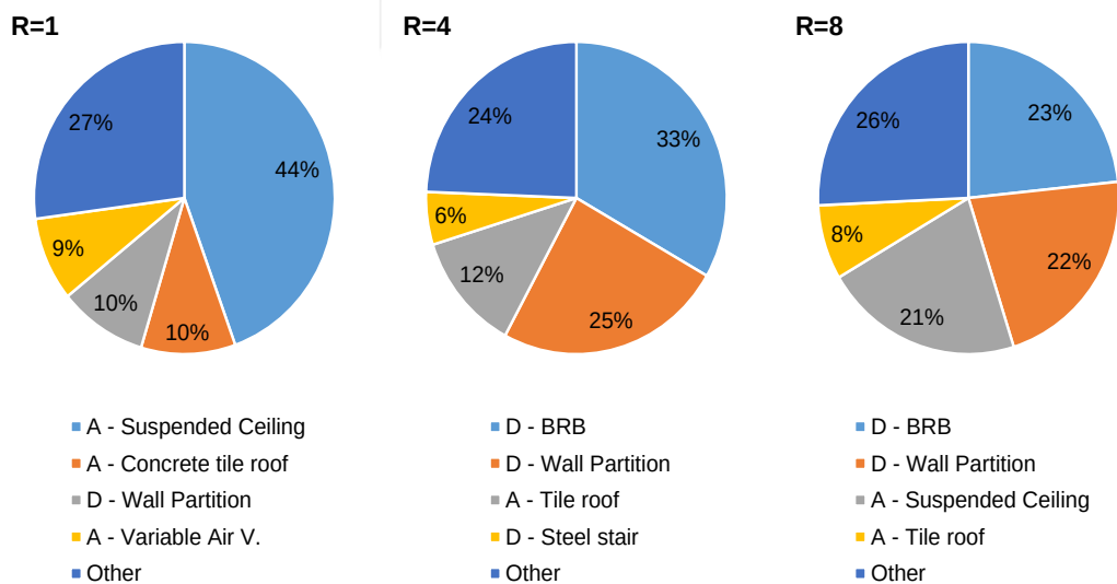
Figure 4.10. Repair Costs of Components for 6-story Archetypes
