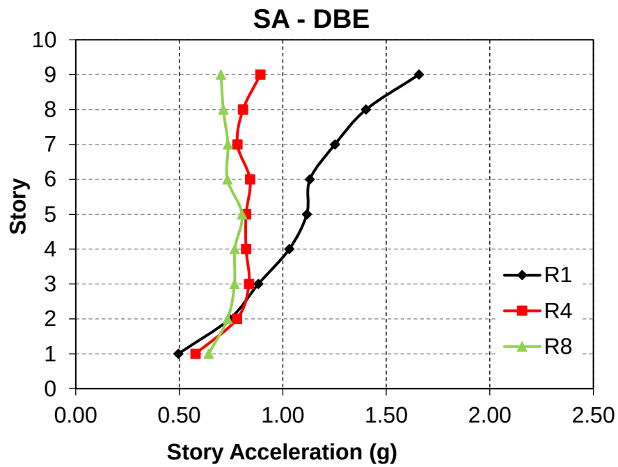
Figure 3.22. Story Acceleration response of 9-story Archetypes - DBE
