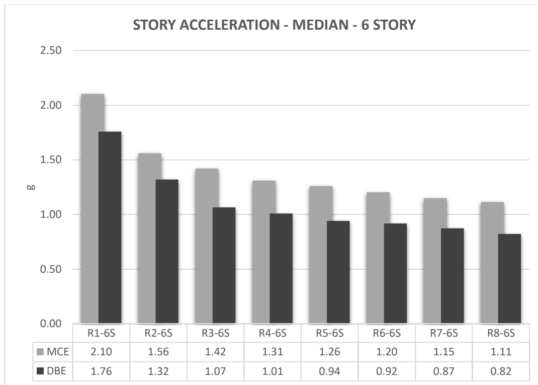
Figure 3.24. Peak story acceleration demands for 6 Story archetypes (Median)
