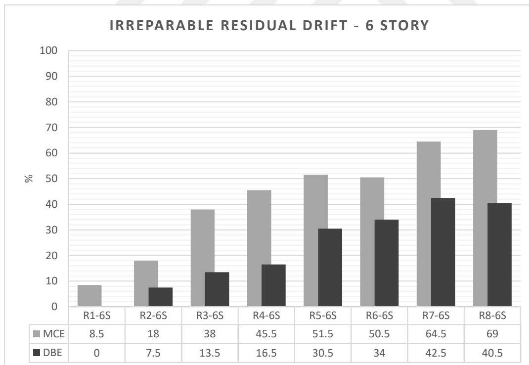
Figure 4.13. Irreparable residual drift probabilities for 6-Story archetypes
