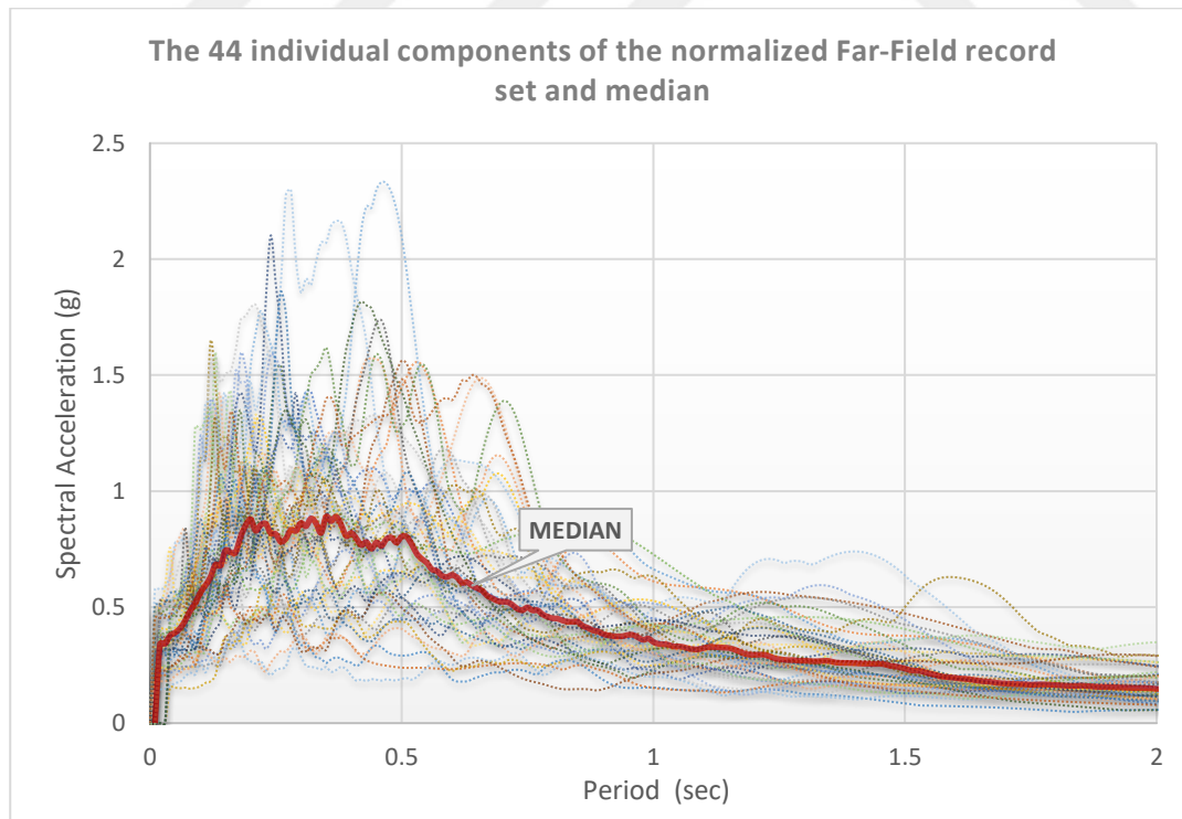
Figure 3.1. FEMA P695 FF Record Set Spectrum
