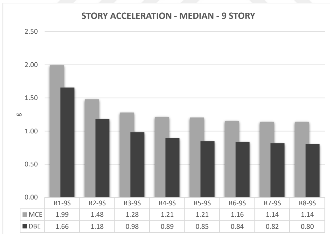
Figure 3.25. Peak story acceleration demands for 9 Story archetypes (Median)
