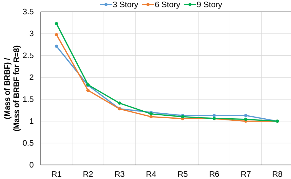
Figure 2.7. Mass of a Single BRBF Bay Excluding BRBs
