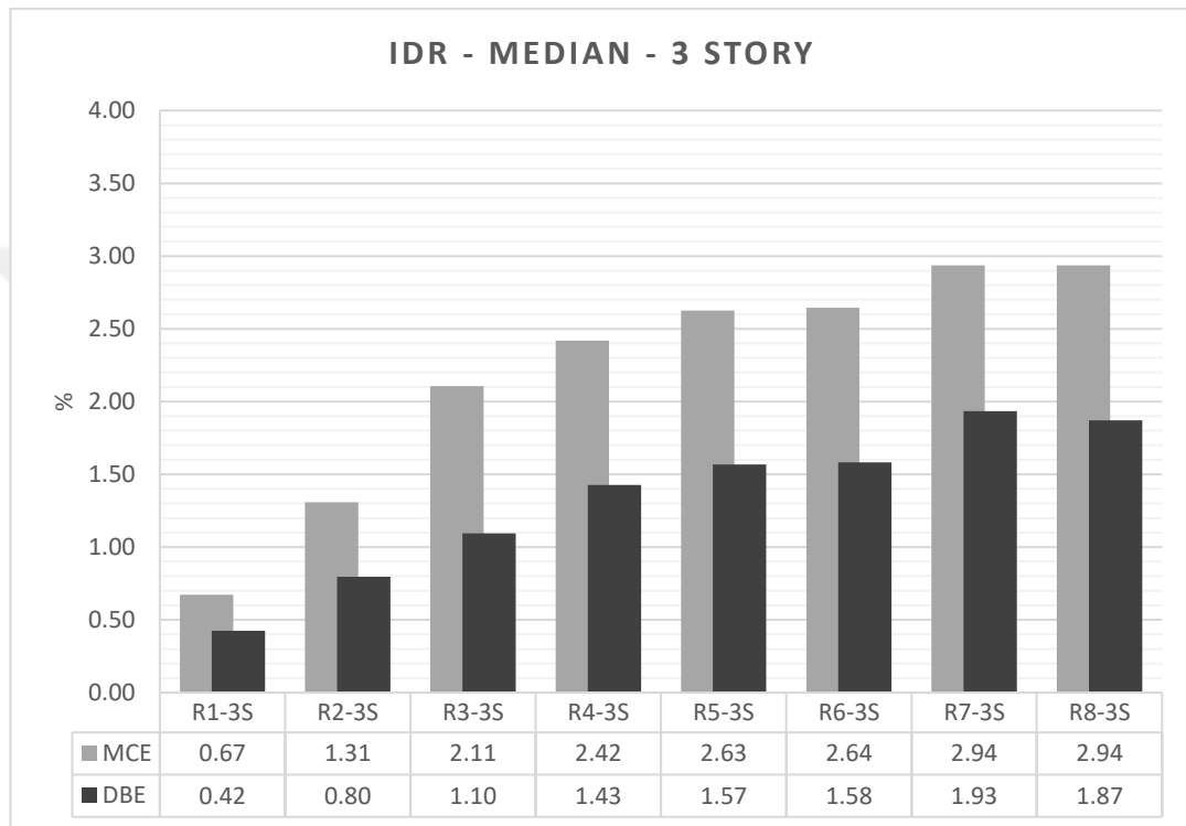
Figure 3.10. IDR demands for 3 Story archetypes (Median)
