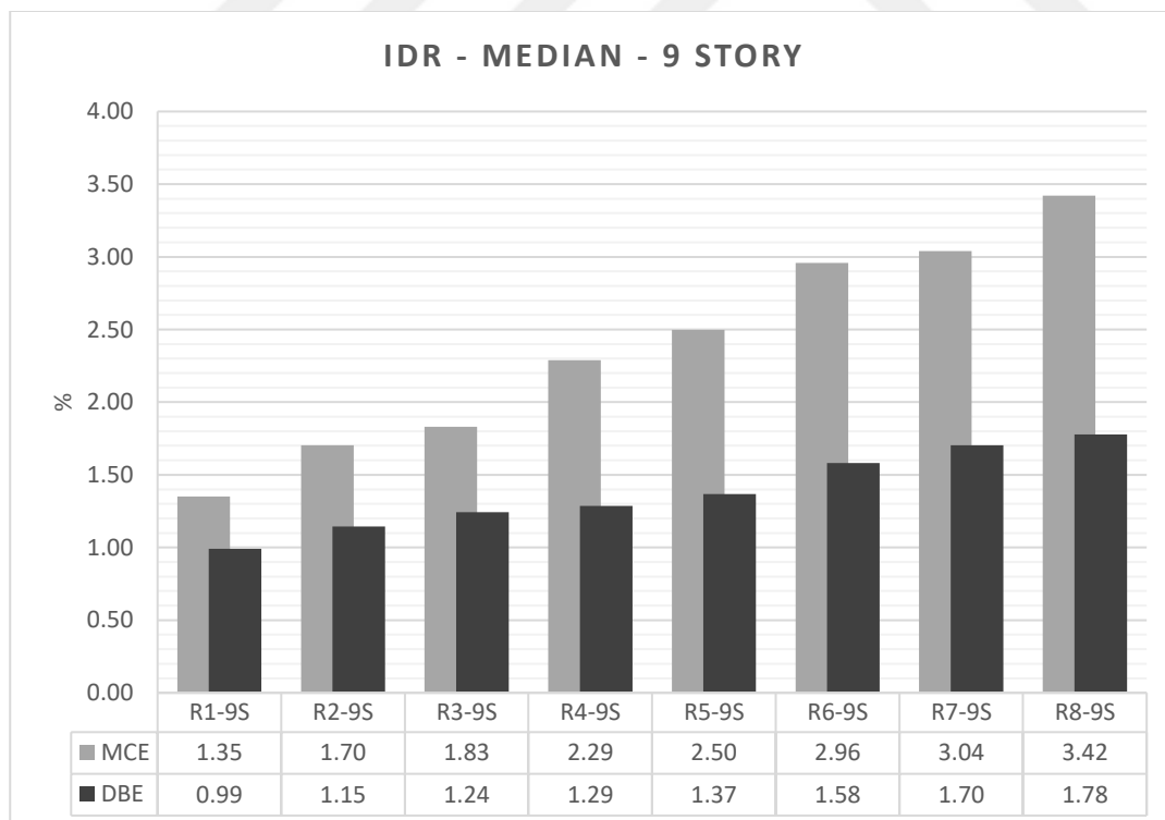
Figure 3.12. IDR demands for 9 Story archetypes (Median)
