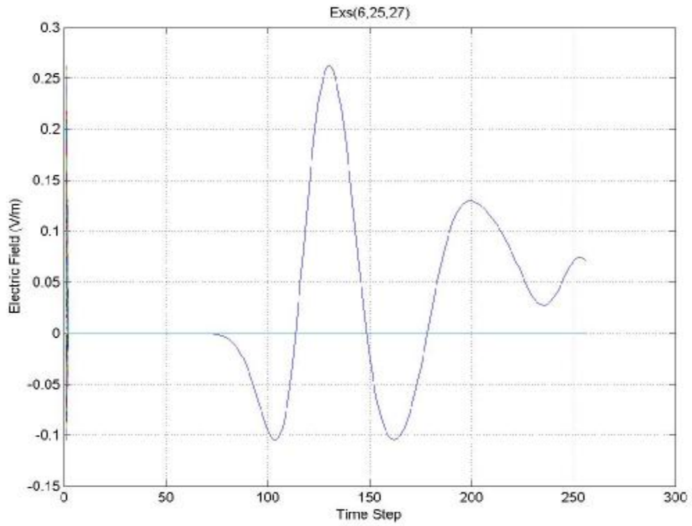
Figure 3.2. Electric field value versus time step in the Ex(6,25,27)
