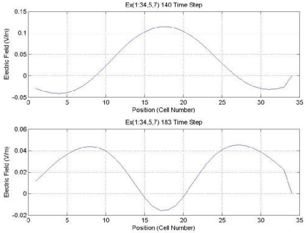
Figure 3.6. Electric field value versus position (cell number) in the Ex(1:34,7,5) for 140. and 183. time steps
