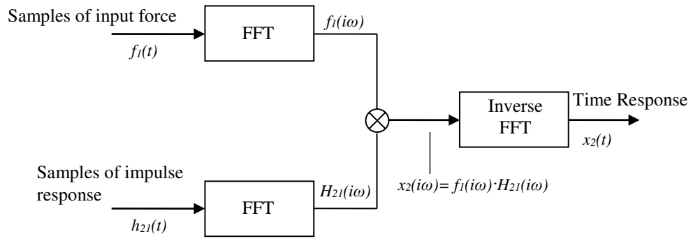
Figure 4.7 Obtaining time response procedure with signal analysis.
