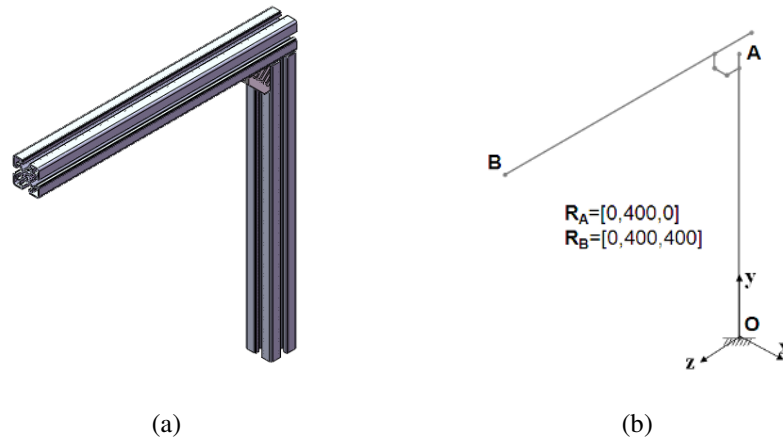
Figure 2.10 L-frame (LF-45) (a) Solid model for simulations, (b) line model.
