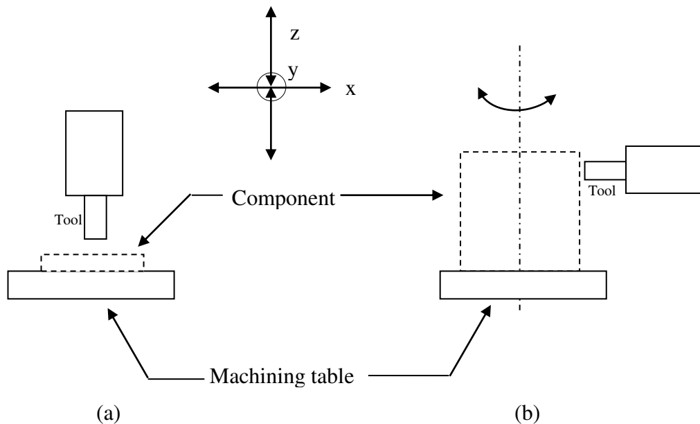
Figure 1.1 CNC machining centers: (a) vertical; (b) horizontal.
