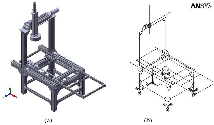
Figure 3.15 Solid model and finite element model of the system at position \mathbf{q}_e=[700,200,400] .
