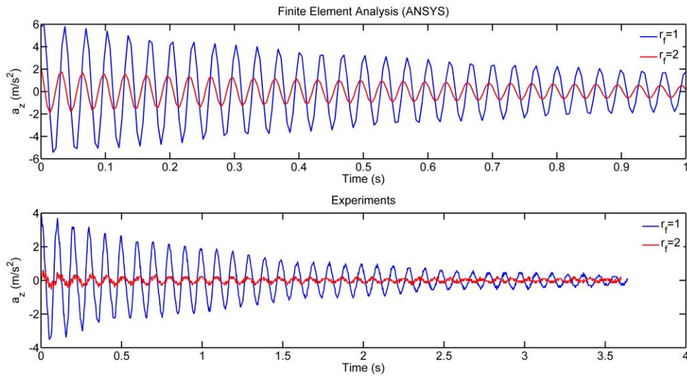
Figure 4.13 Residual vibrations.
