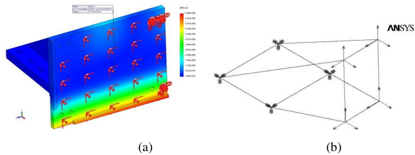
Figure 3.10 Static analysis results for Connector-yz, u_{\text{sum}}=1.814 \times 10^{-10} m (a), u_{\text{sum}}=1.814 \times 10^{-10} m (b).
