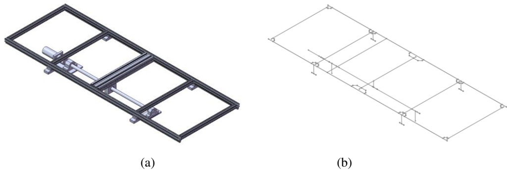
Figure 3.8 (a) Solid model, and (b) line model of LM-x.
