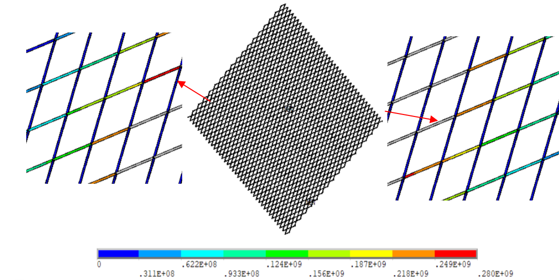
Figure 3.14. Tensile stress diagram of the expanded steel sheet (Pa)
