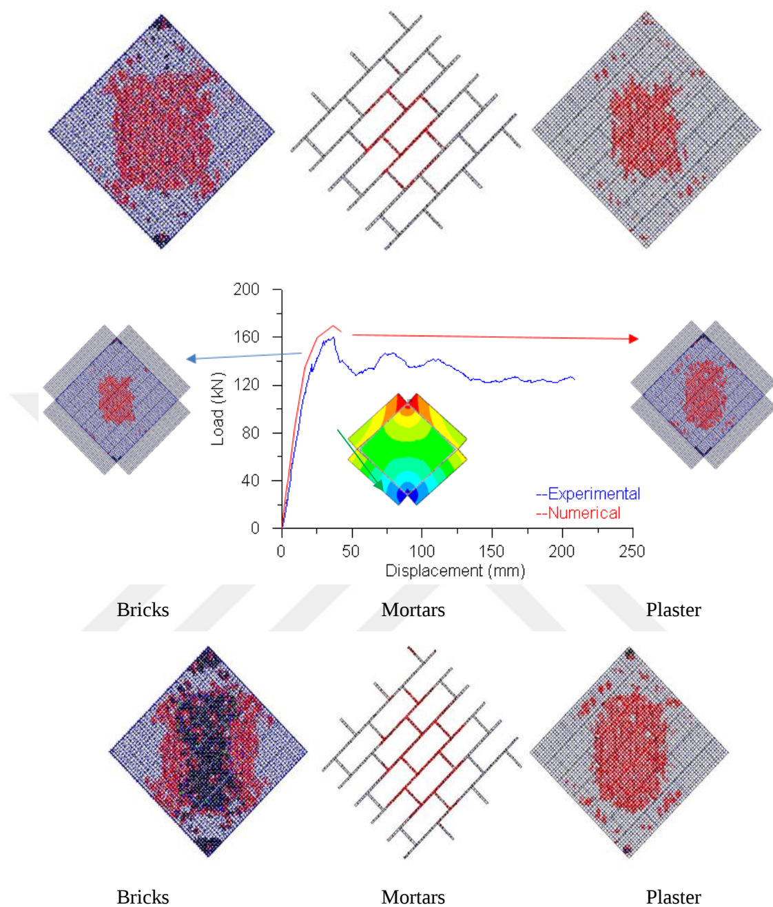
Figure 3.19. Load-displacement curve, deformation shape, and crack pattern of MBW 3.0-150 model
