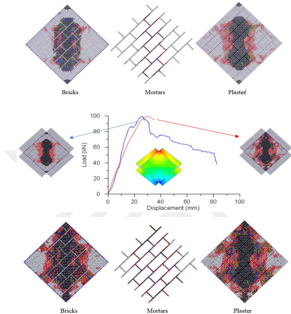
Figure 3.12. Load-displacement curve, deformation shape, and crack pattern of the reference model
