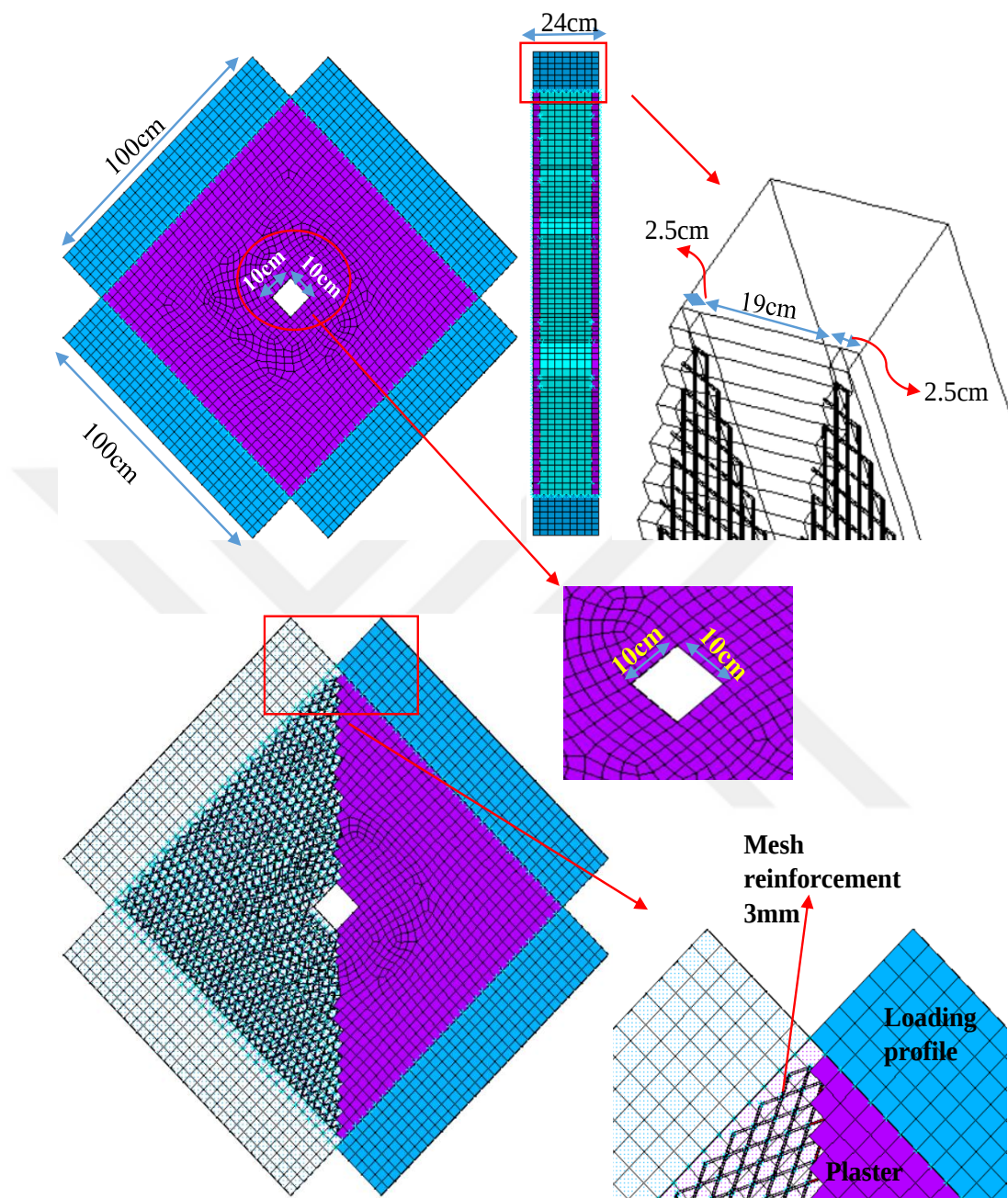
Figure 4.3. 10% opening ratio of the masonry wall model-3.0mm mesh reinforcement
