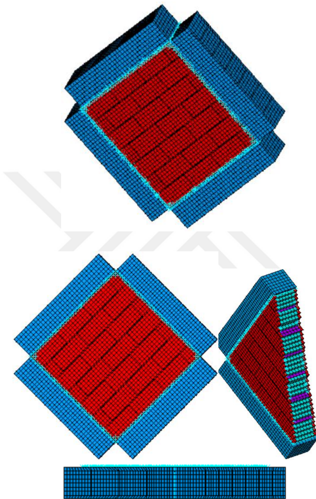
Figure 3.6. FE model of the masonry walls
