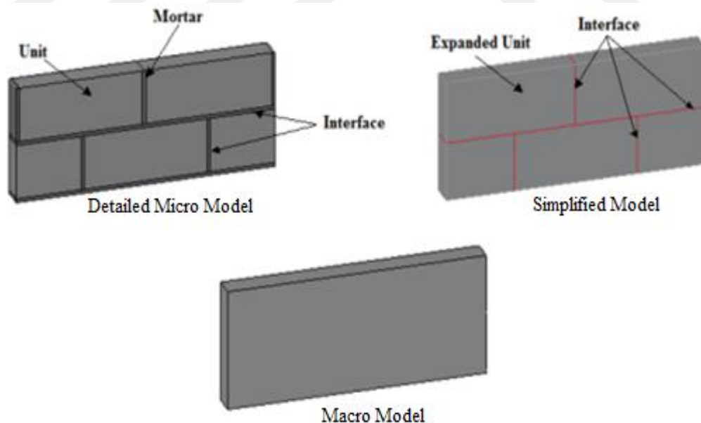
Figure 3.3. Masonry modeling techniques
