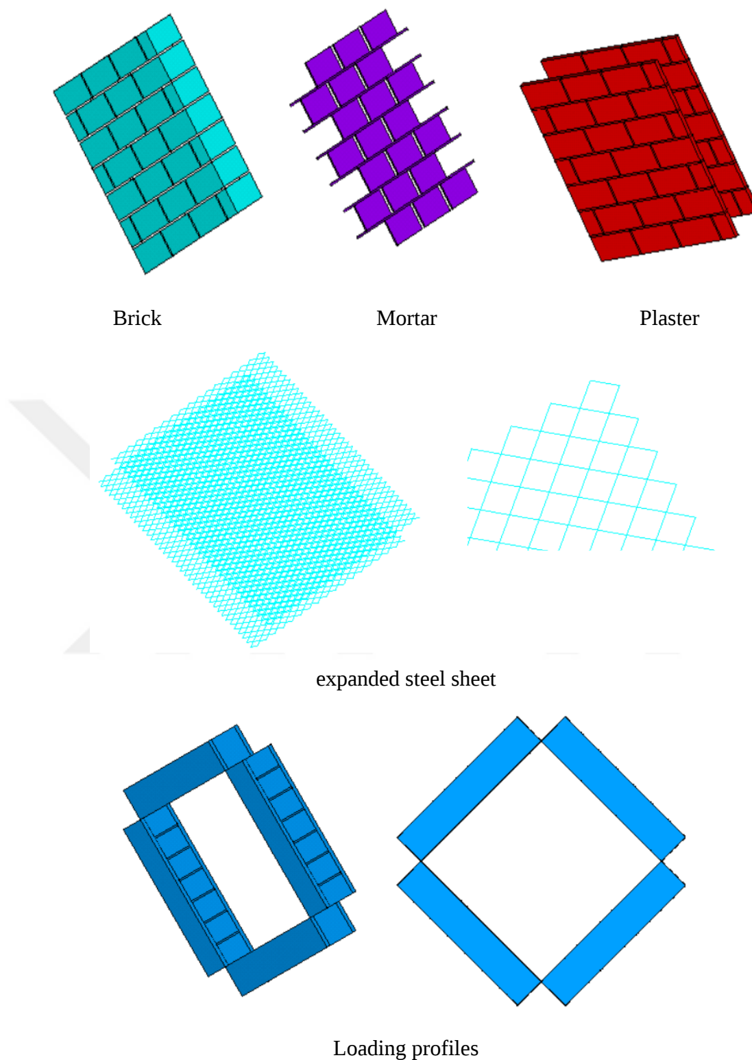
Figure 3.5. Parts of the FE model
