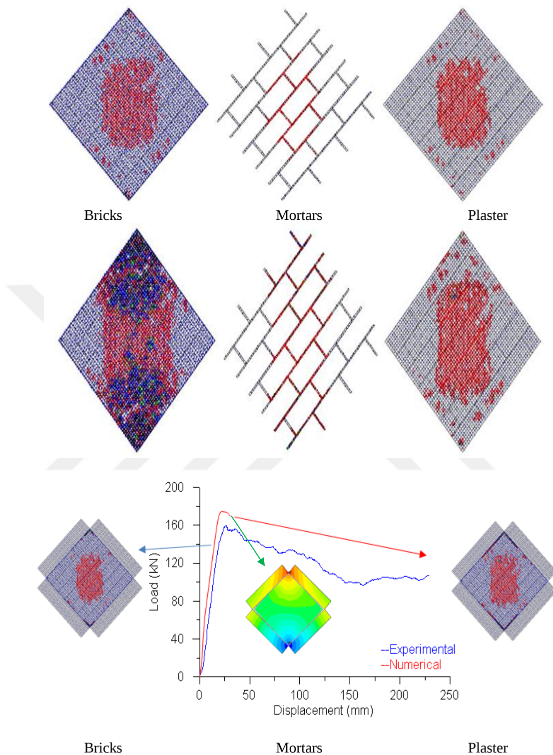
Figure 3.17. Load-displacement curve, deformation shape, and crack pattern of MBW 2.0-150 model
