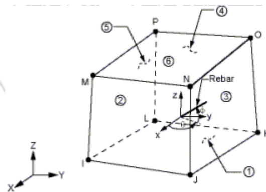
Figure 1.2. SOLID 65 element
