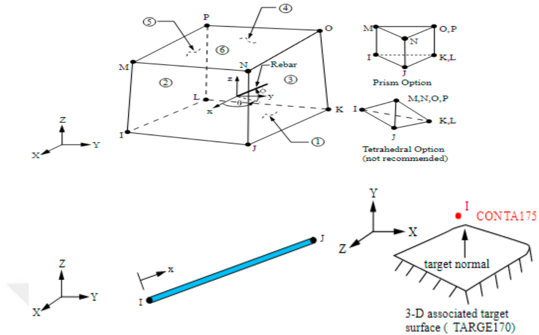
Figure 3.4. Schematic views of the SOLID65, LINK180, TARGE170, and CONTA175 element types [54]
