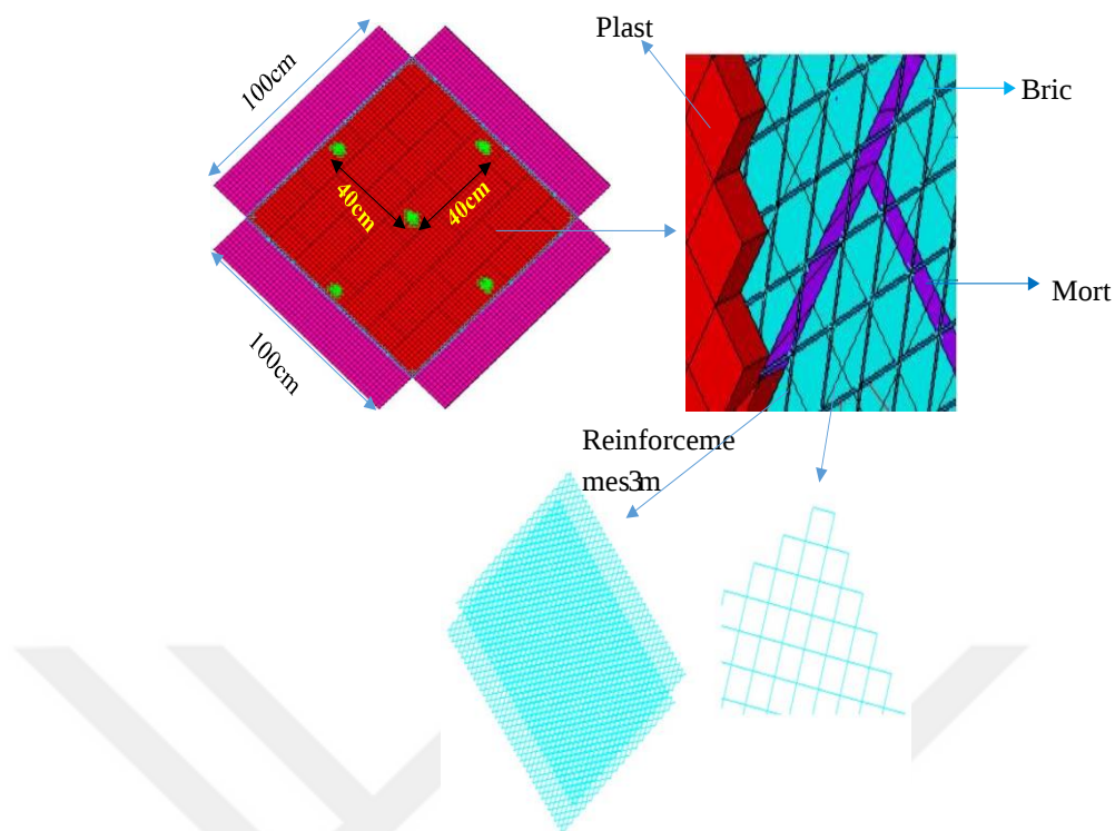
Figure 3.10. Dimensions of the MBW 3.0-400 the numerical model [3]
