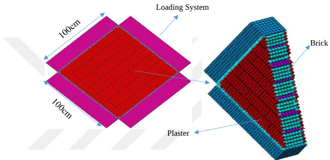
Figure 3.9. Dimensions of the reference of the numerical model [3]
