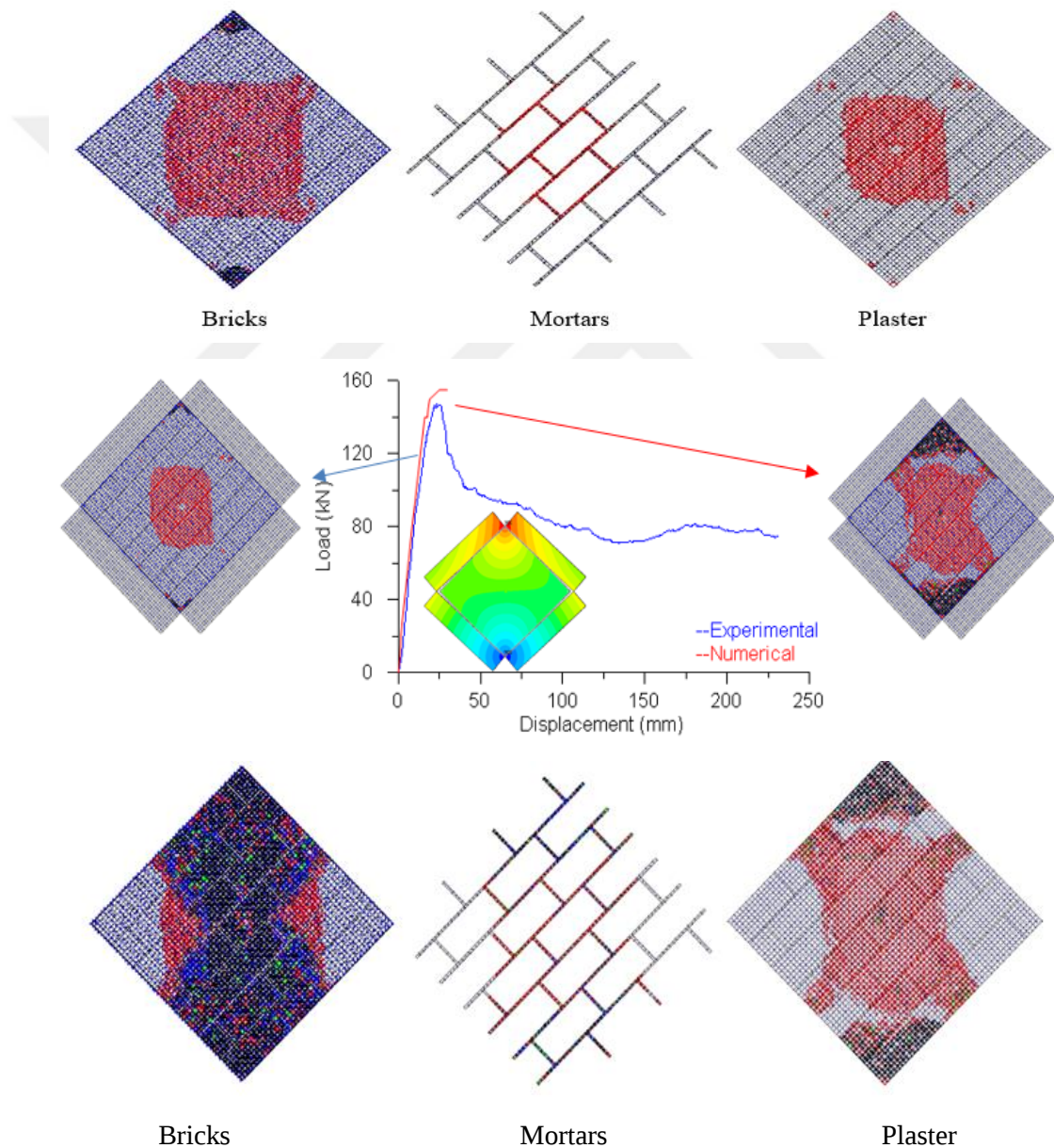
Figure 3.13. Load-displacement curve, deformation shape, and crack pattern of MBW 3.0-400 model
