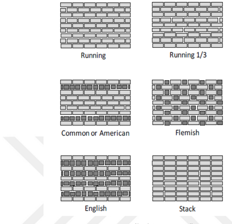
Figure 2.14. Types of bonds in a masonry wall
