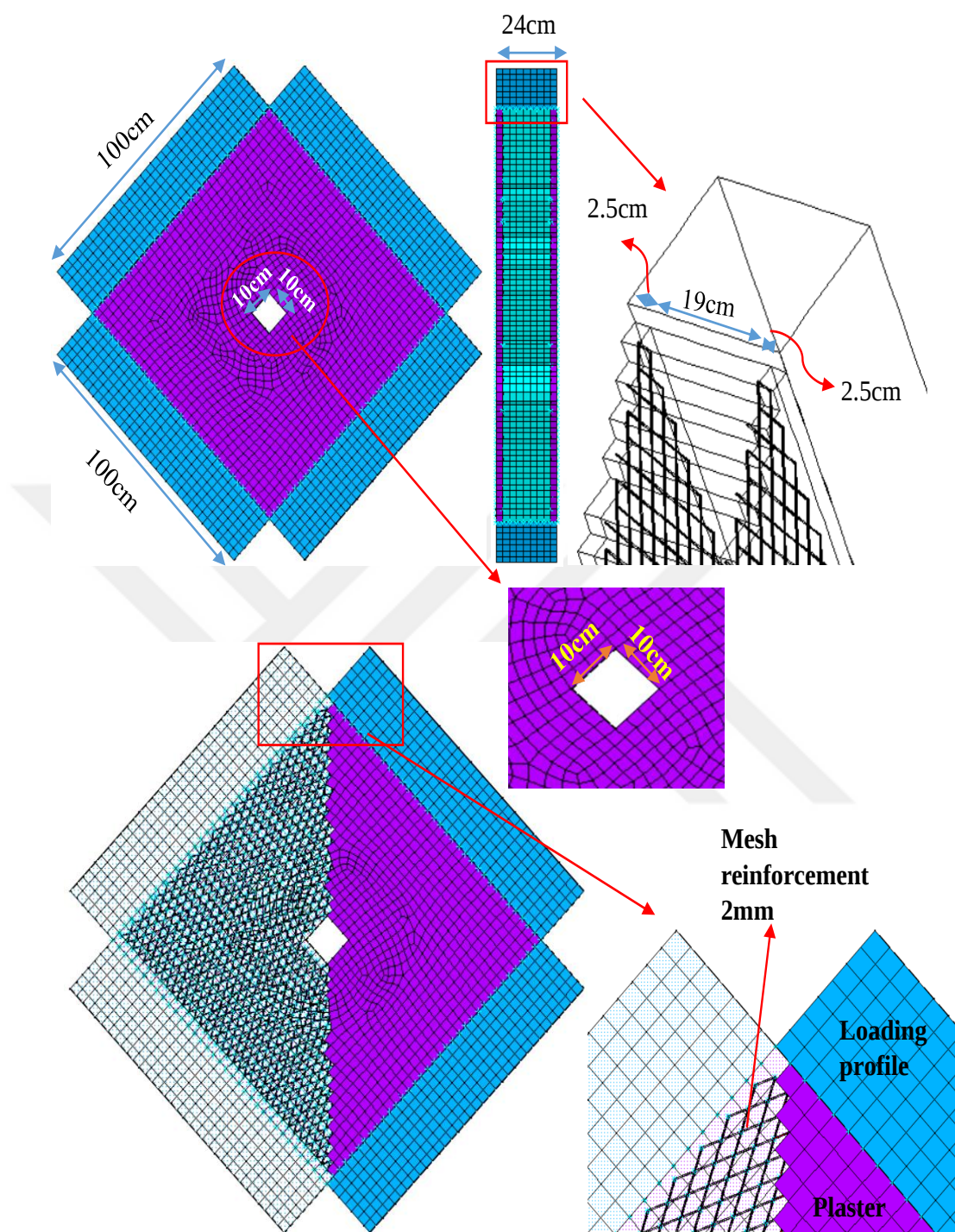
Figure 4.2. 10% opening ratio of the masonry wall model-2.0mm mesh reinforcement
