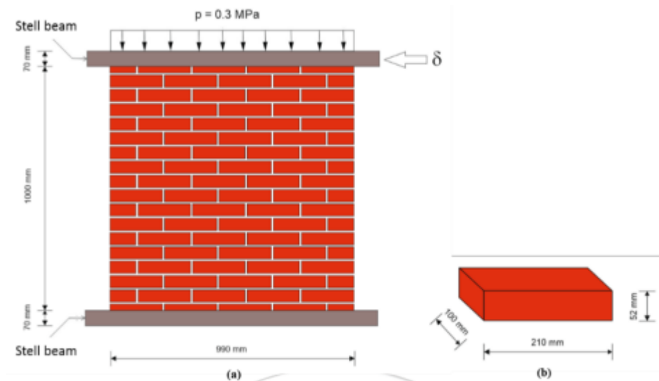
Figure 1.1. (a) Masonry wall geometry (b) masonry unit used in the wall [11]
