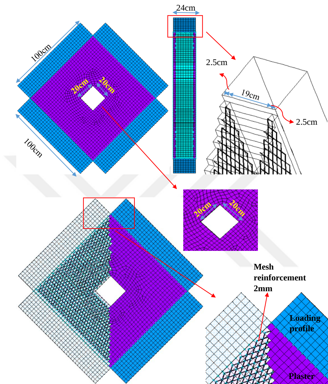
Figure 4.5. 20% opening ratio of the masonry wall model-2.0mm mesh reinforcement
