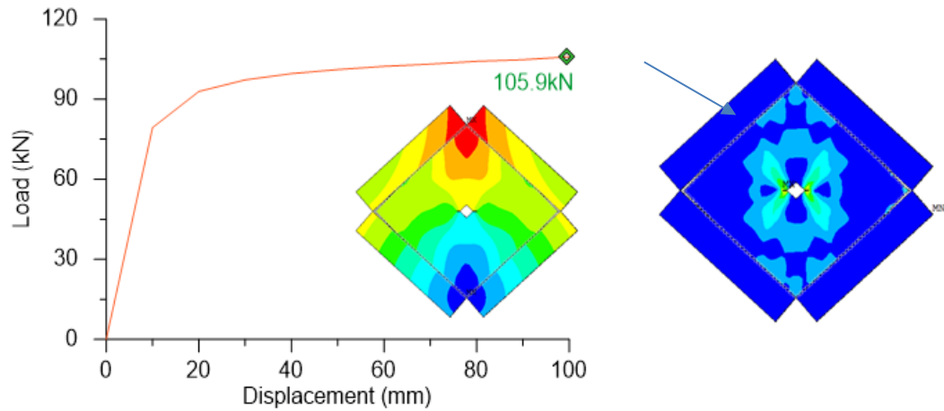
Figure 4.7. Load-Displacement curve, deformation shape, and total mechanical strain diagram of the wall with 10% opening (thickness of steel mesh 1.5mm)
