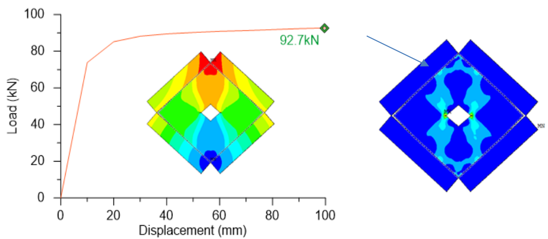
Figure 4.12. Load-Displacement curve, deformation shape, and total mechanical strain diagram of the wall with 20% opening (thickness of steel mesh 3.0mm)
