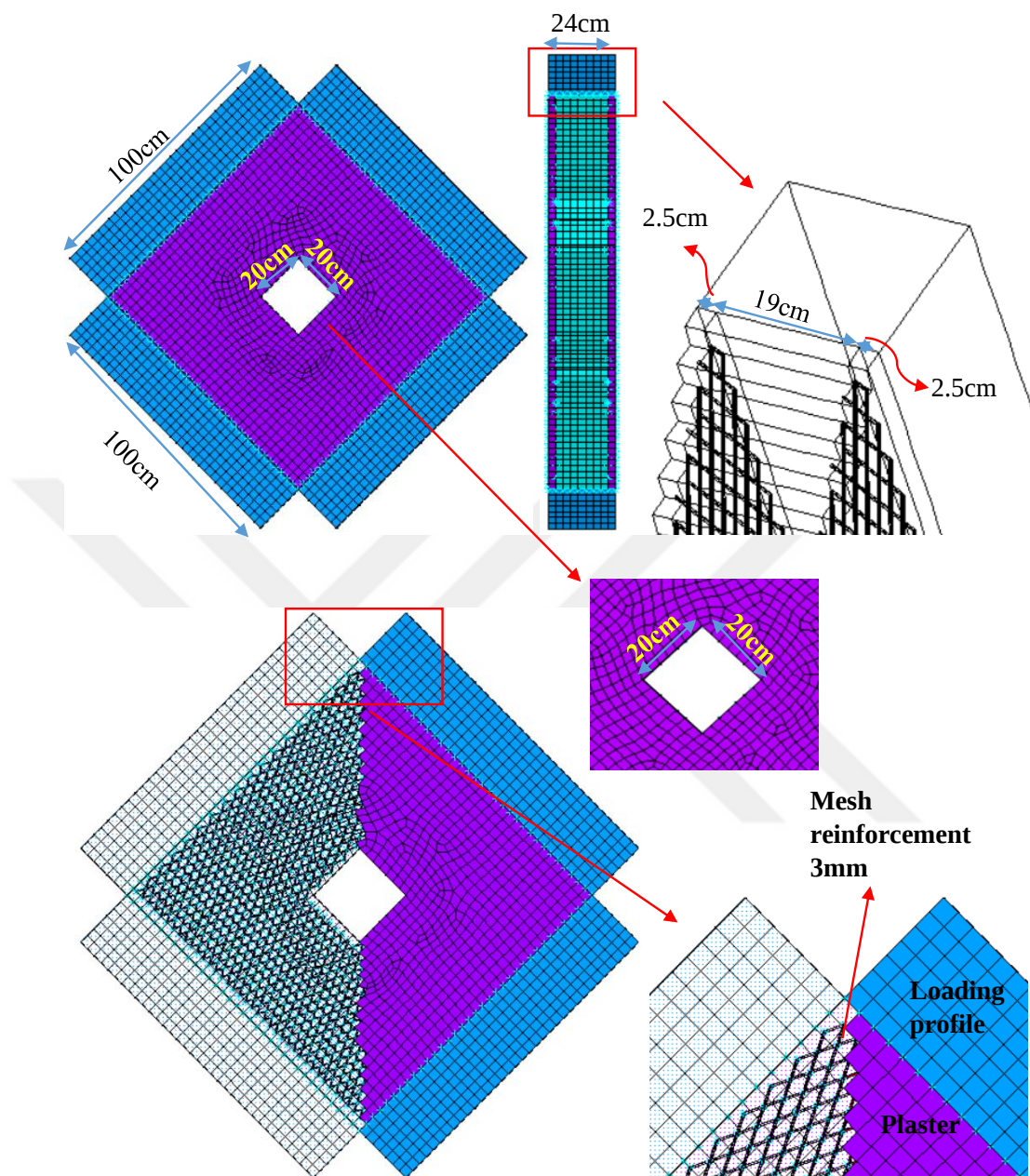
Figure 4.6. 20% opening ratio of the masonry wall model-3mm mesh reinforcement
