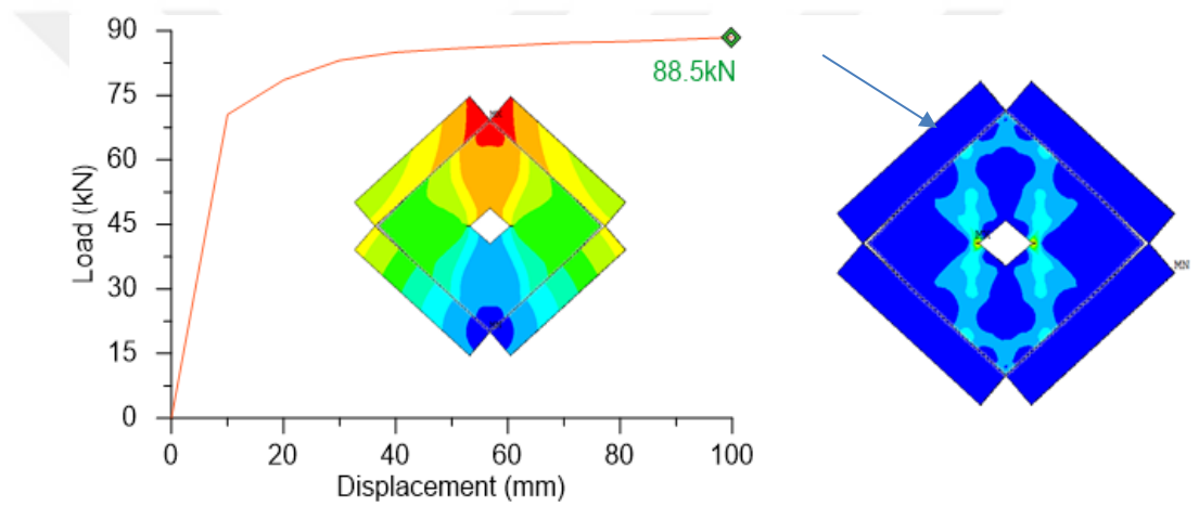
Figure 4.11. Load-Displacement curve, deformation shape, and total mechanical strain diagram of the wall with 20% opening (thickness of steel mesh 2.0mm)
