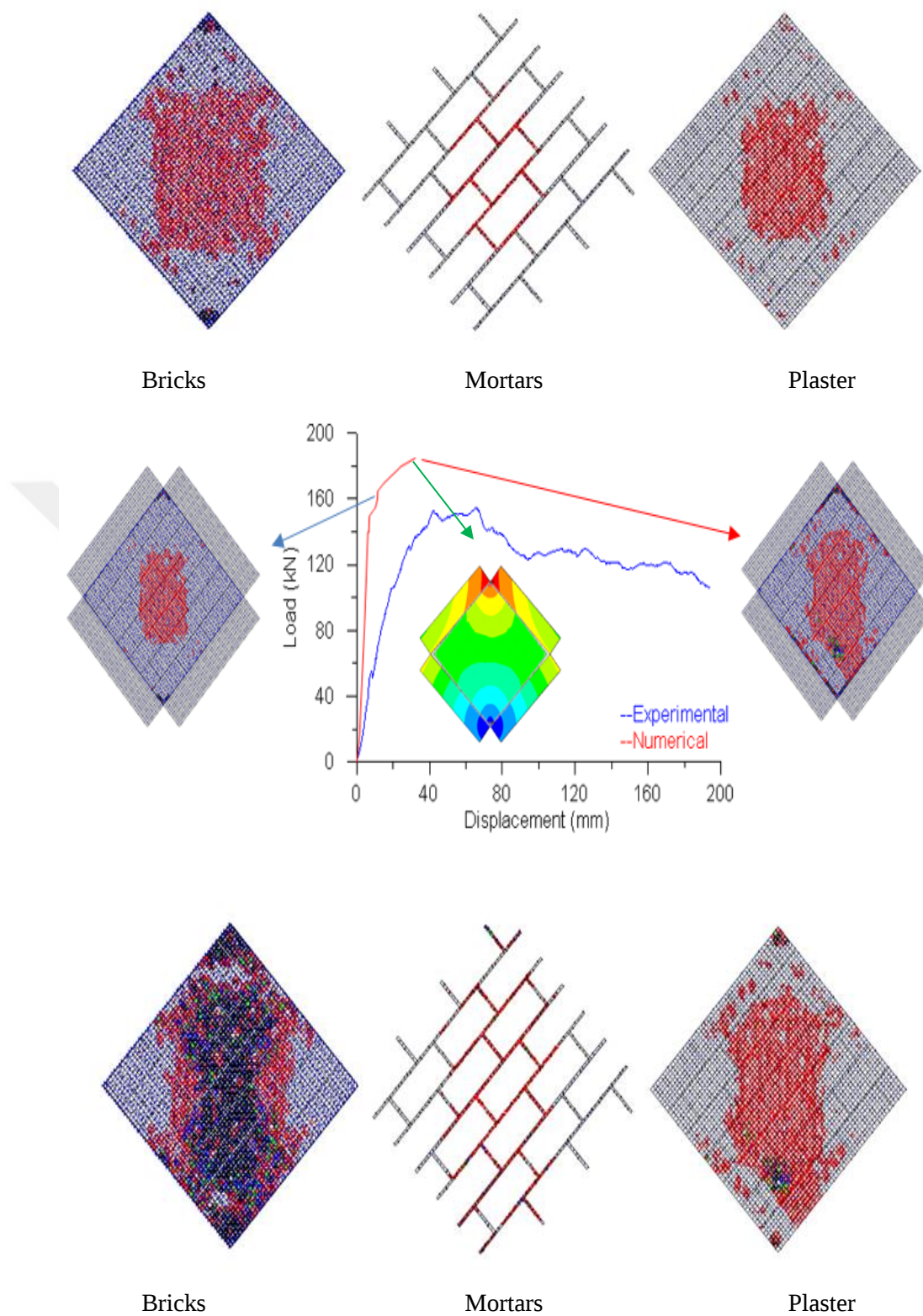
Figure 3.15. Load-displacement curve, deformation shape, and crack pattern of MBW 1.5-150 model
