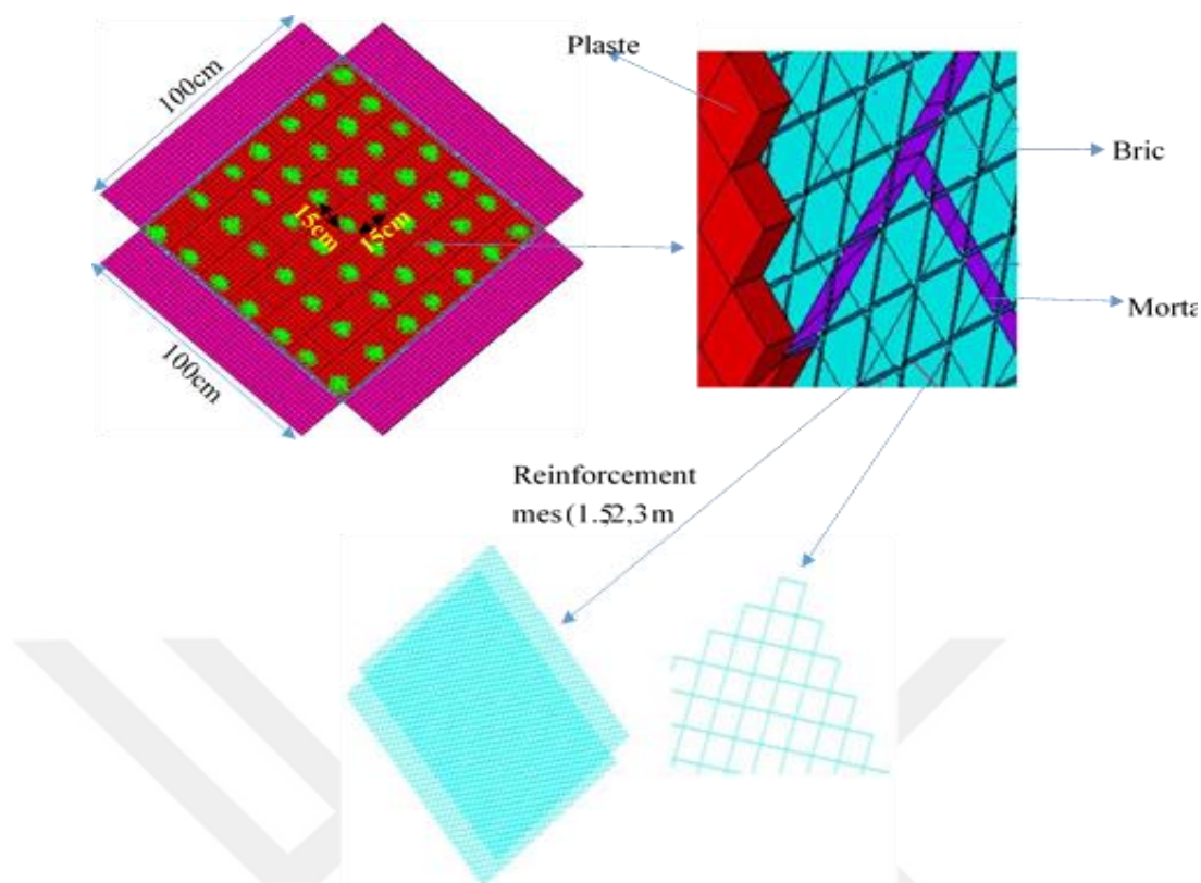
Figure 3.11. Dimensions of the MBW 1.5-150, 2.0-150, 3.0-150 the numerical model [3]
