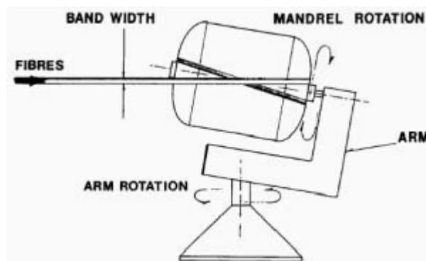
Fig 3.18 Polar winding
