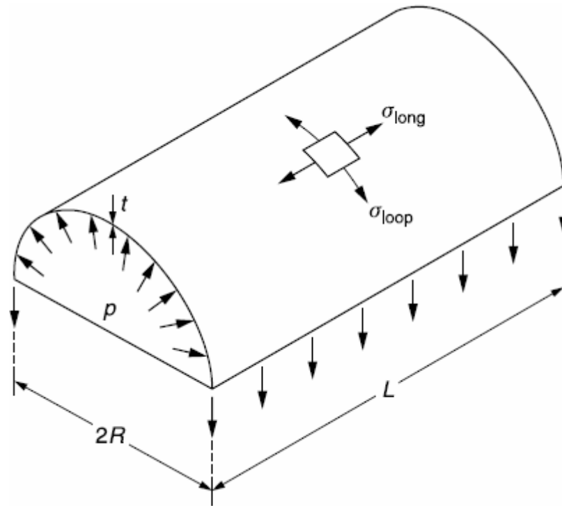
Figure 5.2 Thin cylindrical shell.
