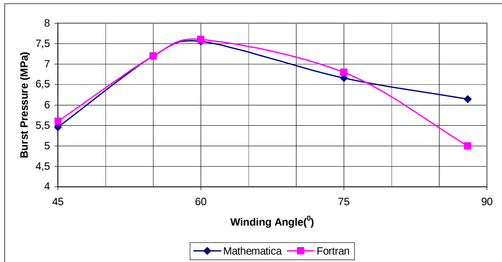
Figure 7.2 Numerical results of burst pressure with increasing winding angle for a laminates symmetrically.
