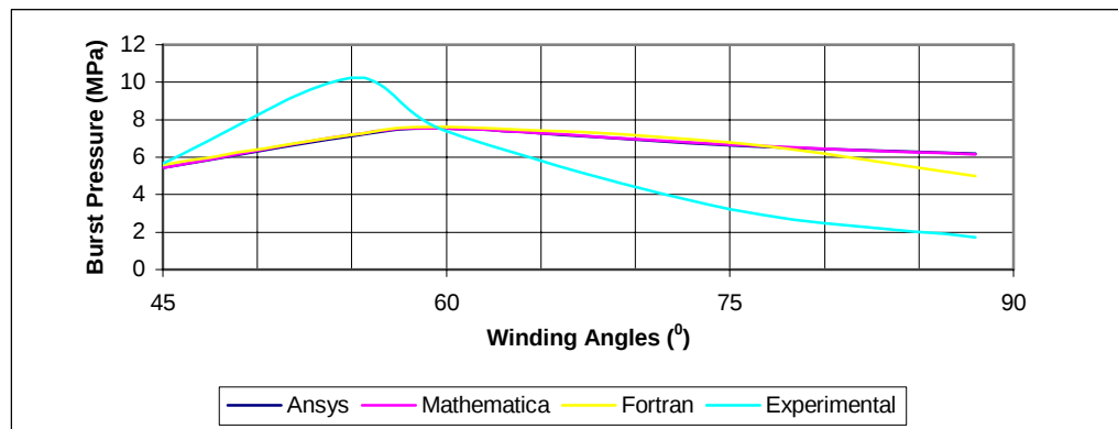
Figure 7.6 Comparing theoretical results, finite element results with experimental result symmetrically.
