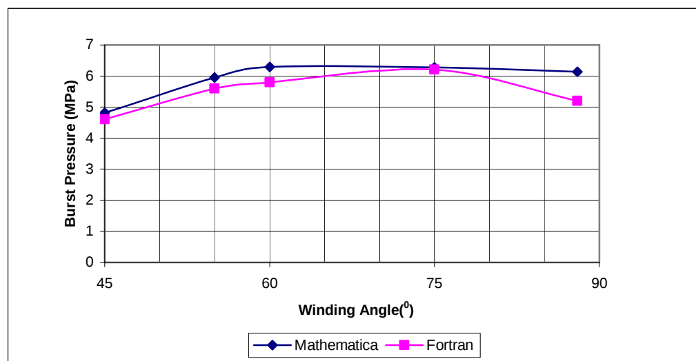
Figure 7.3 Numerical results of burst pressure with increasing winding angle for a laminates antisymmetrically.
