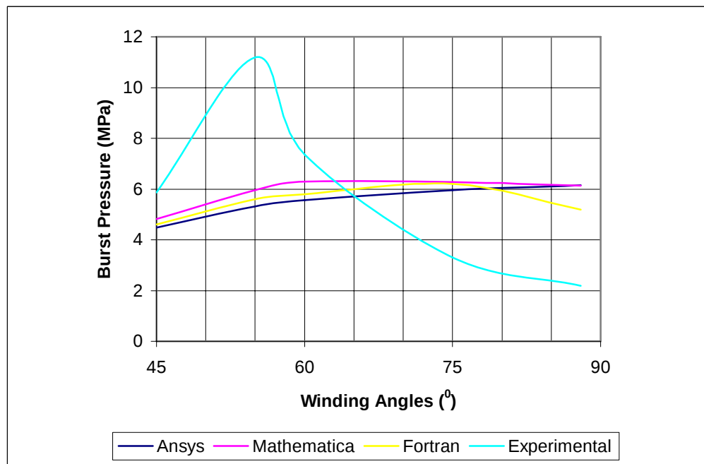
Figure 7.7 Comparing theoretical results, finite element results with experimental results antisymmetrically.
