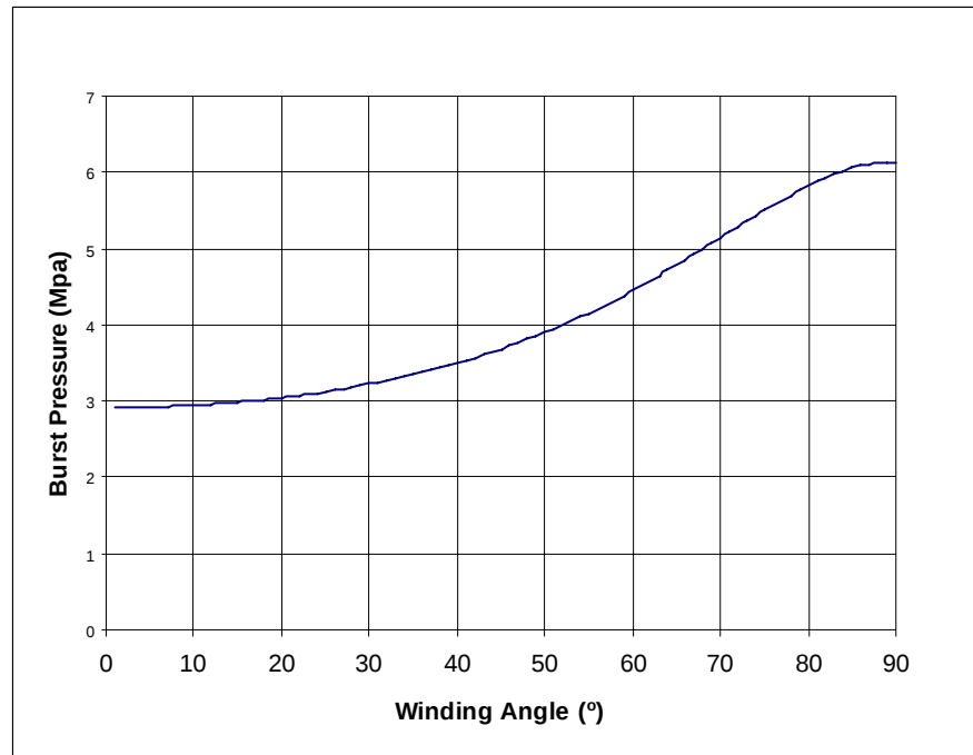
Figure 7.1 Variation of burst pressure with increasing winding angle for a lamina.
