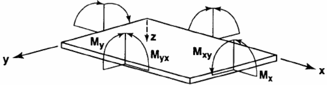
Figure 4.7 Moments on a flat laminate.
