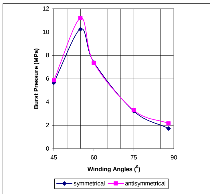
Figure 7.5 Experimental results of burst pressure with increasing winding angle for test specimens.
