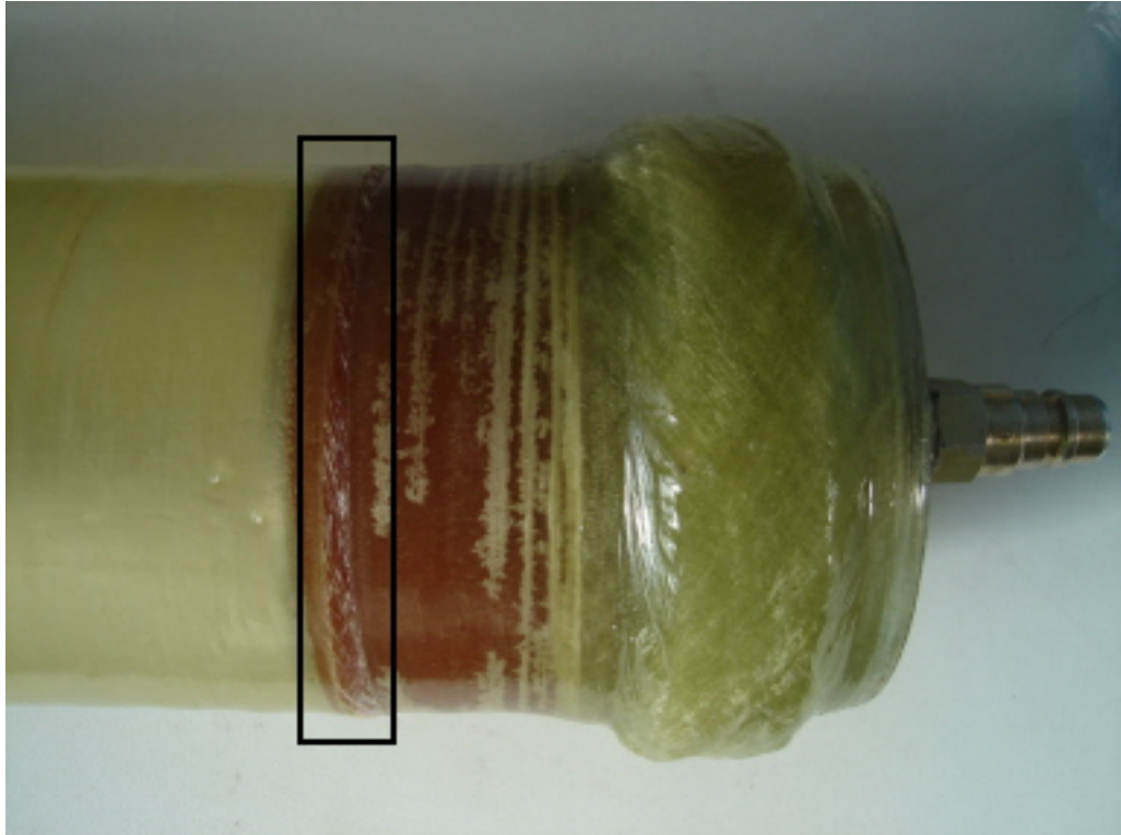
Figure 7.10 Fiber breakage damage mechanism.
