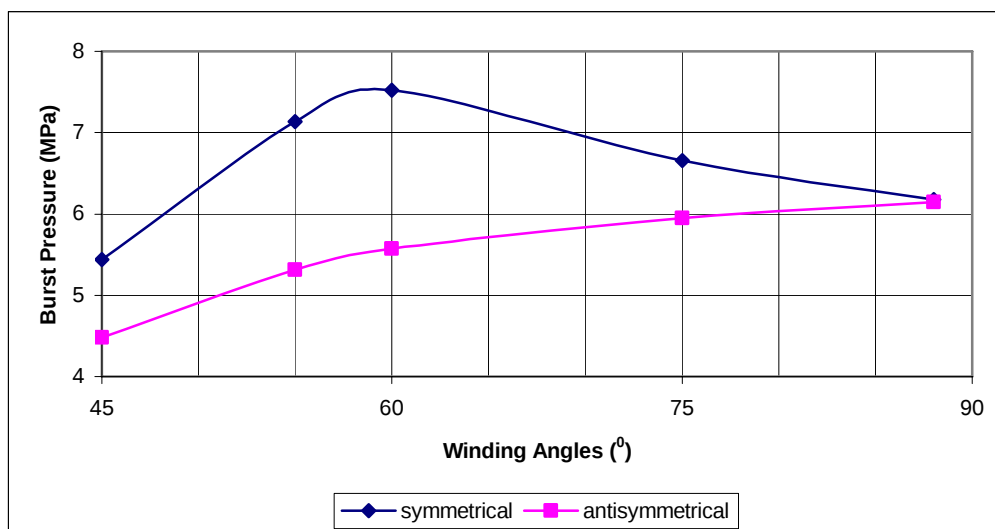
Figure 7.4 Ansys results of burst pressure with increasing winding angle for a laminates
