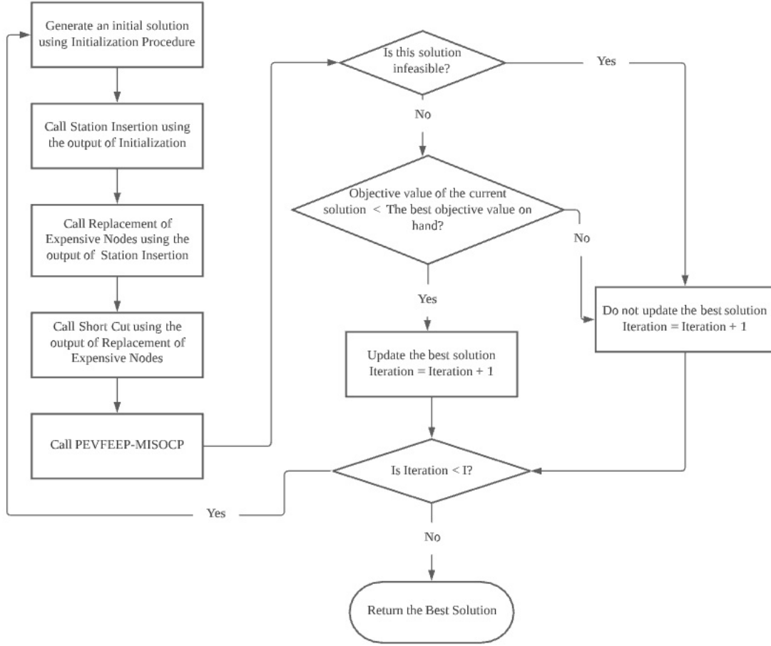
Figure 4.5: VNS Algorithm
