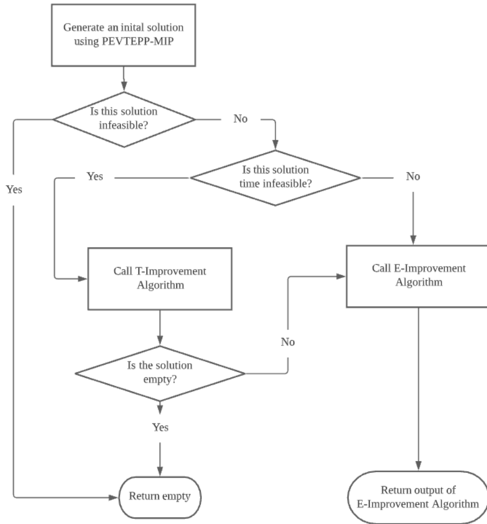
Figure 4.1: Matheuristic Algorithm with MIP Initialization
