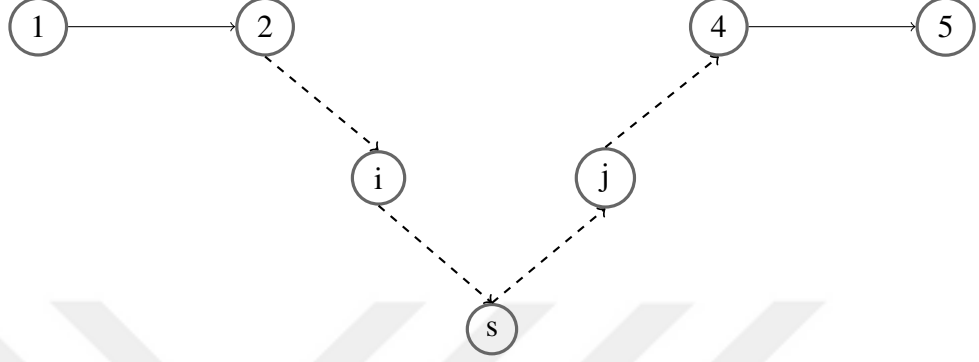
Connection of a Station Node s \in S to the Path using unvisited Nodes i and j \in N
