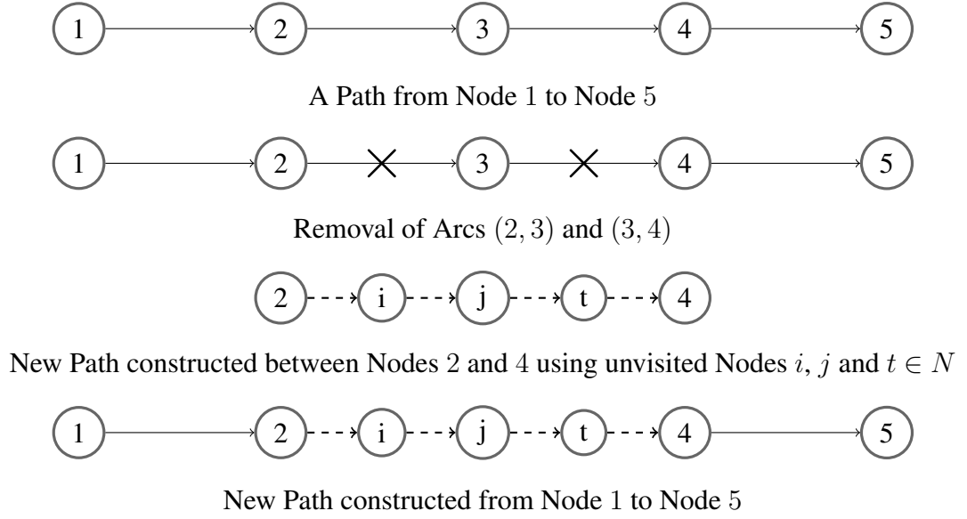
Figure 4.3: An Illustration of Replacement of Expensive Nodes Algorithm
