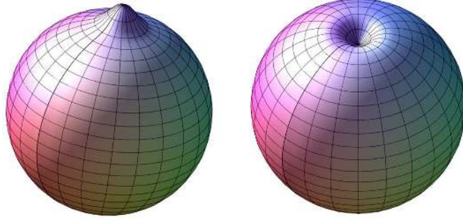
Figure B.1: A sphere with a bump on the left and a miss/reverse bump on the right. The exact value of the parameters in Eq. (B.11) are as follows: R = 1 , \alpha = 40 and \epsilon_0 = \pm 0.2 . The positive and negative \epsilon_0 results in the left and in the right figures, respectively.
