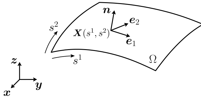
Figure C.1: Surface parametrization.
