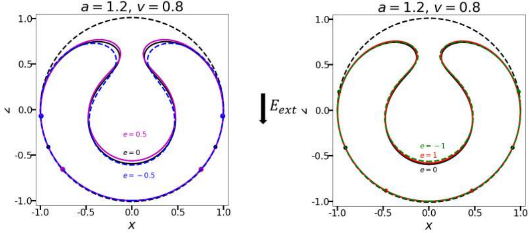
Figure 4.6: Response of flexoelectric fluid membrane with (a, v) = (1.2, 0.8) for small values of |e| . The black curve indicates the flexoelectric membrane in the absence of an electric field.
