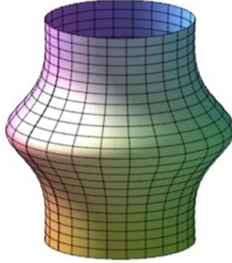
Figure B.4: A large cylinder with small deformation on the z = 0 ( xy - plane ) and \lambda = -0.3
